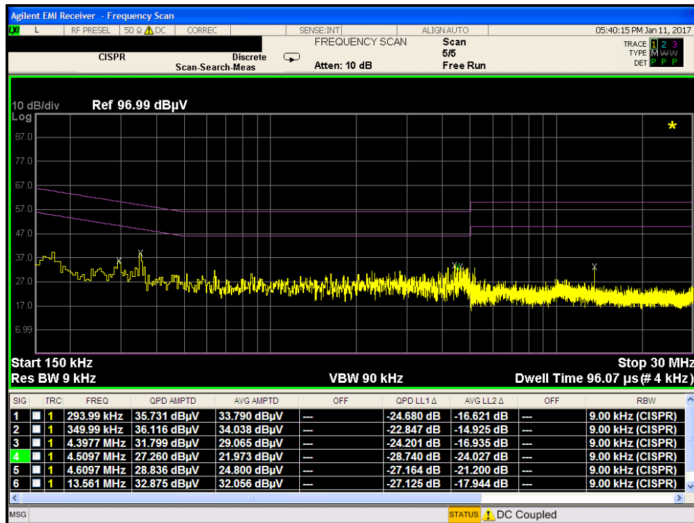
Plot 7-2. Line-Conducted Test Plot (N, Antenna Terminated in 50Ω)
