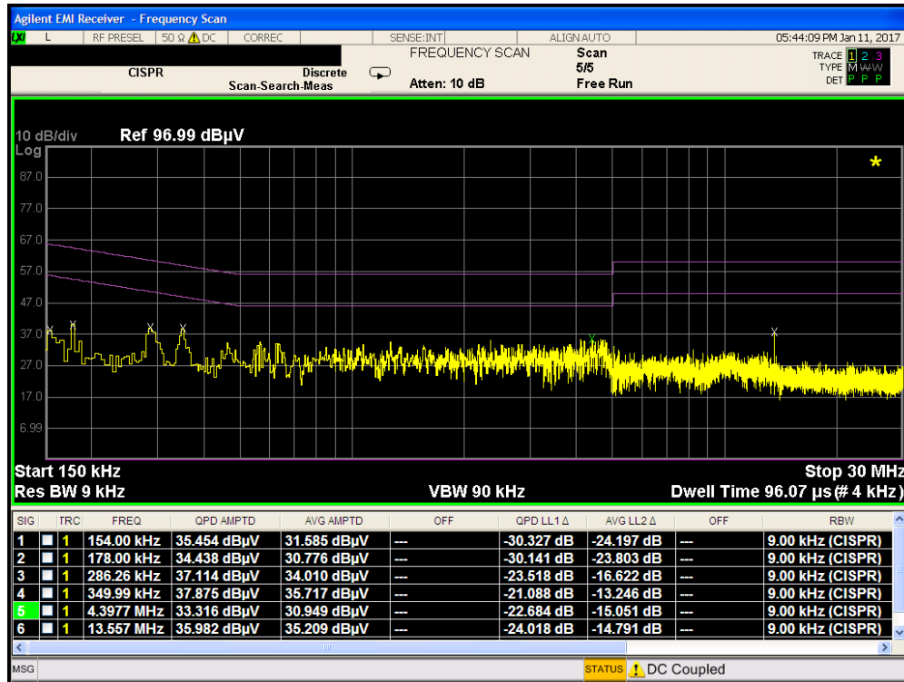
Plot 7-1. Line-Conducted Test Plot (L1, Antenna Terminated in 50Ω)
