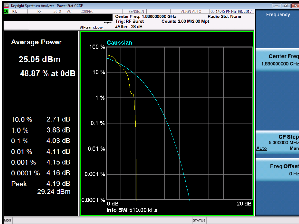
Plot 7-42. Peak-Average Ratio Plot (EDGE1900 Mode – Ch. 661)
