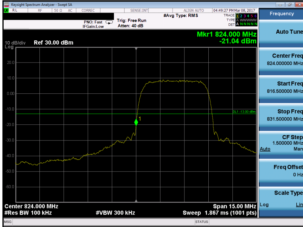
Plot 7-39. Band Edge Plot (Cellular WCDMA Mode – Ch. 4132)
