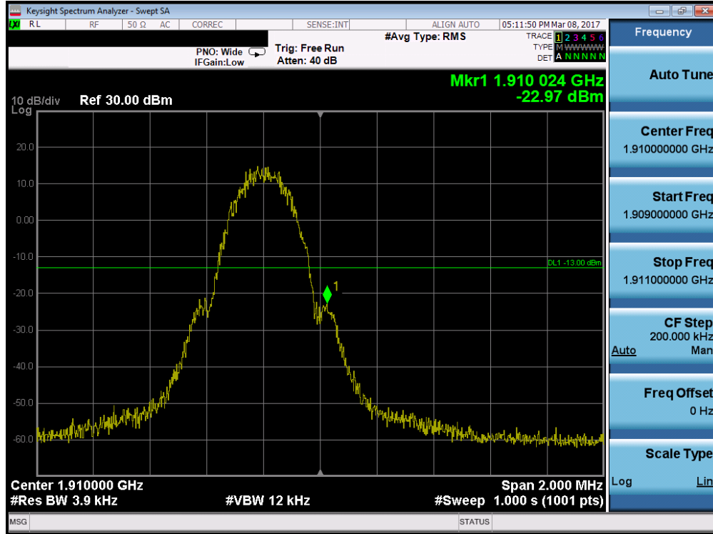
Plot 7-37. Band Edge Plot (PCS GSM Mode – Ch. 810)
