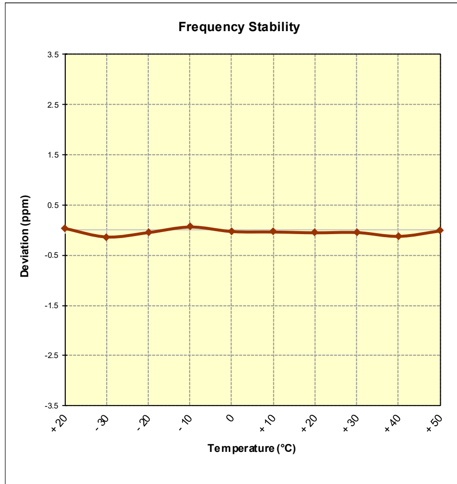
Figure 7-10. Frequency Stability Graph (PCS GSM Mode – Ch. 661)
