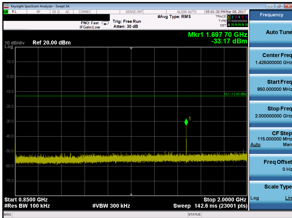
Plot 7-13. Conducted Spurious Plot (Cellular GSM Mode – Ch. 251)
