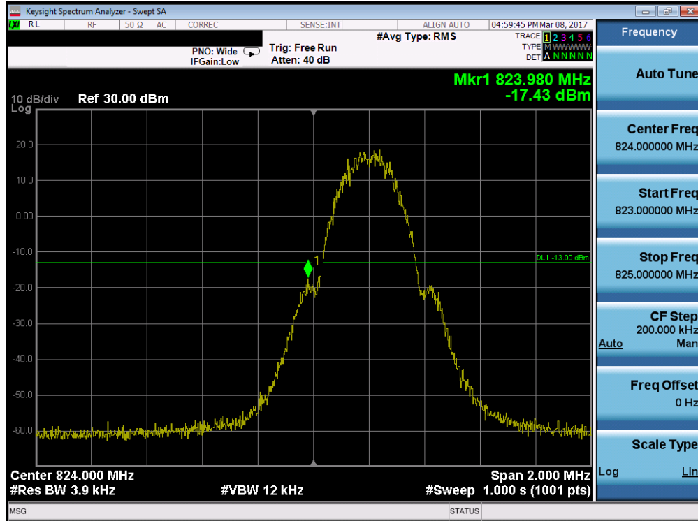
Plot 7-33. Band Edge Plot (Cellular GSM Mode – Ch. 128)
