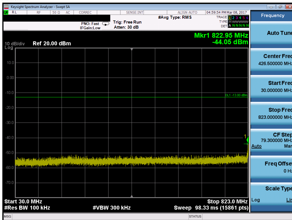
Plot 7-6. Conducted Spurious Plot (Cellular GSM Mode – Ch. 128)
