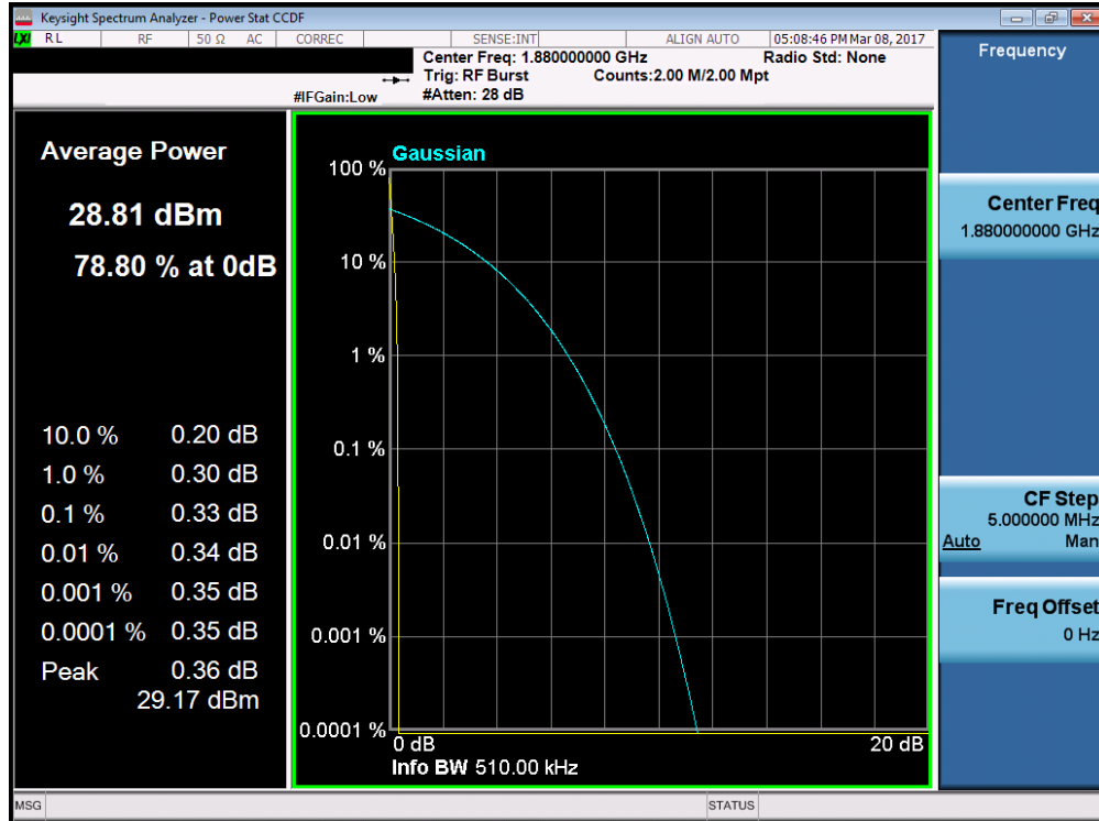
Plot 7-41. Peak-Average Ratio Plot (PCS GSM Mode – Ch. 661)
