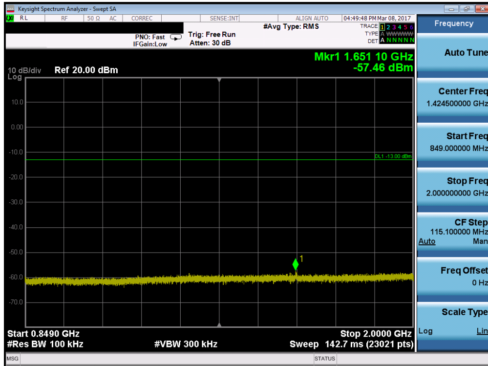
Plot 7-25. Conducted Spurious Plot (Cellular WCDMA Mode – Ch. 4132)
