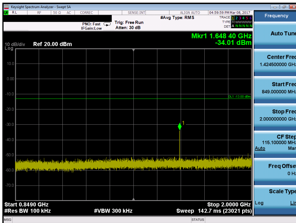
Plot 7-7. Conducted Spurious Plot (Cellular GSM Mode – Ch. 128)
