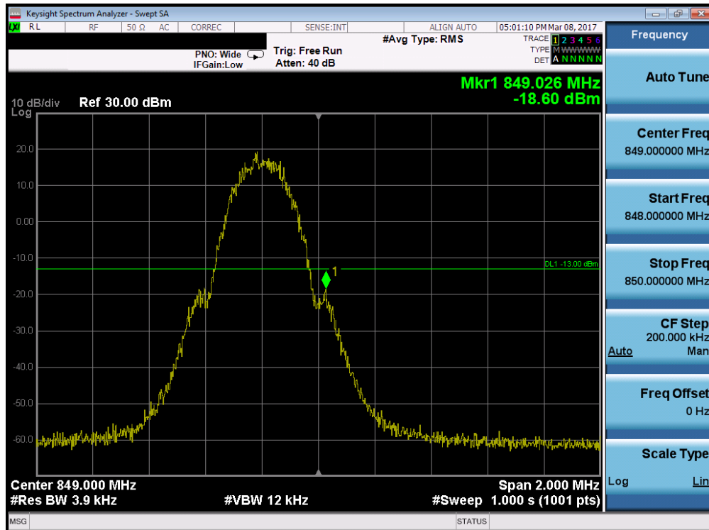
Plot 7-34. Band Edge Plot (Cellular GSM Mode – Ch. 251)
