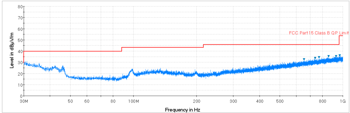
Plot 7-280. Radiated Spurious Plot below 1GHz (802.11a – U3 Ch. 157, Ant. Pol. H)
