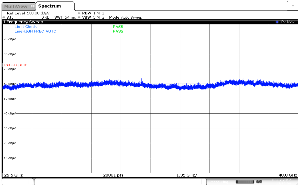
Plot 7-192. Radiated Spurious Plot 26.5-40GHz (2.4GHz – 5GHz, Ant. Pol. V)
