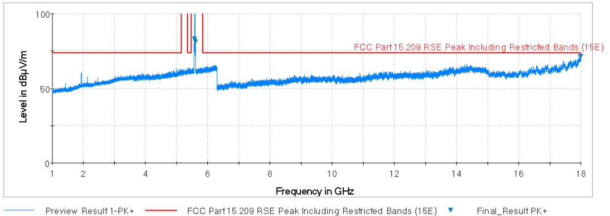
Plot 7-162. Radiated Spurious Plot above 1GHz (802.11a – U2C Ch. 116, Ant. Pol. V)
