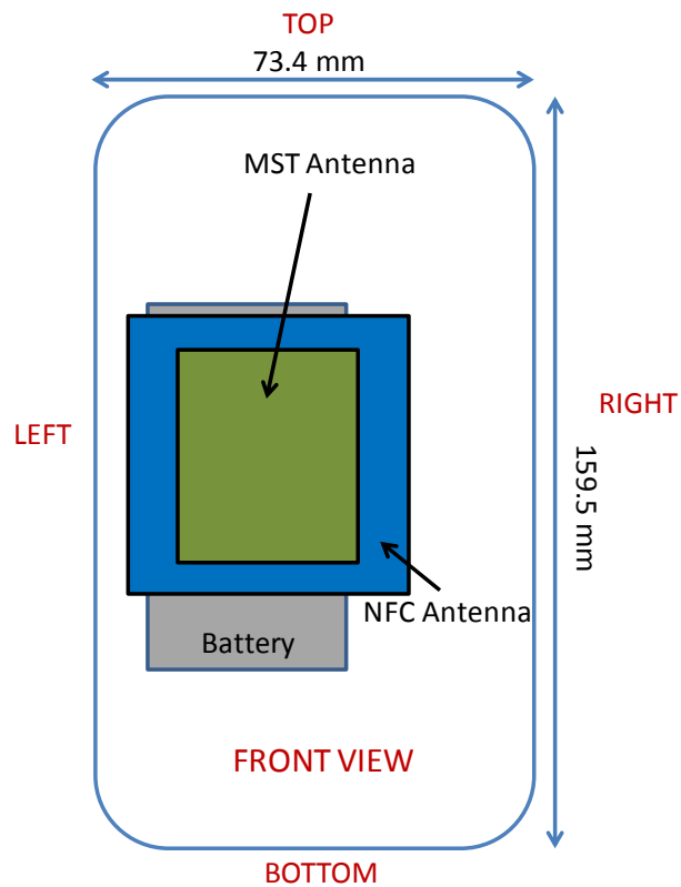
Figure F-2 MST and NFC Antenna Locations
