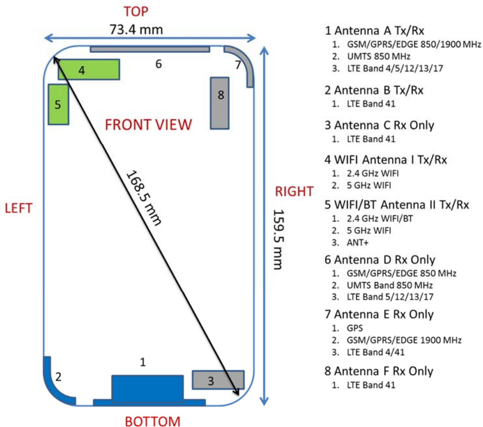
Figure F-1 DUT Antenna Locations
