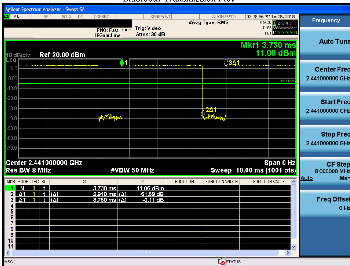
Bluetooth Transmission Plot
