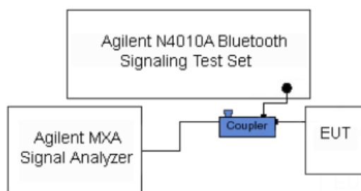
Power Measurement Setup
