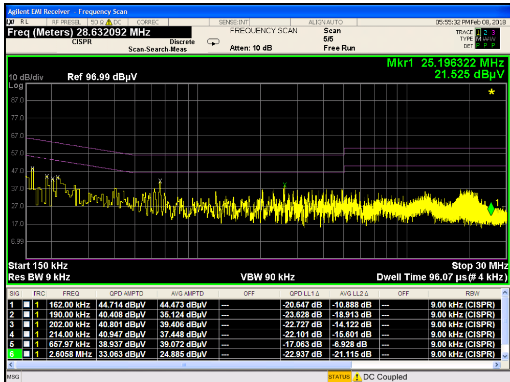
Plot 7-11. Line-Conducted Test Plot (N) with WCC
