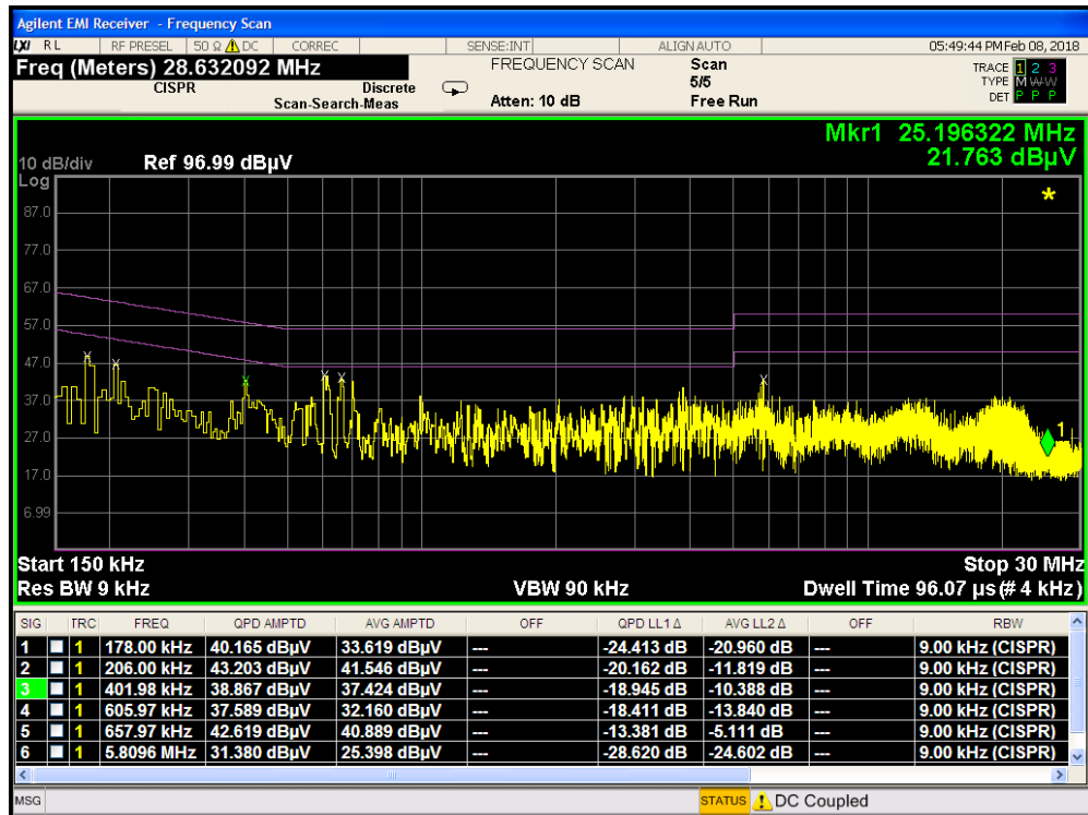
Plot 7-10. Line-Conducted Test Plot (L1) with WCC
