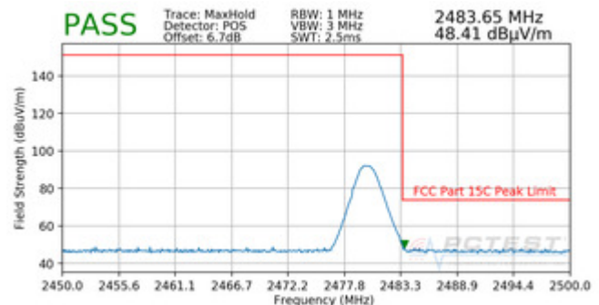
Plot 7-7. Radiated Restricted Upper Band Edge Measurement with WCP (Peak)
