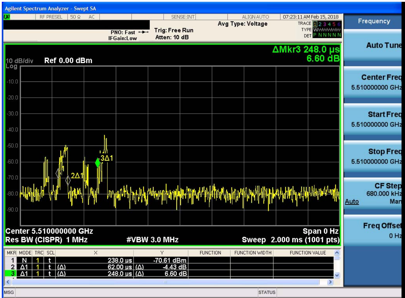
Figure 5-2. Band 2C Pulse Width & Period
