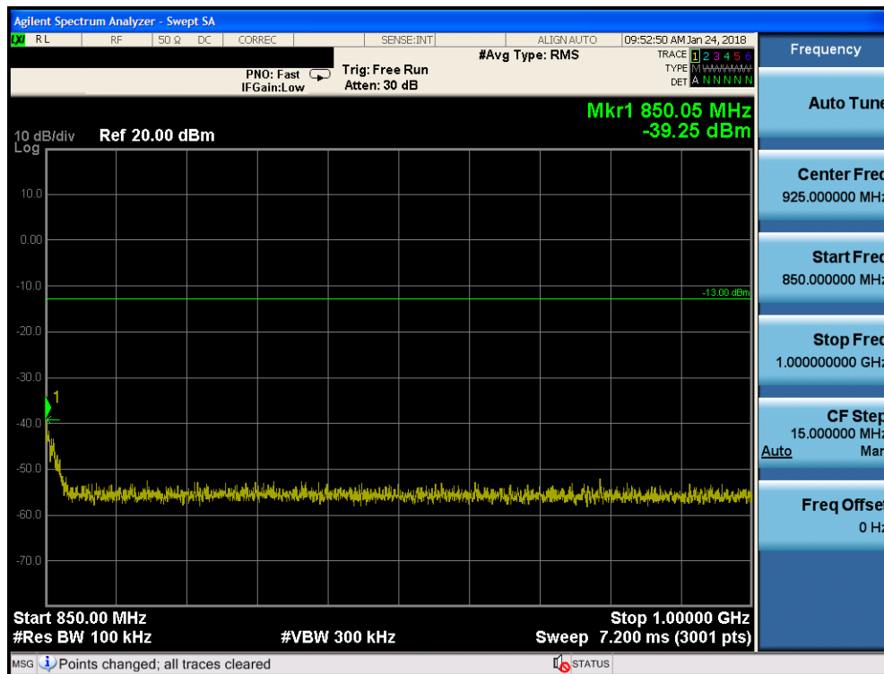
Plot 7-13. Conducted Spurious Plot (Cellular GPRS Mode - High Channel)
