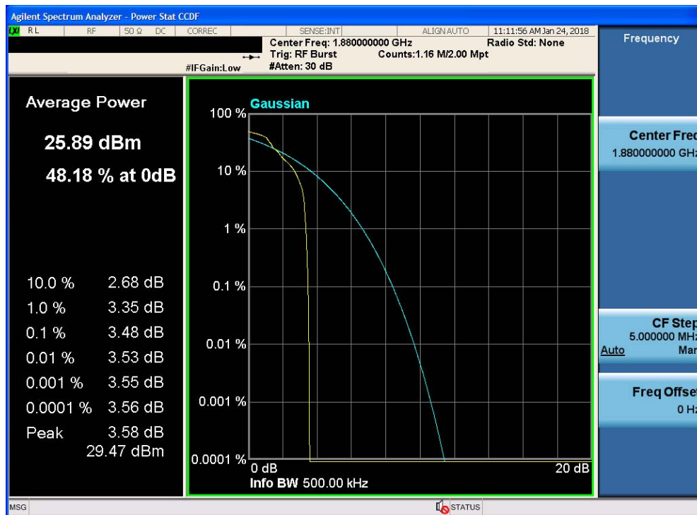
Plot 7-44. Peak-Average Ratio Plot (PCS EDGE Mode)
