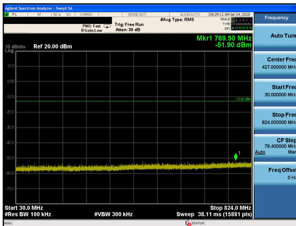
Plot 7-9. Conducted Spurious Plot (Cellular GPRS Mode - Mid Channel)
