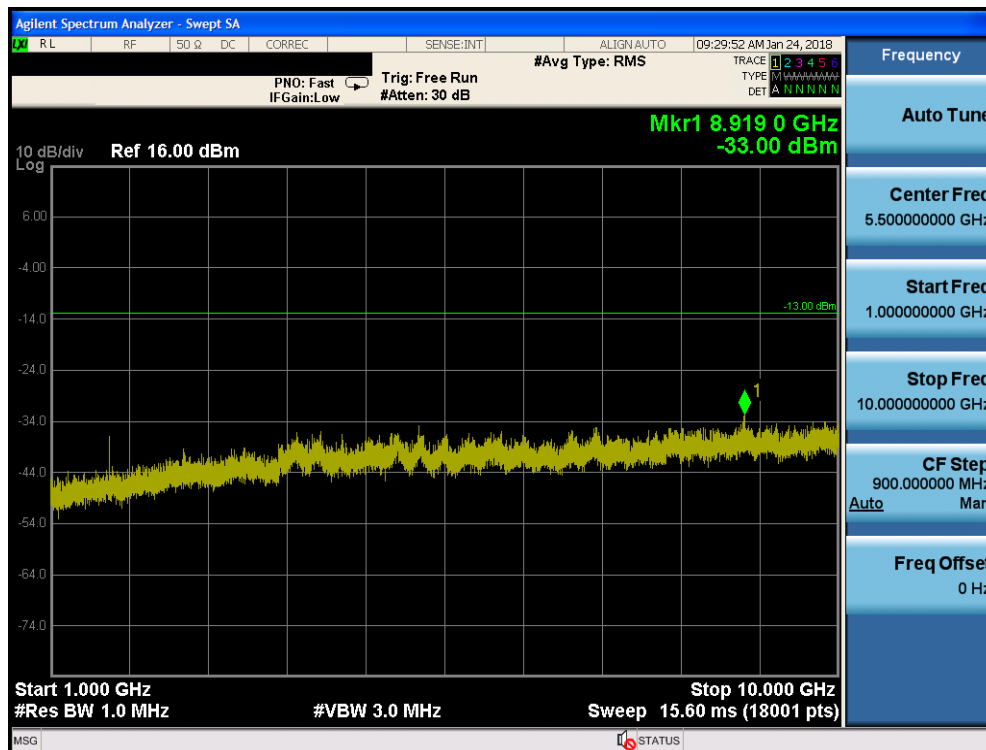
Plot 7-11. Conducted Spurious Plot (Cellular GPRS Mode - Mid Channel)
