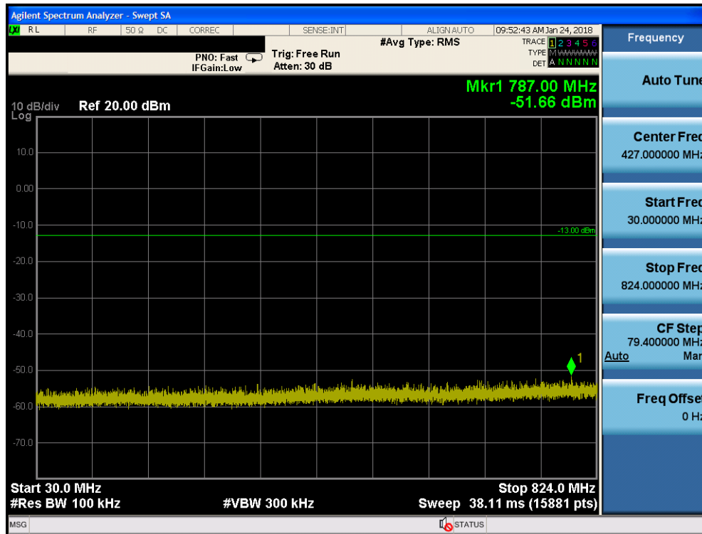
Plot 7-12. Conducted Spurious Plot (Cellular GPRS Mode - High Channel)
