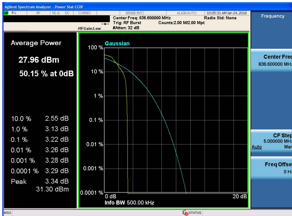
Plot 7-42. Peak-Average Ratio Plot (Cellular EDGE Mode)
