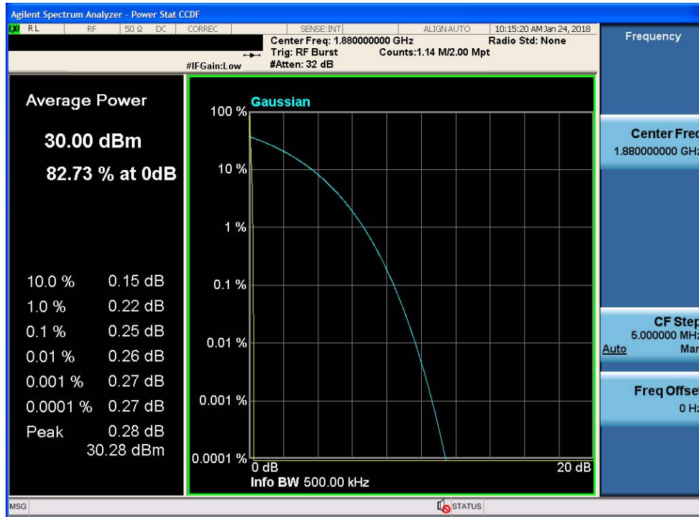
Plot 7-43. Peak-Average Ratio Plot (PCS GPRS Mode)
