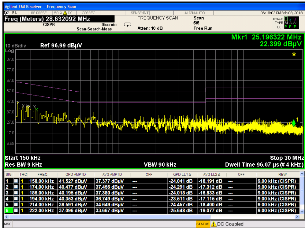
Plot 7-57. Line-Conducted Test Plot (L1) with WCP
