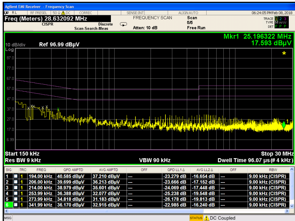
Plot 7-58. Line-Conducted Test Plot (N) with WCP
