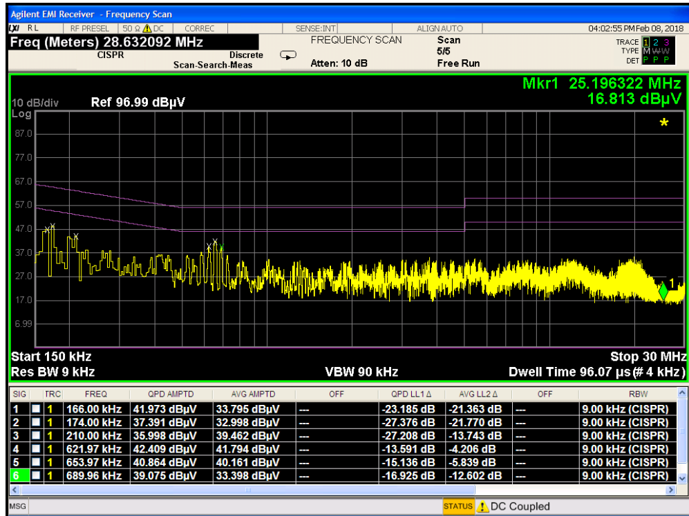
Plot 7-55. Line-Conducted Test Plot (L1)
