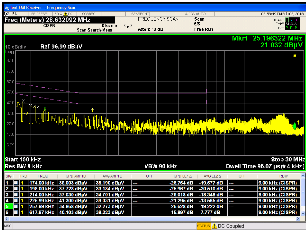
Plot 7-56. Line-Conducted Test Plot (N)
