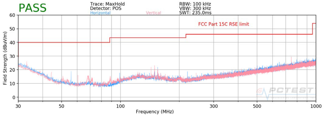
Plot 7-54. Radiated Spurious Plot below 1GHz
