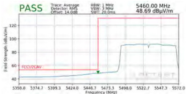
Plot 7-227. Radiated Lower Band Edge Plot (Average – UNII Band 2C)
