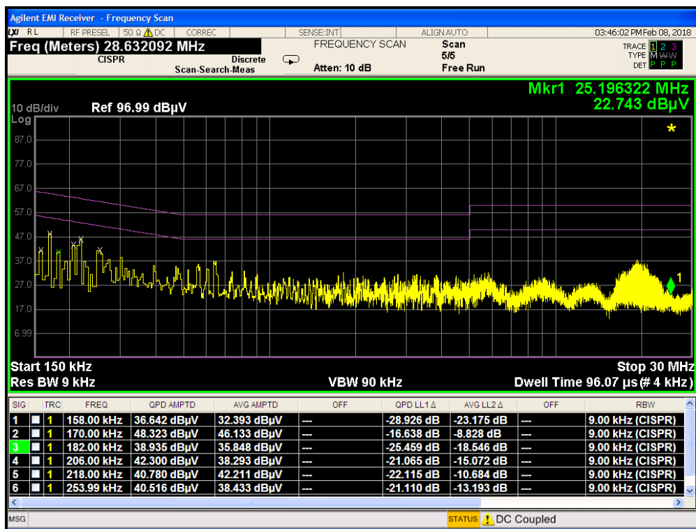
Plot 7-270. Line Conducted Plot with 802.11a UNII Band 2C (N)
