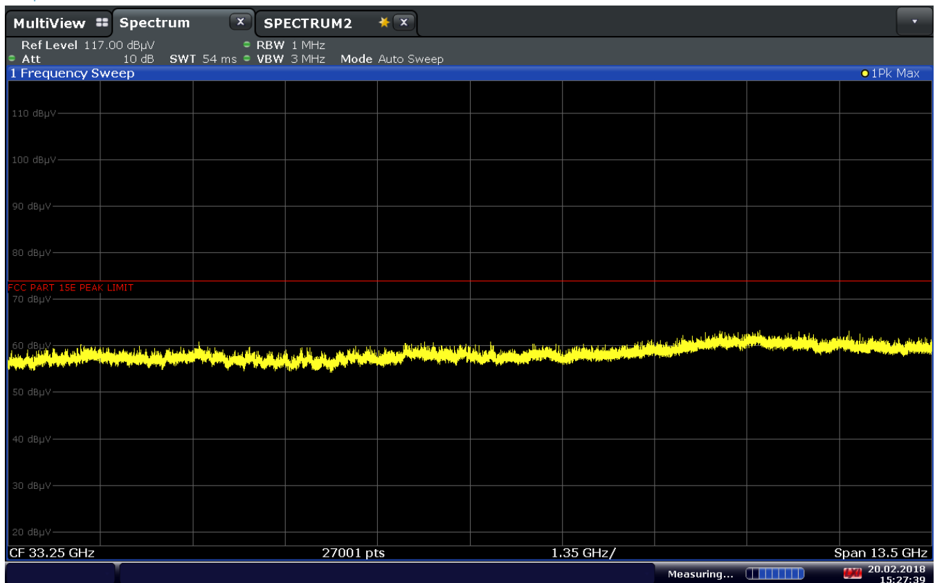
Plot 7-171. Radiated Spurious Plot above 26.5GHz (2.4GHz – 5GHz) H
