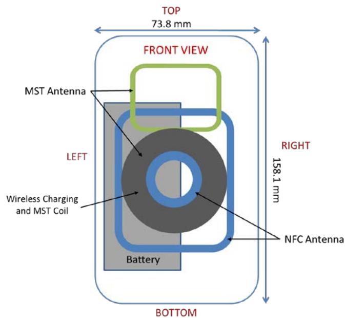
Figure F-2 NFC Antenna Locations
