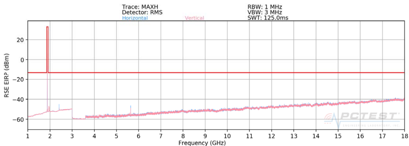
Plot 7-48. Radiated Spurious Emission Plot >1GHz (PCS GPRS Mode)
