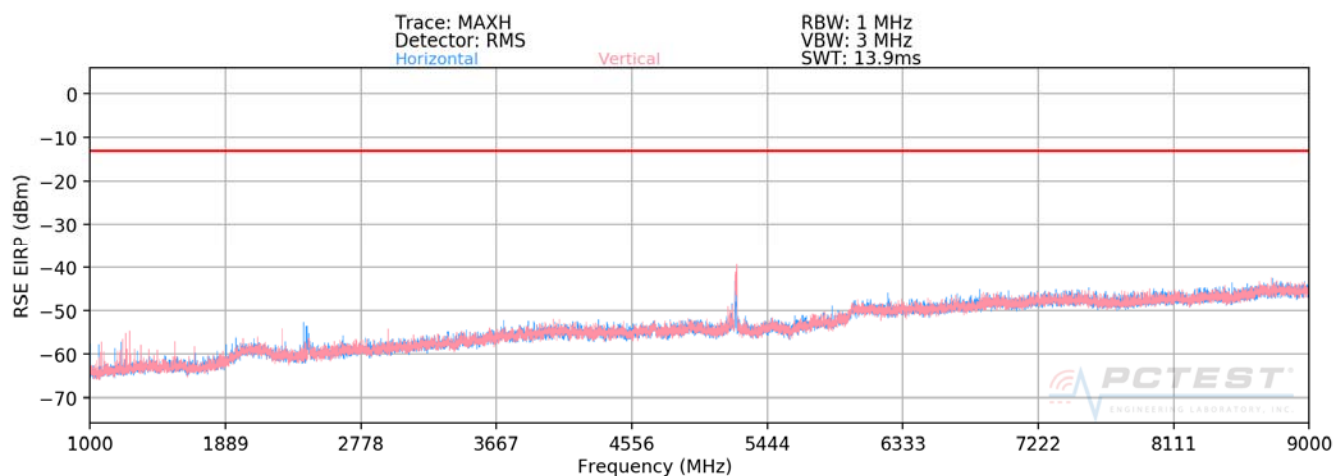
Plot 7-47. Radiated Spurious Emission Plot >1GHz (Cellular WCDMA Mode)
