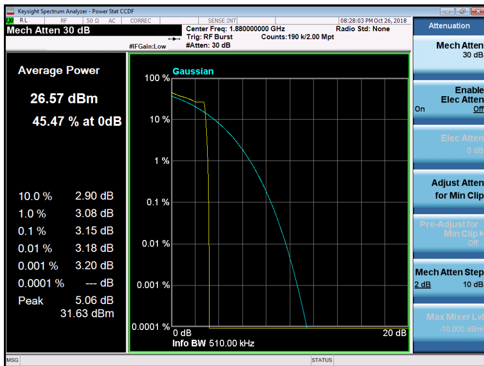
Plot 7-44. Peak-Average Ratio Plot (PCS EDGE1900 Mode)
