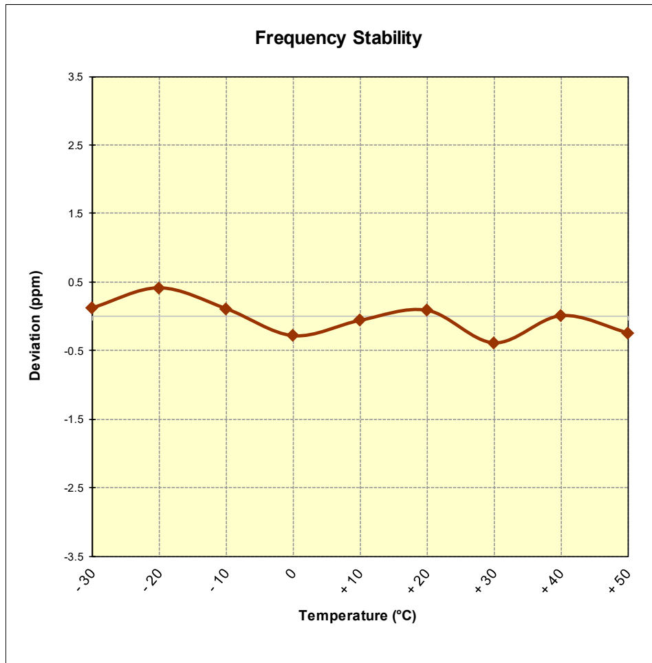
Figure 7-9. Frequency Stability Graph (Cellular WCDMA Mode – Ch. 4183)
