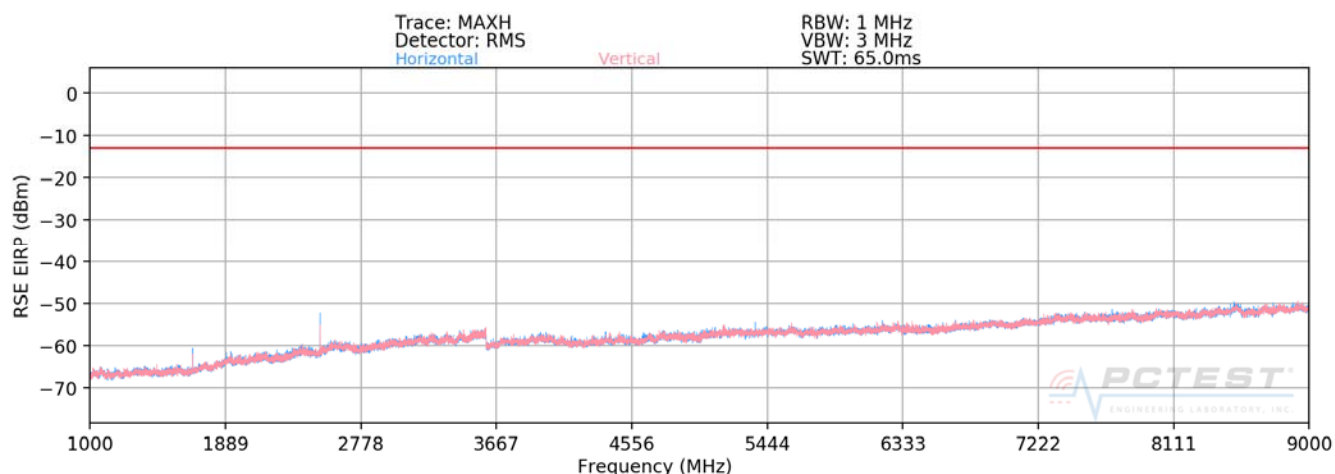
Plot 7-46. Radiated Spurious Emission Plot >1GHz (Cellular GPRS Mode)
