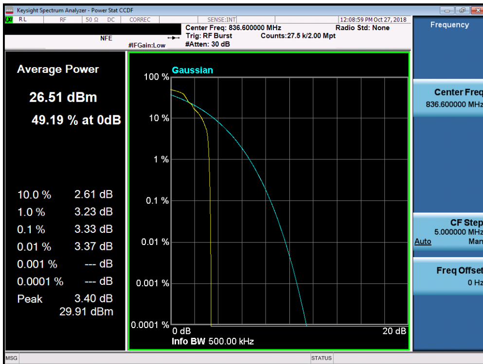
Plot 7-42. Peak-Average Ratio Plot (Cellular EDGE850 Mode)
