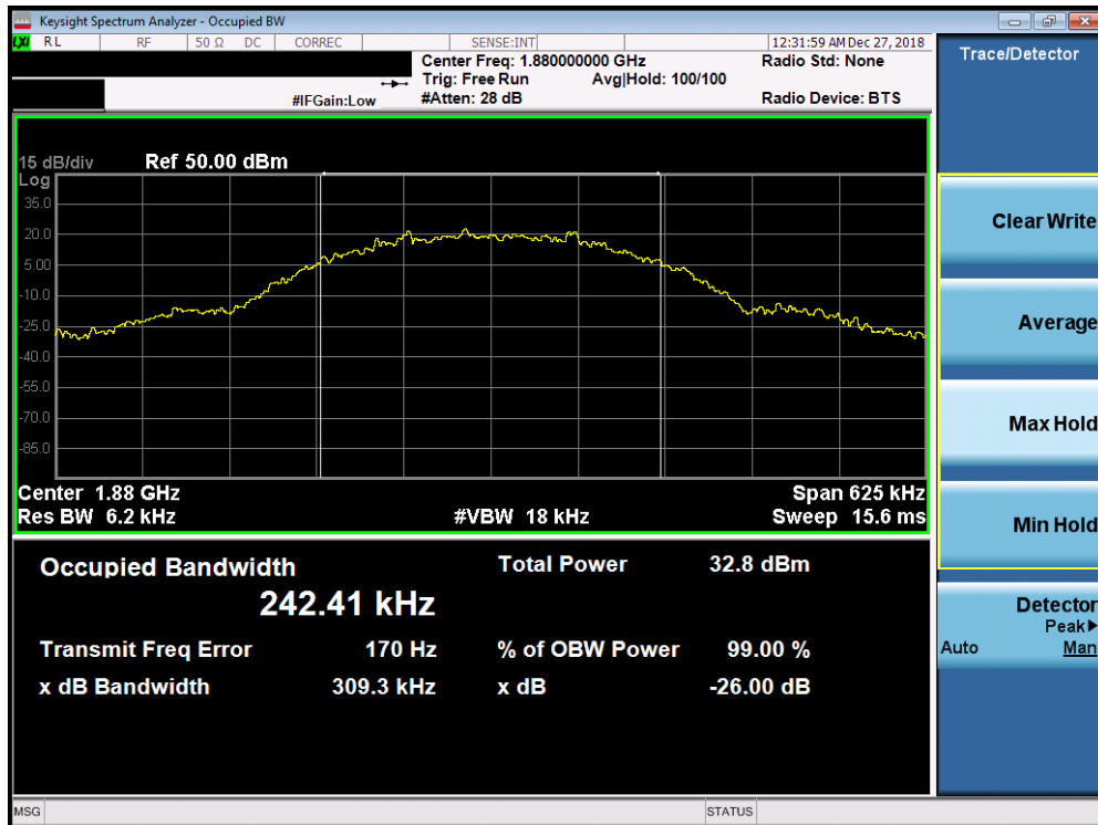
Plot 7-4. Occupied Bandwidth Plot (PCS EDGE1900 Mode)
