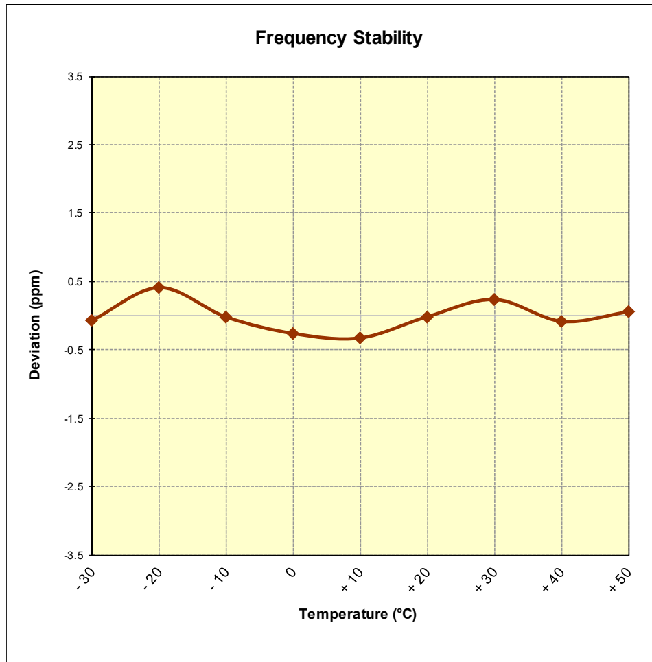
Figure 7-8. Frequency Stability Graph (Cellular GPRS Mode – Ch. 190)
