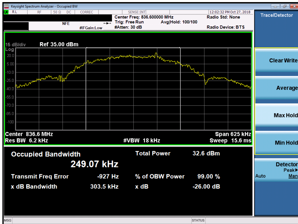
Plot 7-2. Occupied Bandwidth Plot (Cellular EDGE850 Mode)
