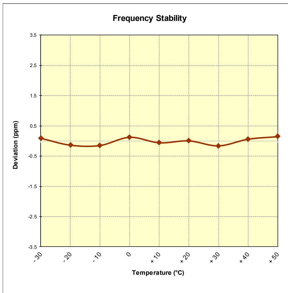
Figure 7-10. Frequency Stability Graph (PCS GPRS Mode – Ch. 661)
