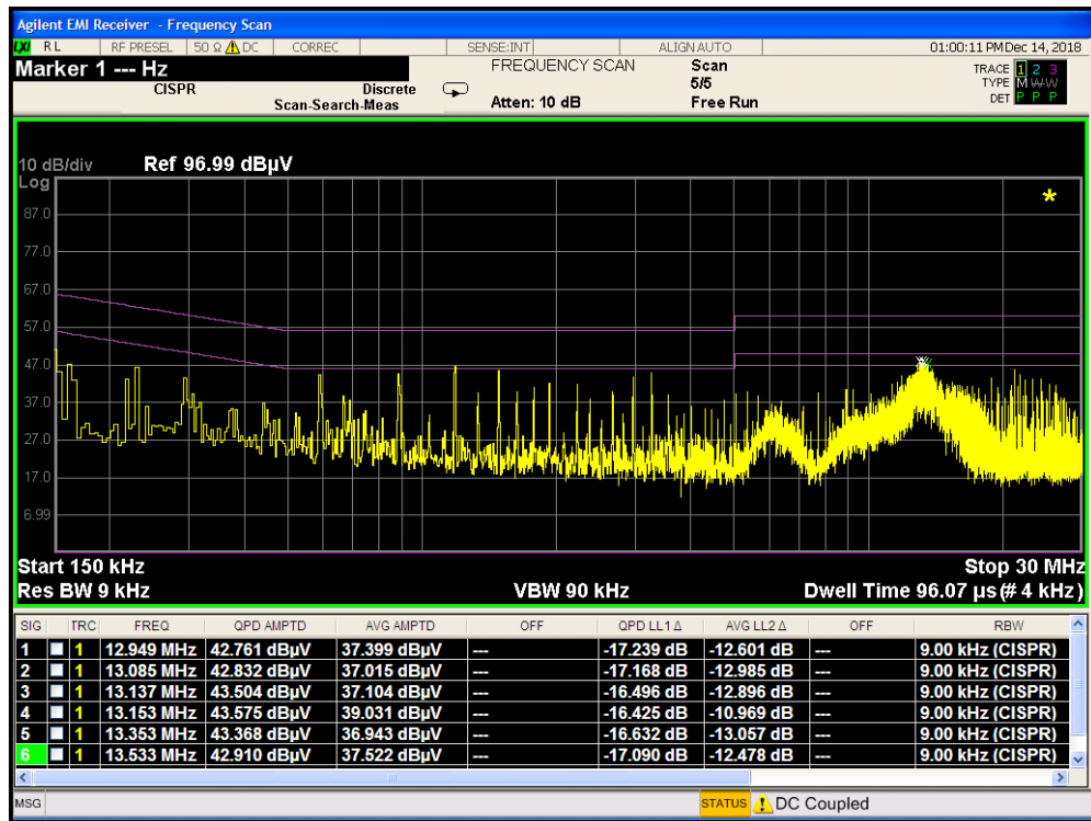
Plot 7-51. Line-Conducted Test Plot (L1) with Wireless Charging Pad
