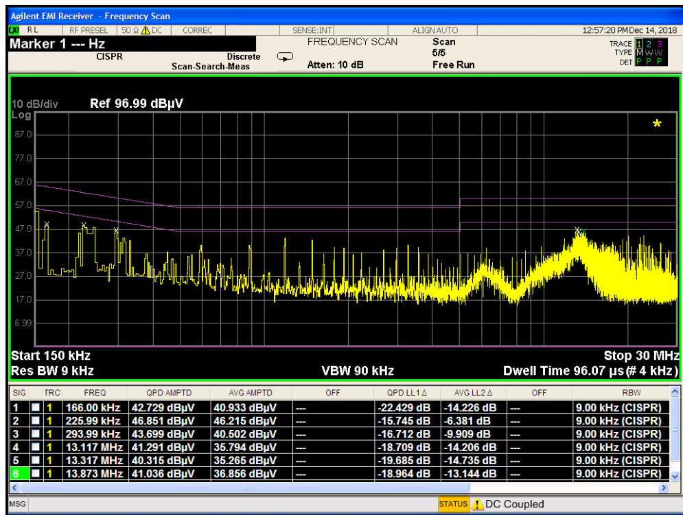
Plot 7-52. Line-Conducted Test Plot (N) with Wireless Charging Pad
