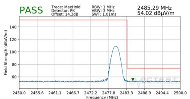
Plot 7-47. Radiated Restricted Upper Band Edge Measurement with WCP (Peak)
