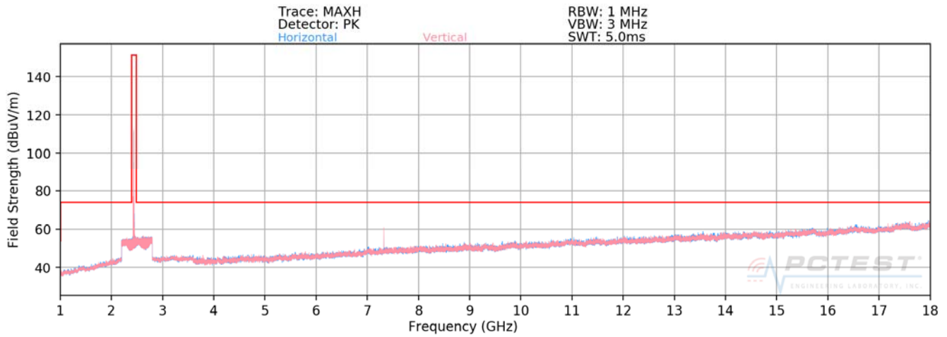
Plot 7-42. Radiated Spurious Plot above 1GHz (BT- Ch. 39)
