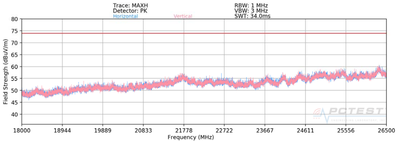
Plot 7-43. Radiated Spurious Plot above 18GHz
