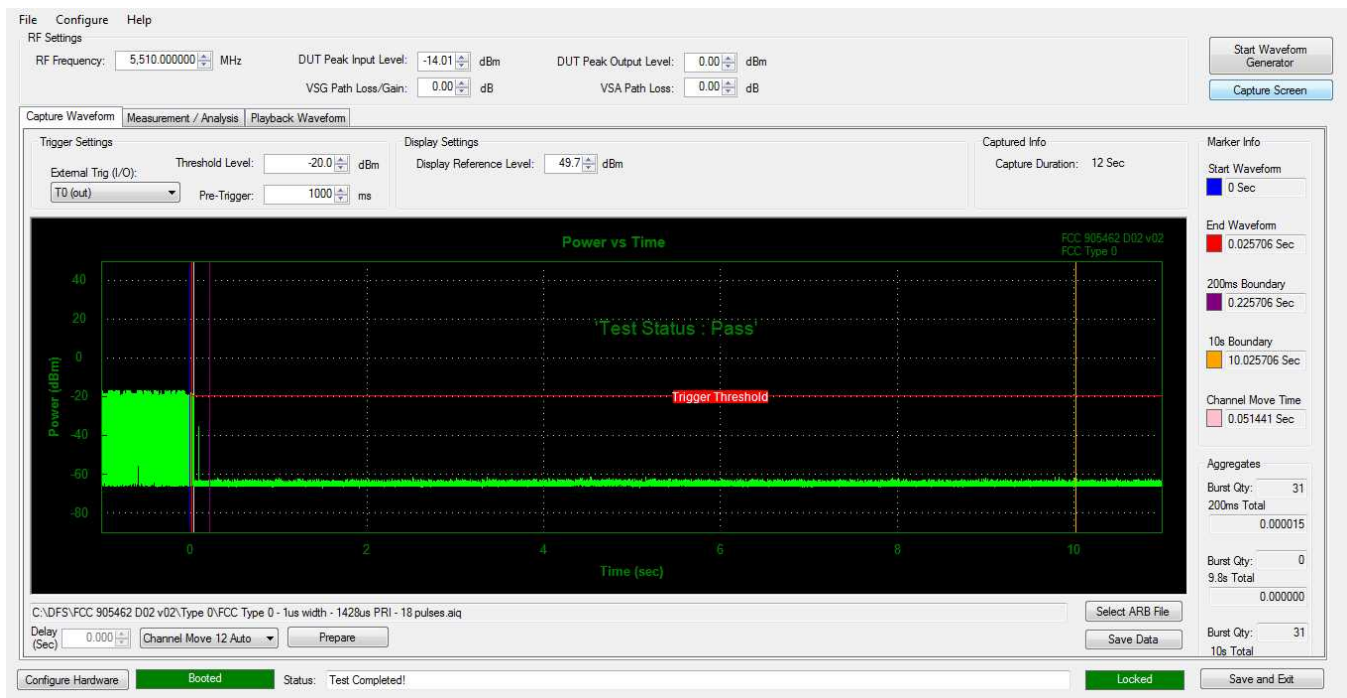
Figure 5-4. Band 2C Move Time and Aggregate Time
