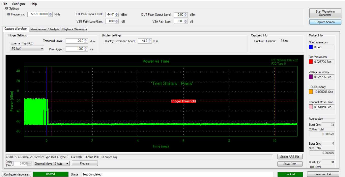
Figure 5-3. Band 2A Move Time and Aggregate Time
