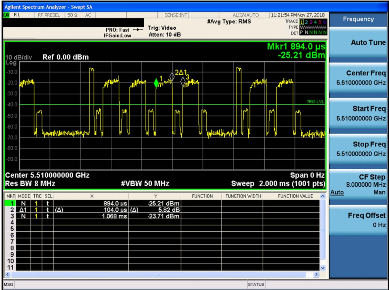
Figure 5-2. Band 2C Pulse Width and Period
