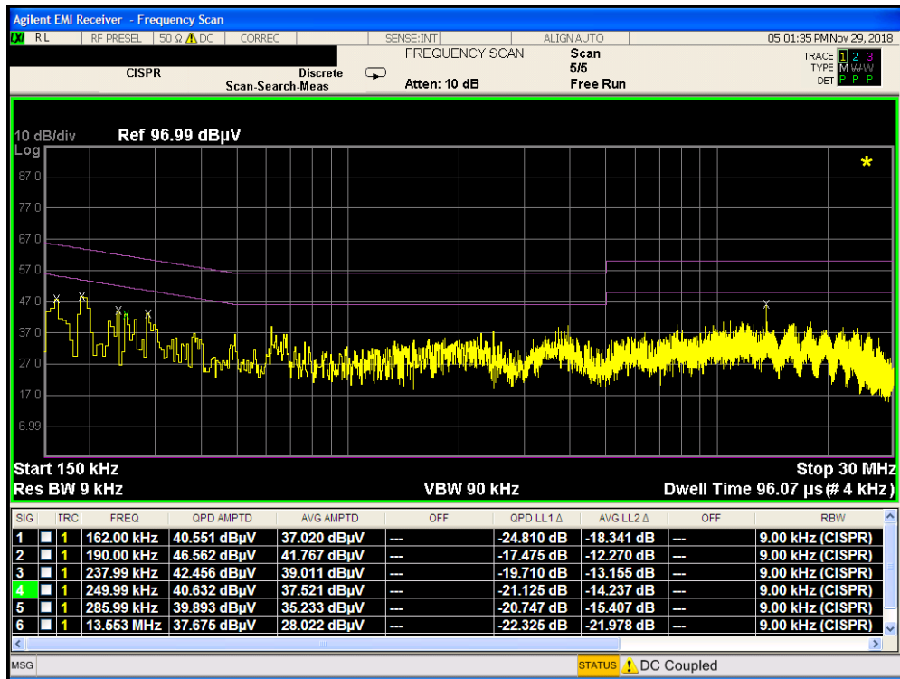
Plot 7-143. Line Conducted Plot with 802.11b (L1)
