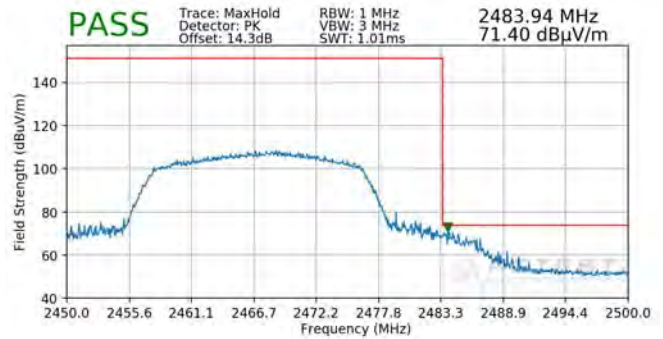
Plot 7-116. Radiated Restricted Upper Band Edge Measurement SISO ANT2 (Peak)
