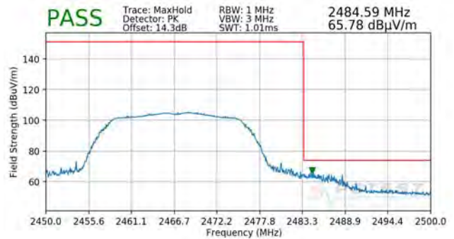
Plot 7-106. Radiated Restricted Upper Band Edge Measurement SISO ANT1 (Peak)
