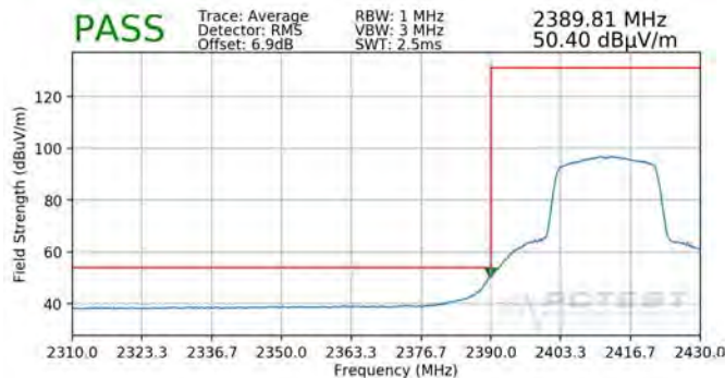
Plot 7-111. Radiated Restricted Lower Band Edge Measurement SISO ANT2 (Average)
