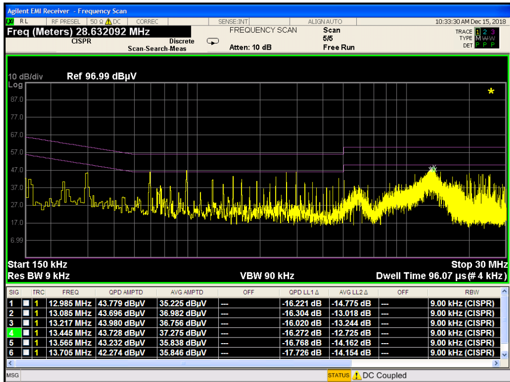
Plot 7-145. Line Conducted Plot with 802.11b (L1) with Wireless Charging Pad
