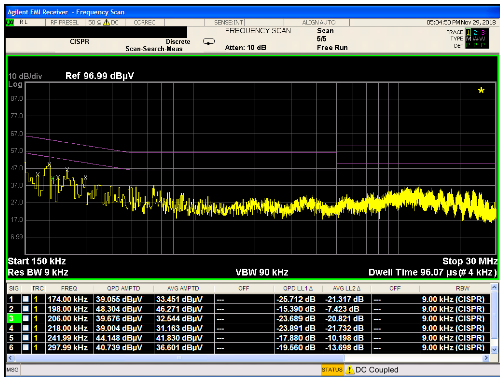
Plot 7-144. Line Conducted Plot with 802.11b (N)
