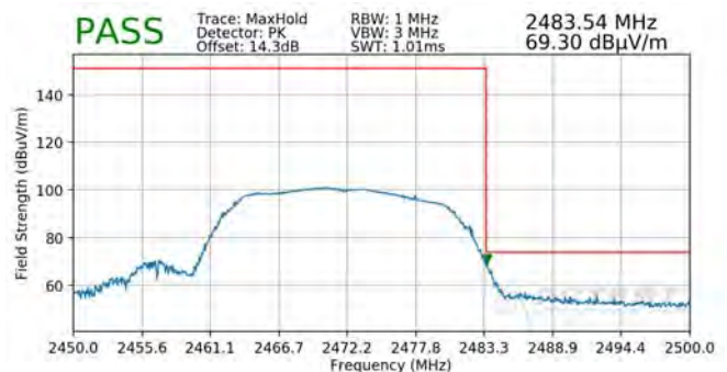
Plot 7-108. Radiated Restricted Upper Band Edge Measurement SISO ANT1 (Peak)
