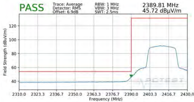
Plot 7-119. Radiated Restricted Band Edge Measurement SISO ANT2 with WCP (Average)
