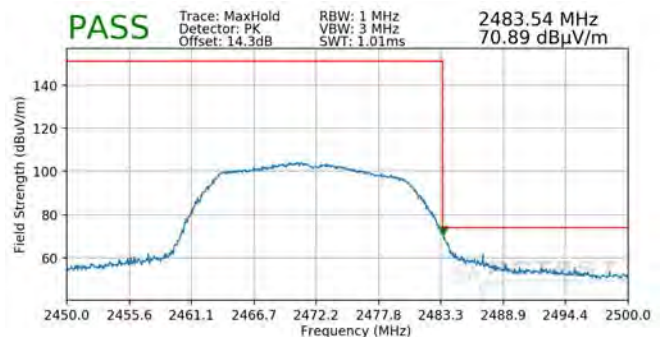
Plot 7-128. Radiated Restricted Upper Band Edge Measurement MIMO (Peak)
