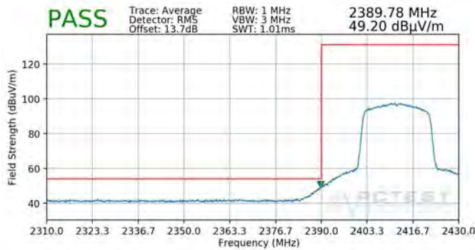
Plot 7-129. Radiated Restricted Band Edge Measurement MIMO with WCP (Average)
