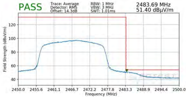
Plot 7-125. Radiated Restricted Upper Band Edge Measurement MIMO (Average)
