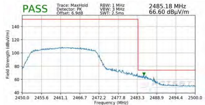
Plot 7-124. Radiated Restricted Upper Band Edge Measurement MIMO (Peak)
