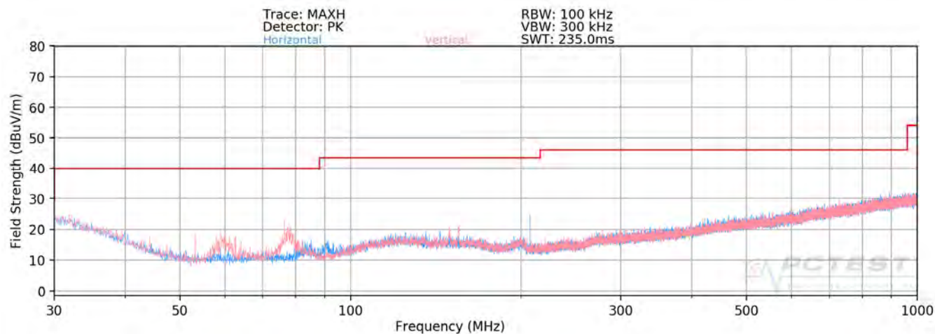
Plot 7-141. Radiated Spurious Plot below 1GHz SISO ANT1
