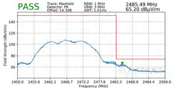
Plot 7-136. Radiated Restricted Upper Band Edge Measurement CDD (Peak)
