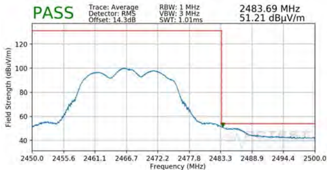
Plot 7-135. Radiated Restricted Upper Band Edge Measurement CDD (Average)
