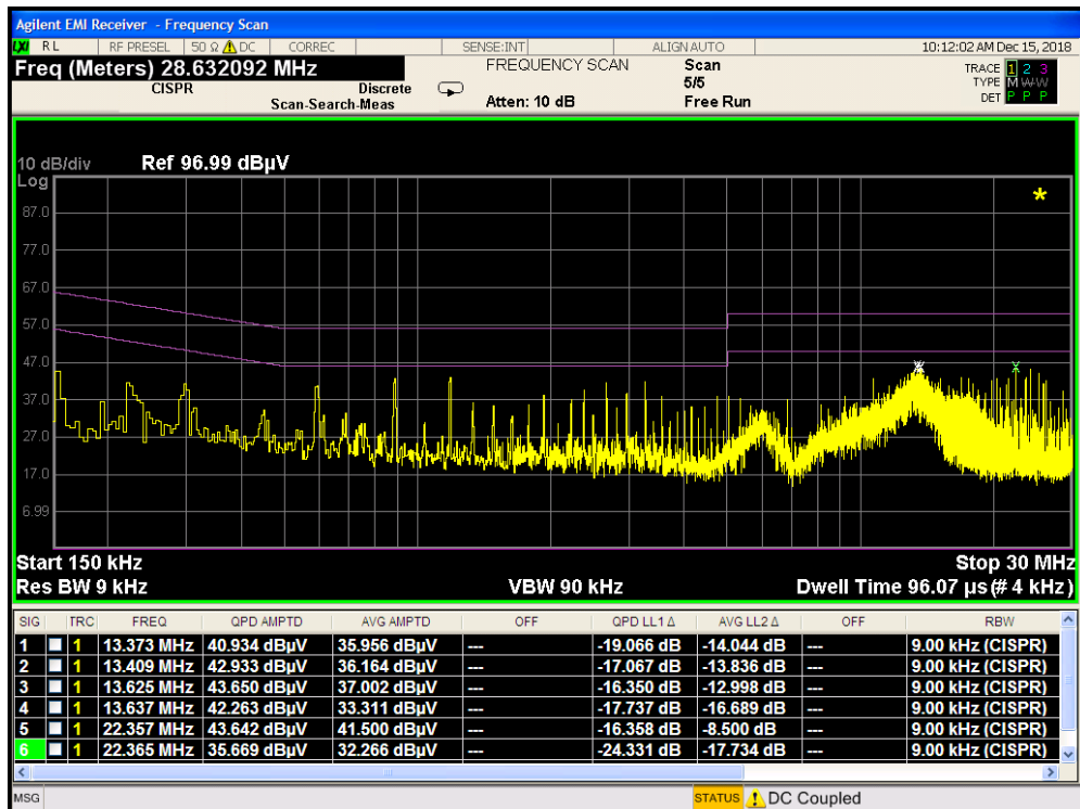
Plot 7-146. Line Conducted Plot with 802.11b (N) with Wireless Charging Pad
