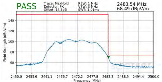
Plot 7-138. Radiated Restricted Upper Band Edge Measurement CDD (Peak)
