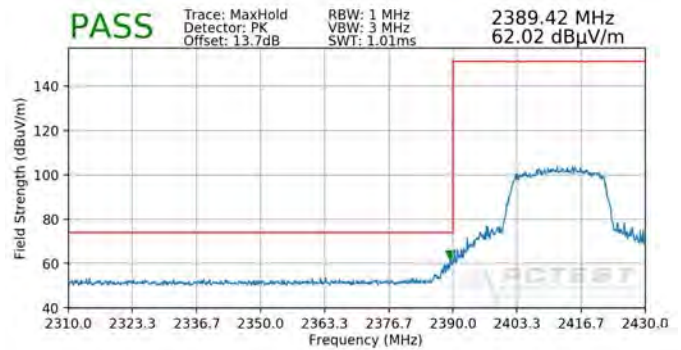
Plot 7-120. Radiated Restricted Band Edge Measurement SISO ANT2 with WCP (Peak)
