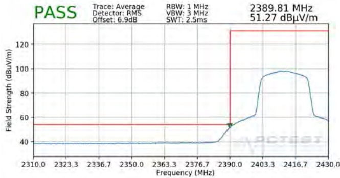
Plot 7-109. Radiated Restricted Band Edge Measurement SISO ANT1 with WCP (Average)
