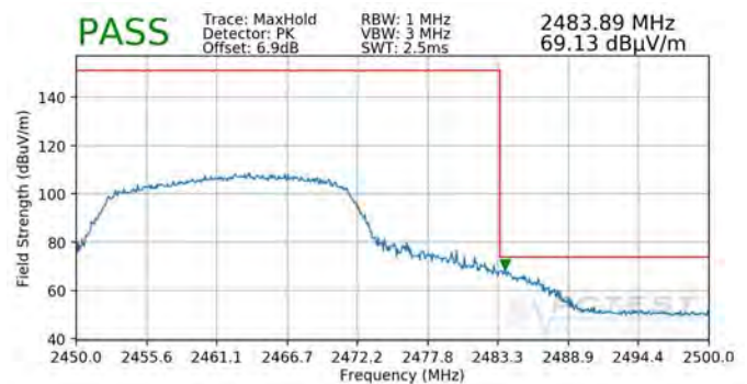
Plot 7-114. Radiated Restricted Upper Band Edge Measurement SISO ANT2 (Peak)
