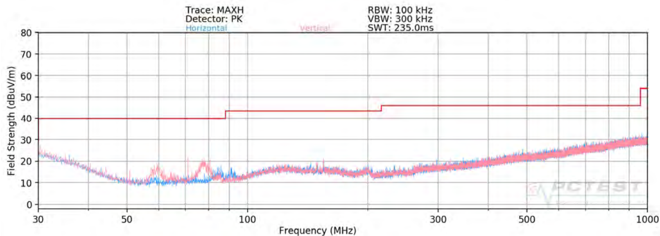
Plot 7-142. Radiated Spurious Plot below 1GHz SISO ANT2
