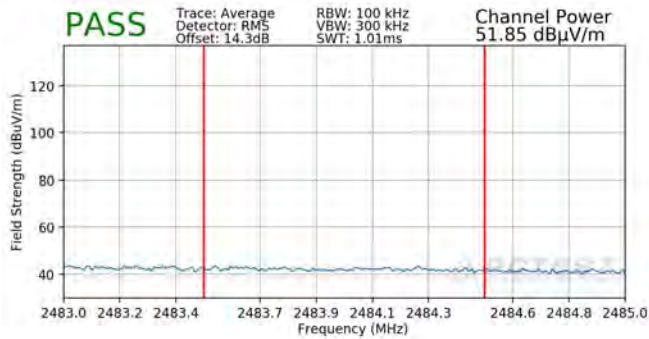
Plot 7-115. Radiated Restricted Upper Band Edge Measurement SISO ANT2 (Average)
