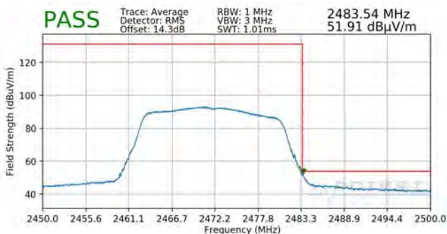
Plot 7-107. Radiated Restricted Upper Band Edge Measurement SISO ANT1 (Average)
