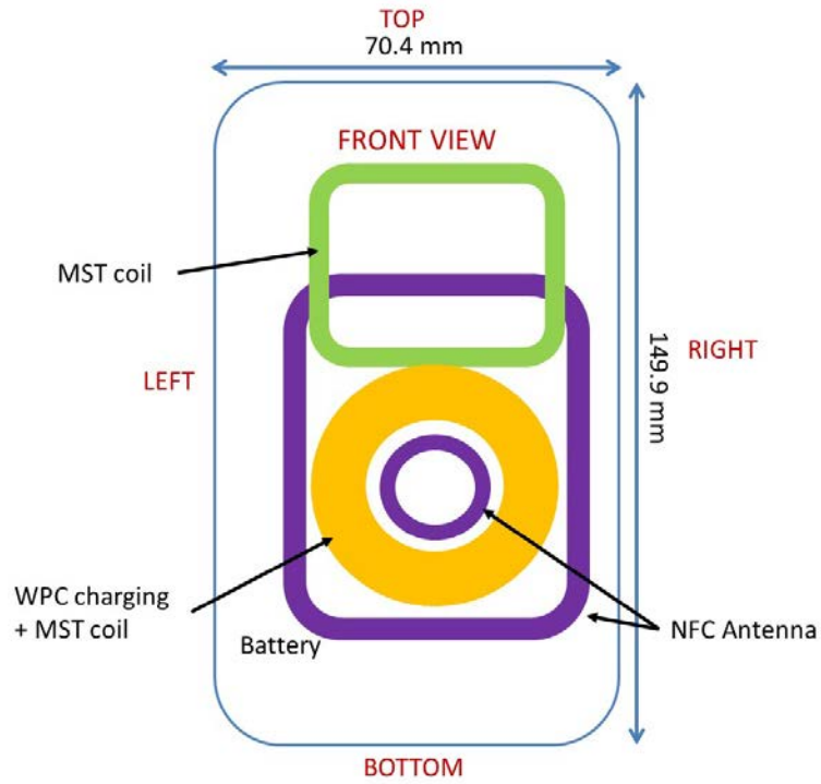
Figure F-2 NFC Antenna Locations
