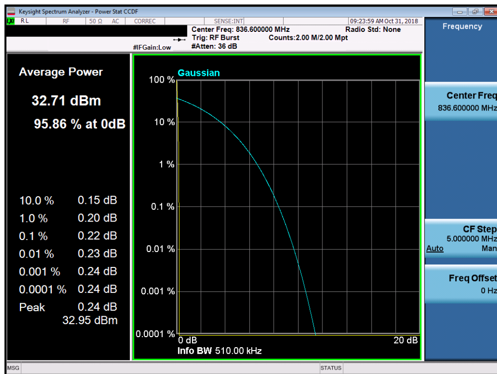
Plot 7-41. Peak-Average Ratio Plot (Cell GPRS Mode)
