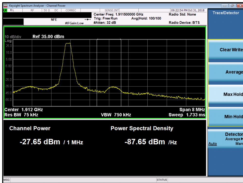
Plot 7-38. 4MHz Span Plot (PCS GSM Mode - High Channel)
