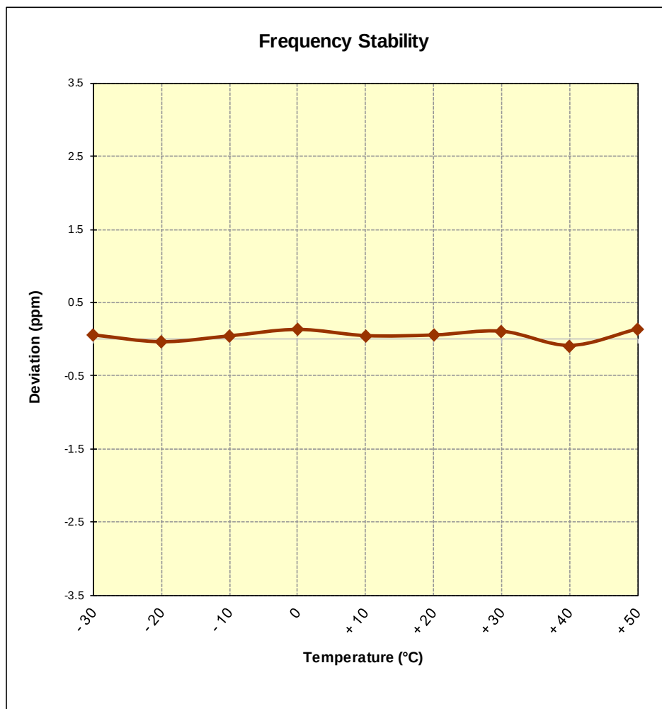
Figure 7-10. Frequency Stability Graph (PCS GPRS Mode – Ch. 661)
