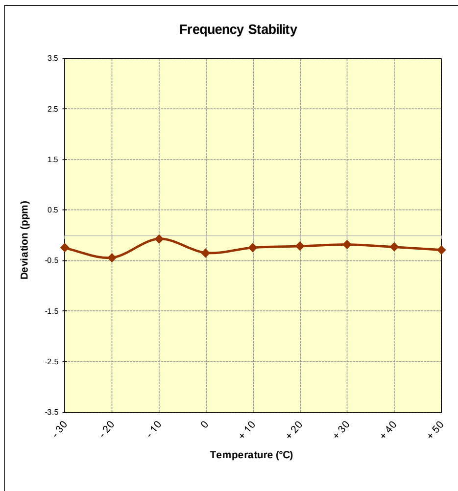
Figure 7-9. Frequency Stability Graph (Cellular WCDMA Mode – Ch. 4183)
