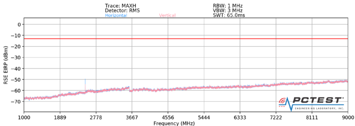
Plot 7-46. Radiated Spurious Plot above 1GHz (Cellular GPRS)
