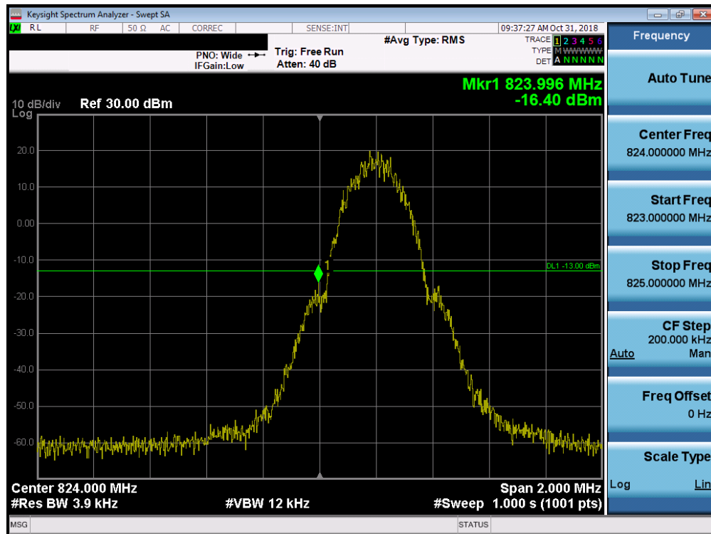
Plot 7-33. Band Edge Plot (Cellular GSM Mode - Low Channel)
