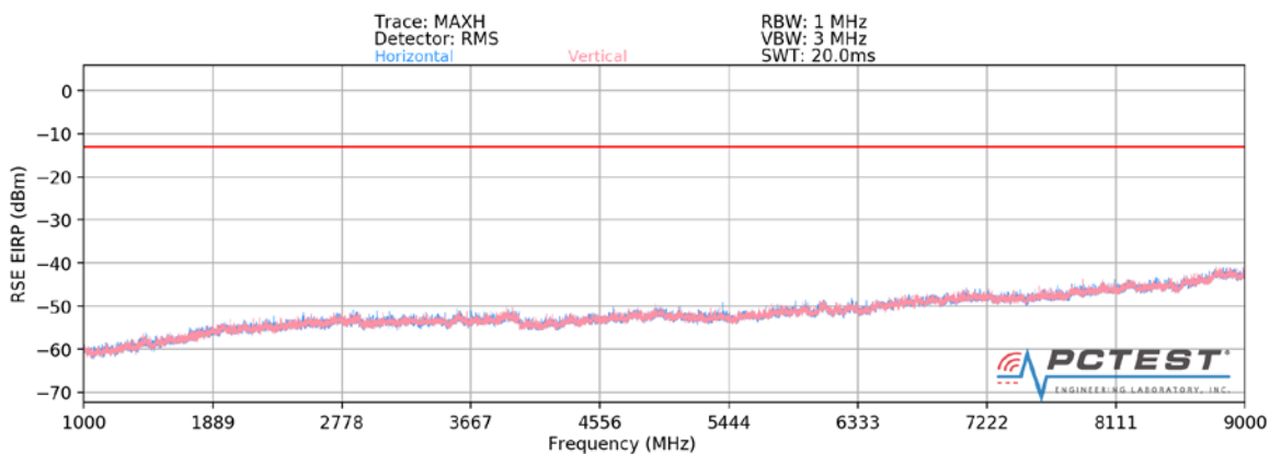
Plot 7-47. Radiated Spurious Plot above 1GHz (Cellular WCDMA)
