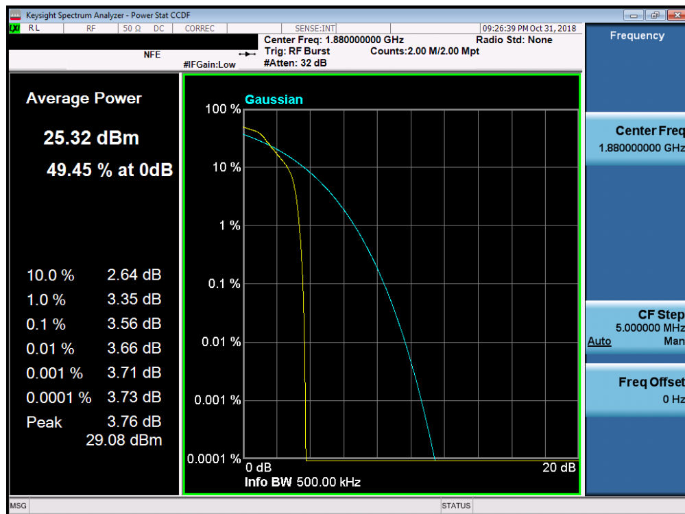
Plot 7-44. Peak-Average Ratio Plot (PCS EDGE Mode)
