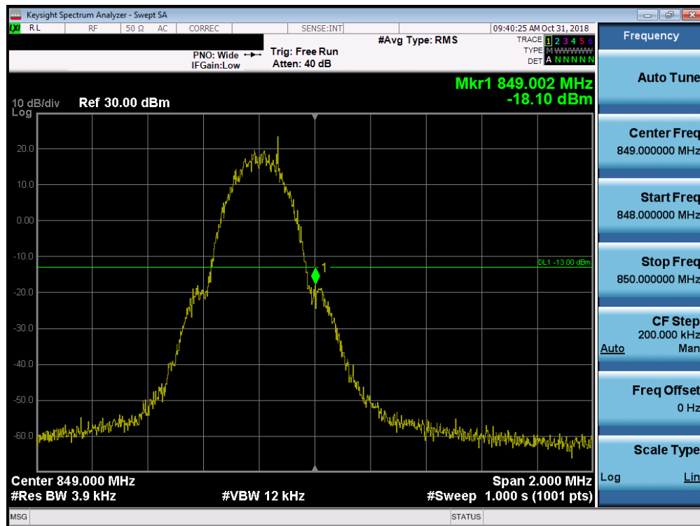
Plot 7-34. Band Edge Plot (Cellular GSM Mode - High Channel)
