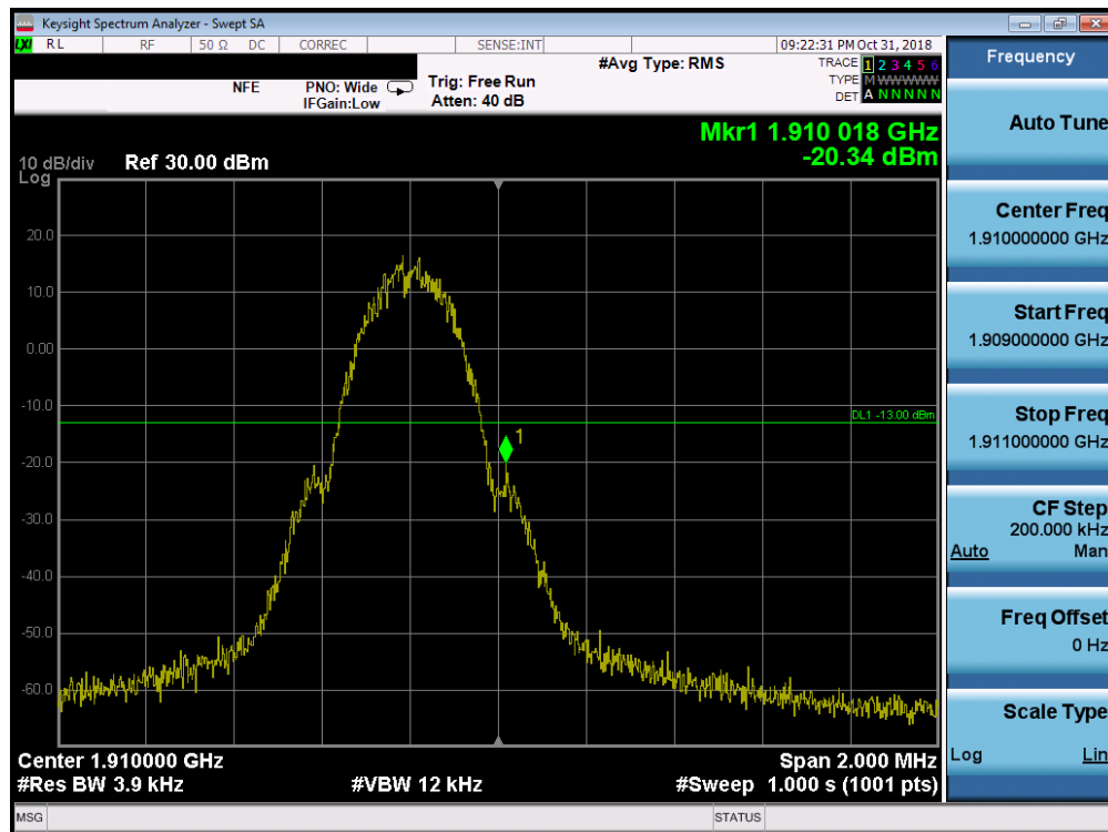
Plot 7-37. Band Edge Plot (PCS GSM Mode - High Channel)
