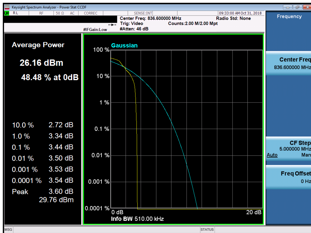
Plot 7-42. Peak-Average Ratio Plot (Cell EDGE Mode)
