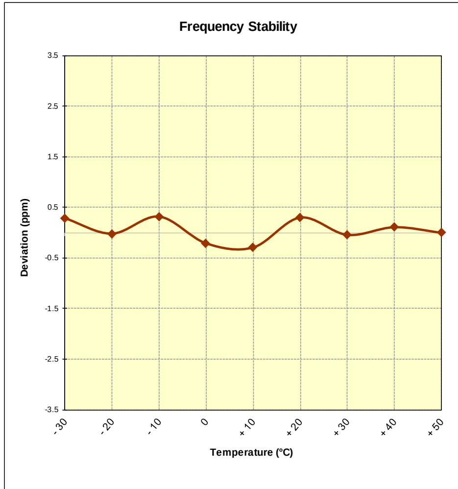
Figure 7-8. Frequency Stability Graph (Cellular GPRS Mode – Ch. 190)
