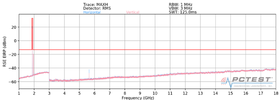
Plot 7-48. Radiated Spurious Plot above 1GHz (PCS GPRS)
