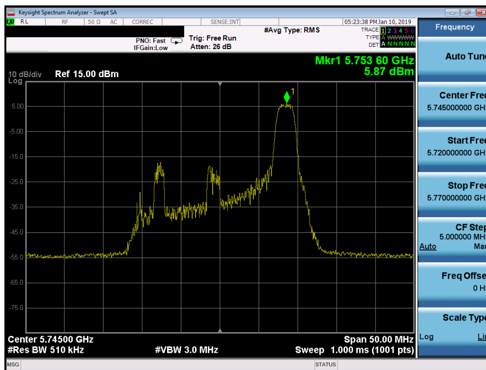
Plot 7-130. Power Spectral Density Plot SISO ANT1 (20MHz BW 802.11ax – 26 Tones (UNII Band 3) – Ch. 149)
