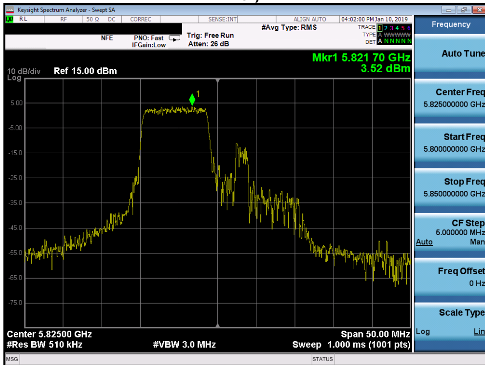
Plot 7-315. Power Spectral Density Plot SISO ANT2 (20MHz BW 802.11ax – 106 Tones (UNII Band 3) – Ch. 165)
