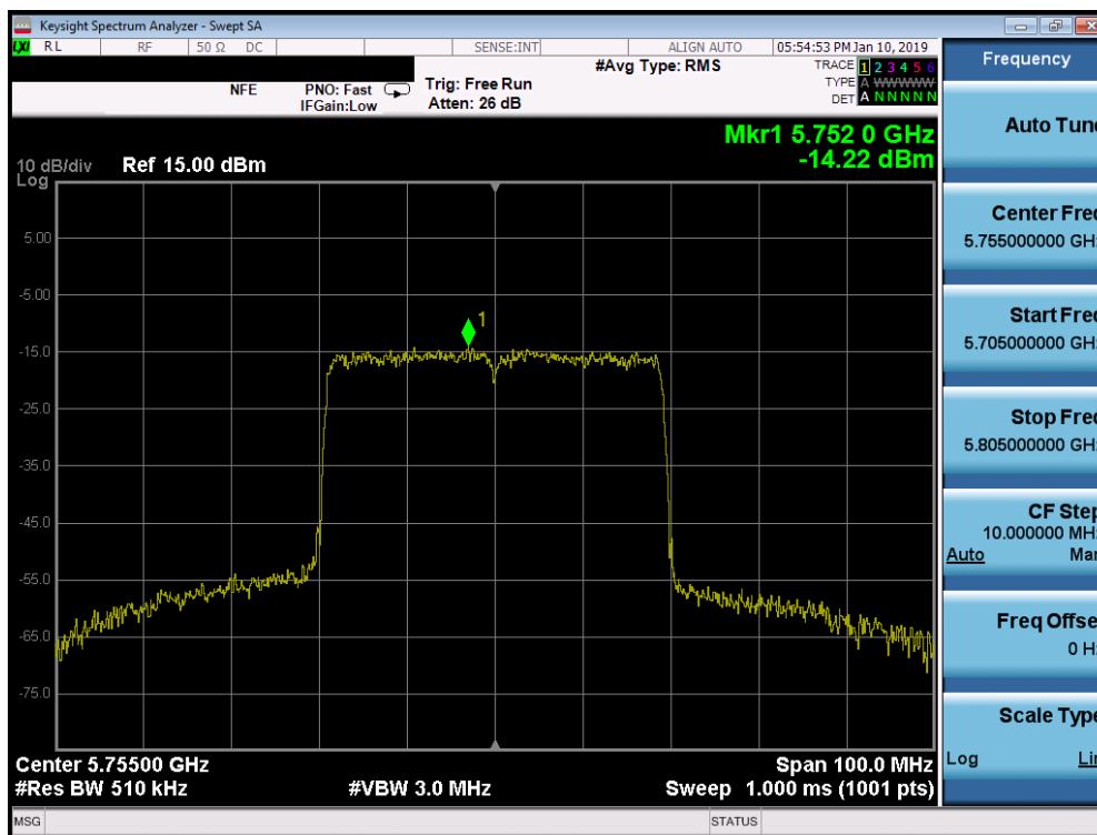
Plot 7-358. Power Spectral Density Plot SISO ANT2 (40MHz BW 802.11ax – 484 Tones (UNII Band 3) – Ch. 151)
