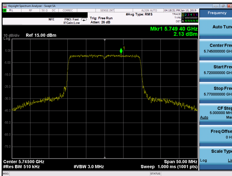
Plot 7-340. Power Spectral Density Plot SISO ANT2 (20MHz BW 802.11ax – 242 Tones (UNII Band 3) – Ch. 149)
