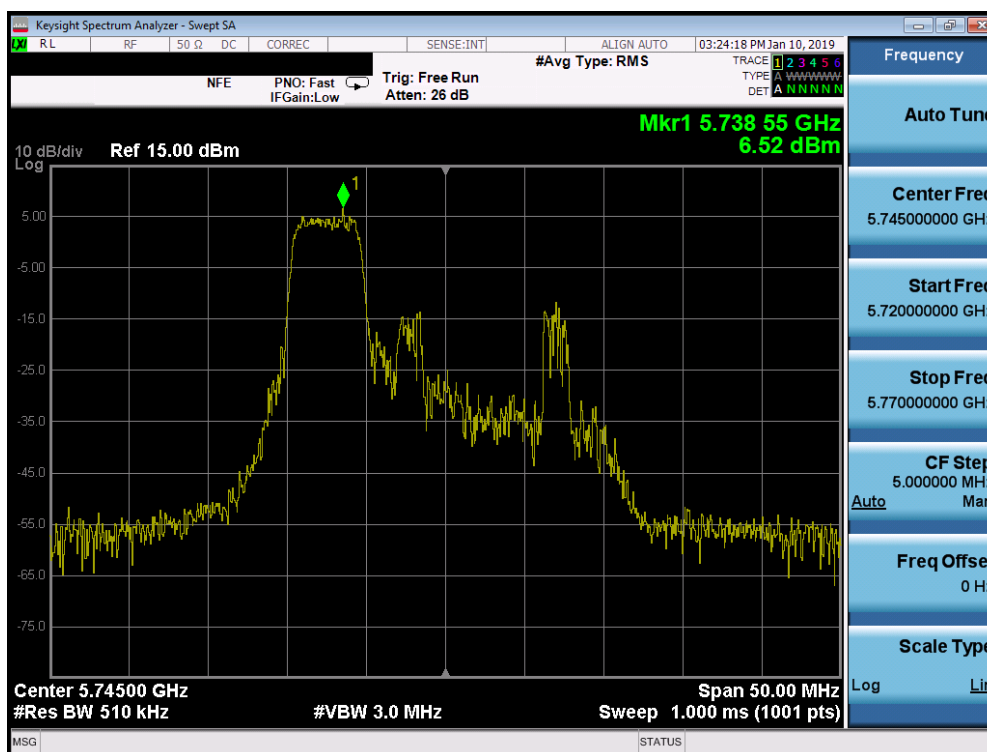
Plot 7-286. Power Spectral Density Plot SISO ANT2 (20MHz BW 802.11ax – 52 Tones (UNII Band 3) – Ch. 149)
