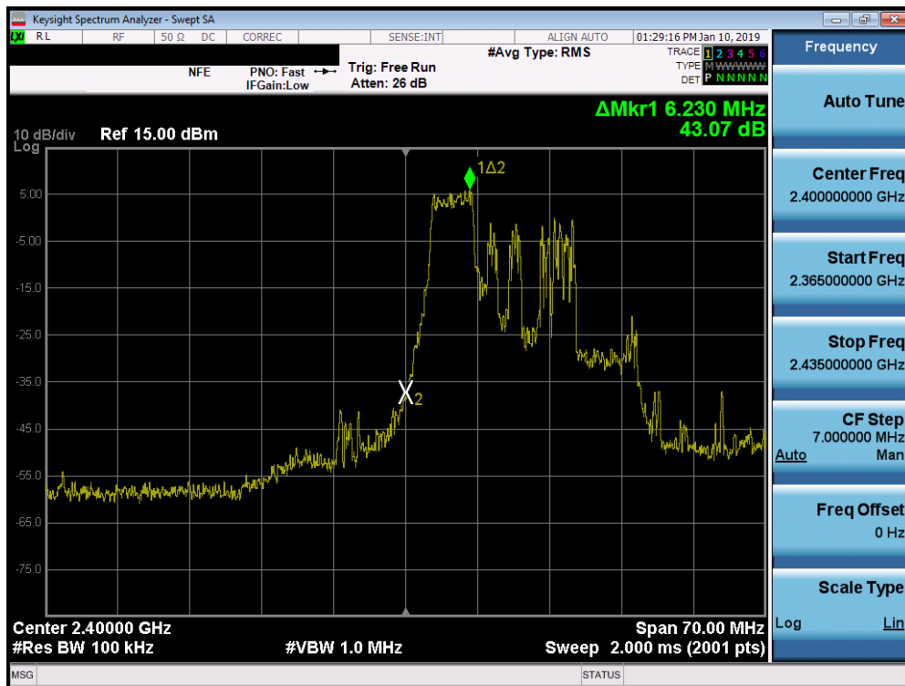
Plot 7-83. Band Edge Plot SISO ANT2 (802.11ax OFDMA – 52 Tones – Ch. 1)
