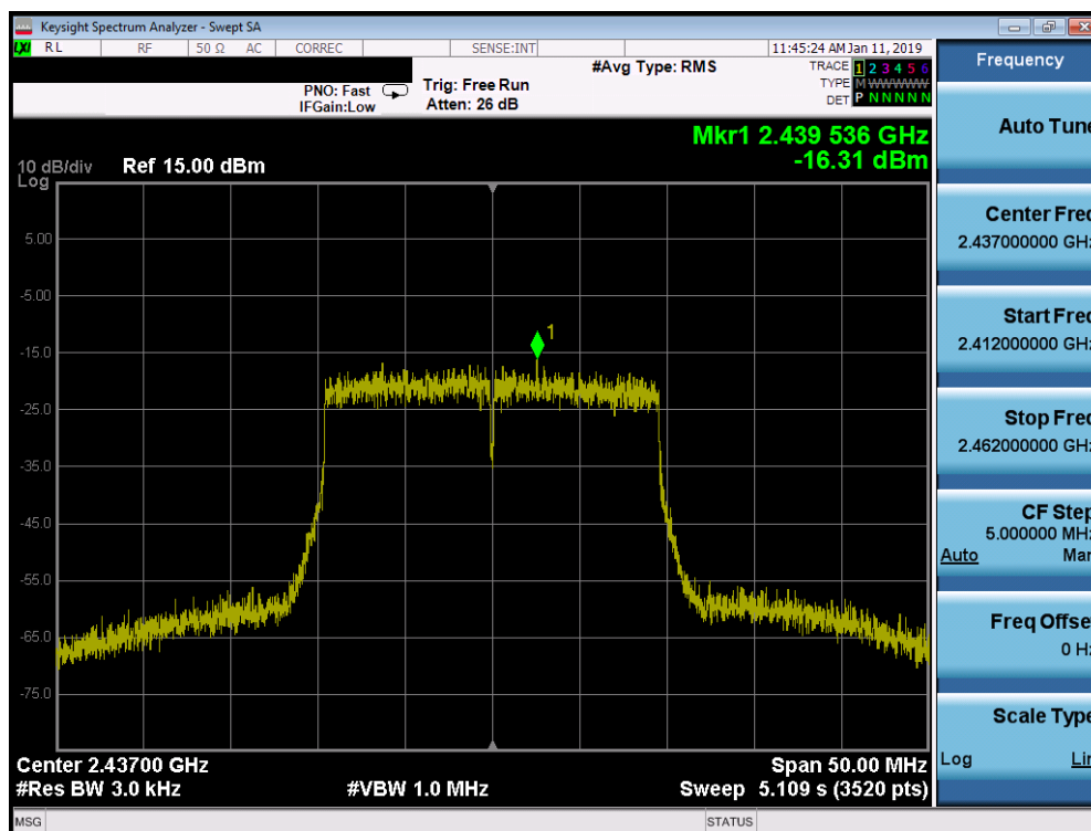
Plot 7-59. Power Spectral Density Plot SISO MIMO ANT1 (802.11ax OFDMA – 242 Tones – Ch. 6)
