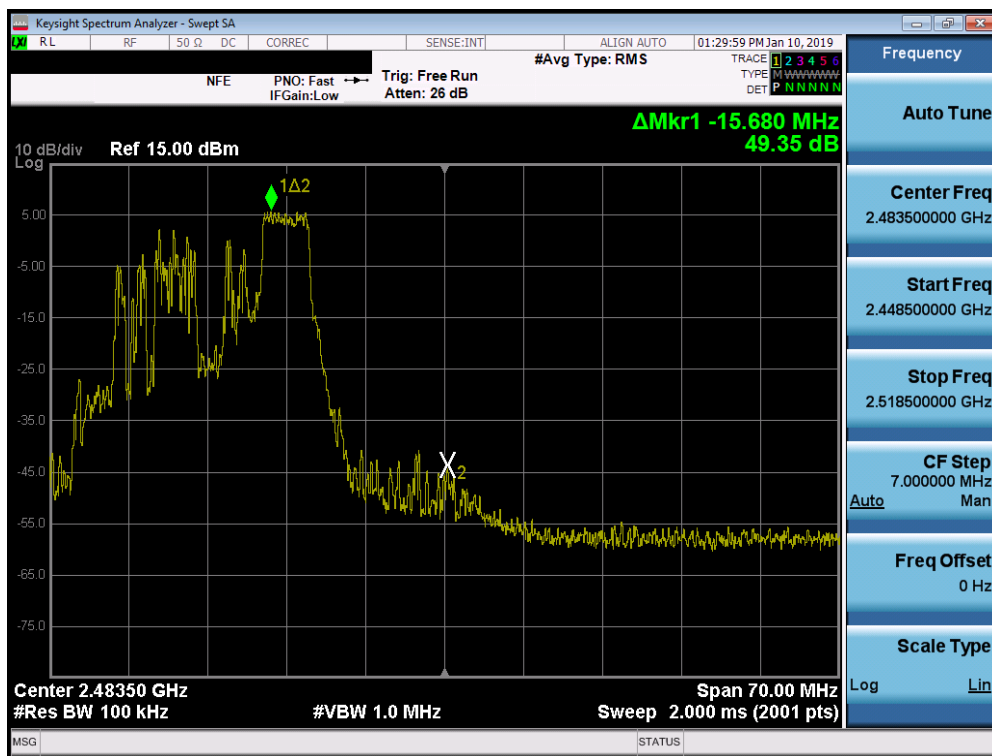
Plot 7-84. Band Edge Plot SISO ANT2 (802.11ax OFDMA – 52 Tones – Ch. 11)
