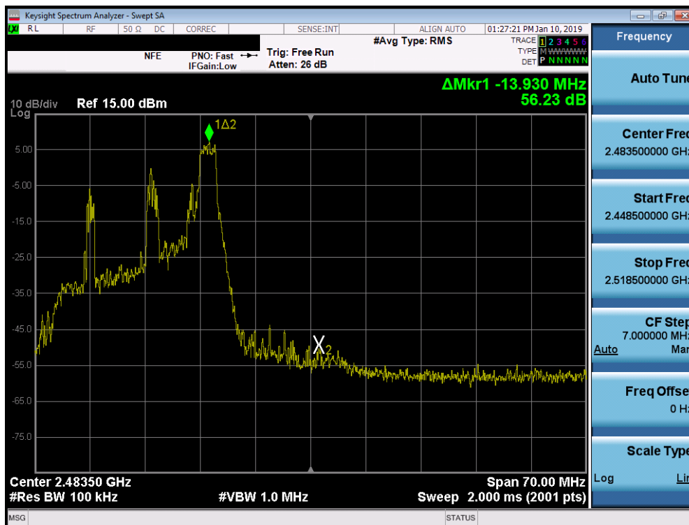
Plot 7-82. Band Edge Plot SISO ANT2 (802.11ax OFDMA - 26 Tones - Ch. 11)
