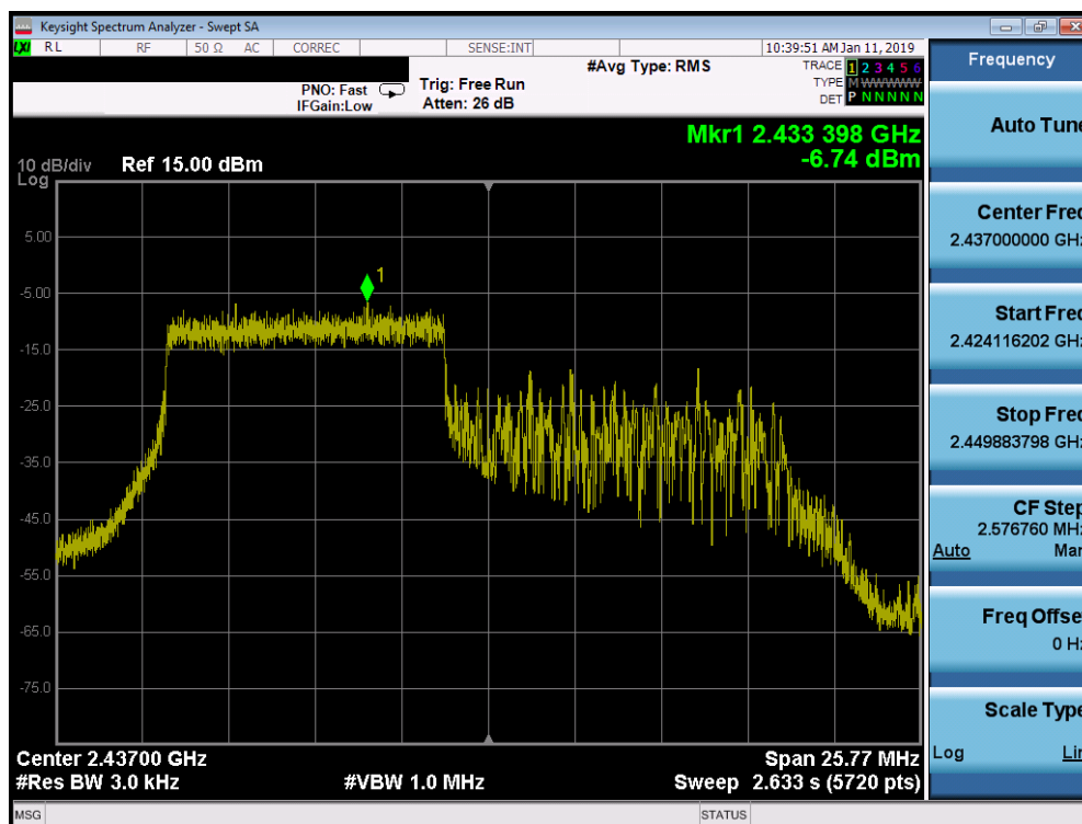
Plot 7-32. Power Spectral Density Plot SISO ANT1 (802.11ax OFDMA – 106 Tones – Ch. 6)
