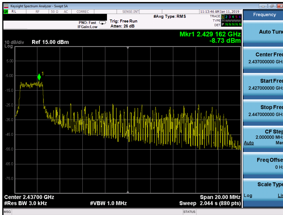
Plot 7-62. Power Spectral Density Plot SISO MIMO ANT2 (802.11ax OFDMA – 26 Tones – Ch. 6)
