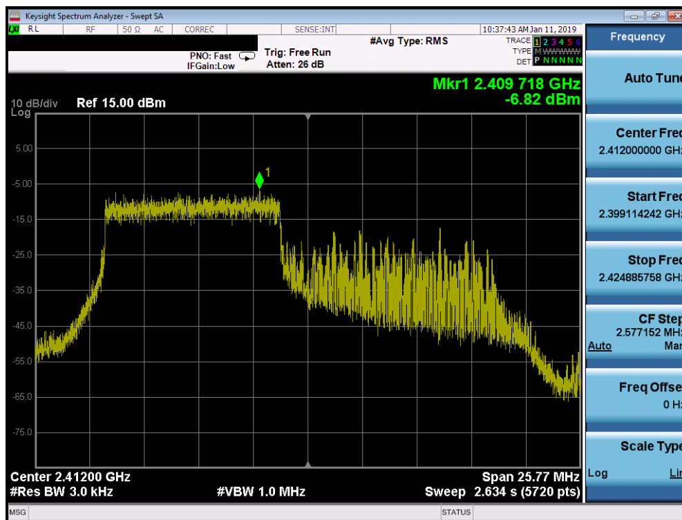
Plot 7-31. Power Spectral Density Plot SISO ANT1 (802.11ax OFDMA – 106 Tones – Ch. 1)
