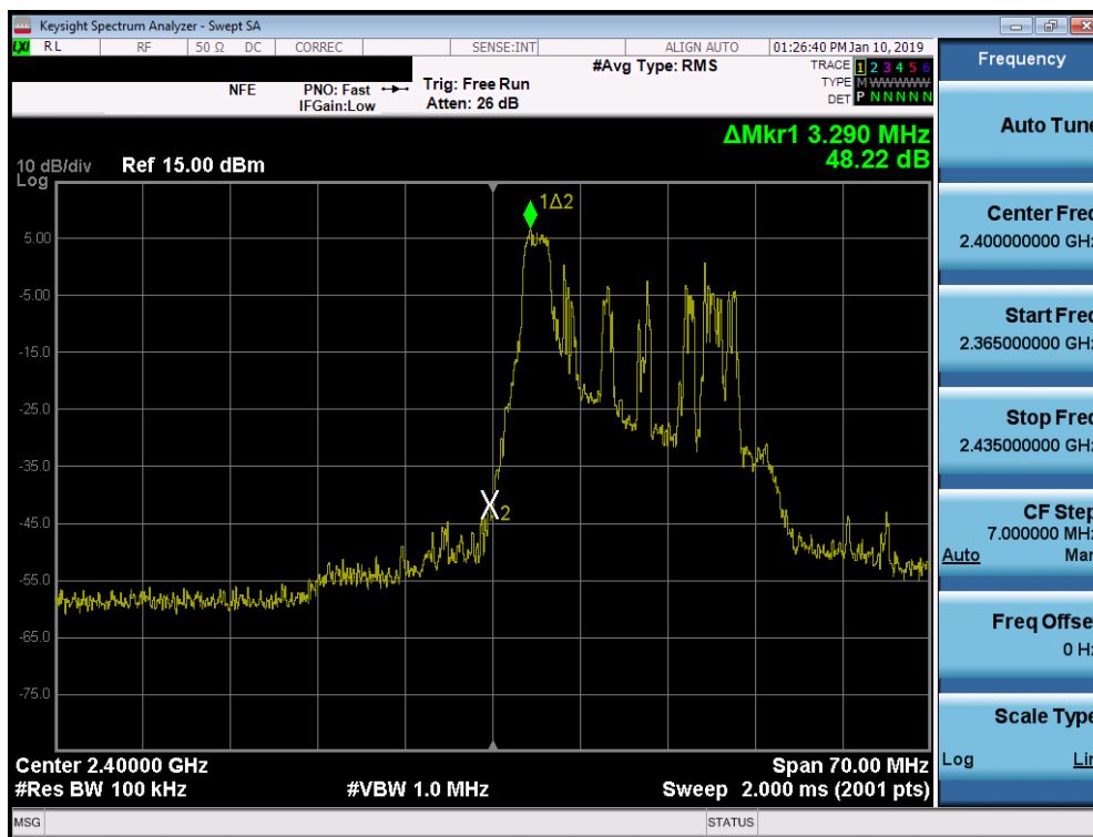
Plot 7-81. Band Edge Plot SISO ANT2 (802.11ax OFDMA - 26 Tones - Ch. 1)
