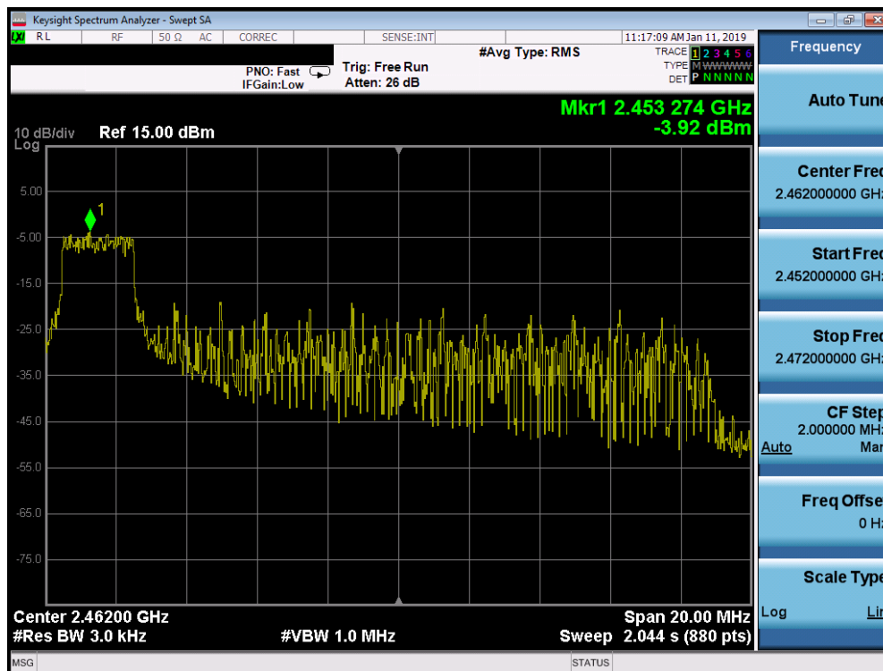
Plot 7-63. Power Spectral Density Plot SISO MIMO ANT2 (802.11ax OFDMA – 26 Tones – Ch. 11)
