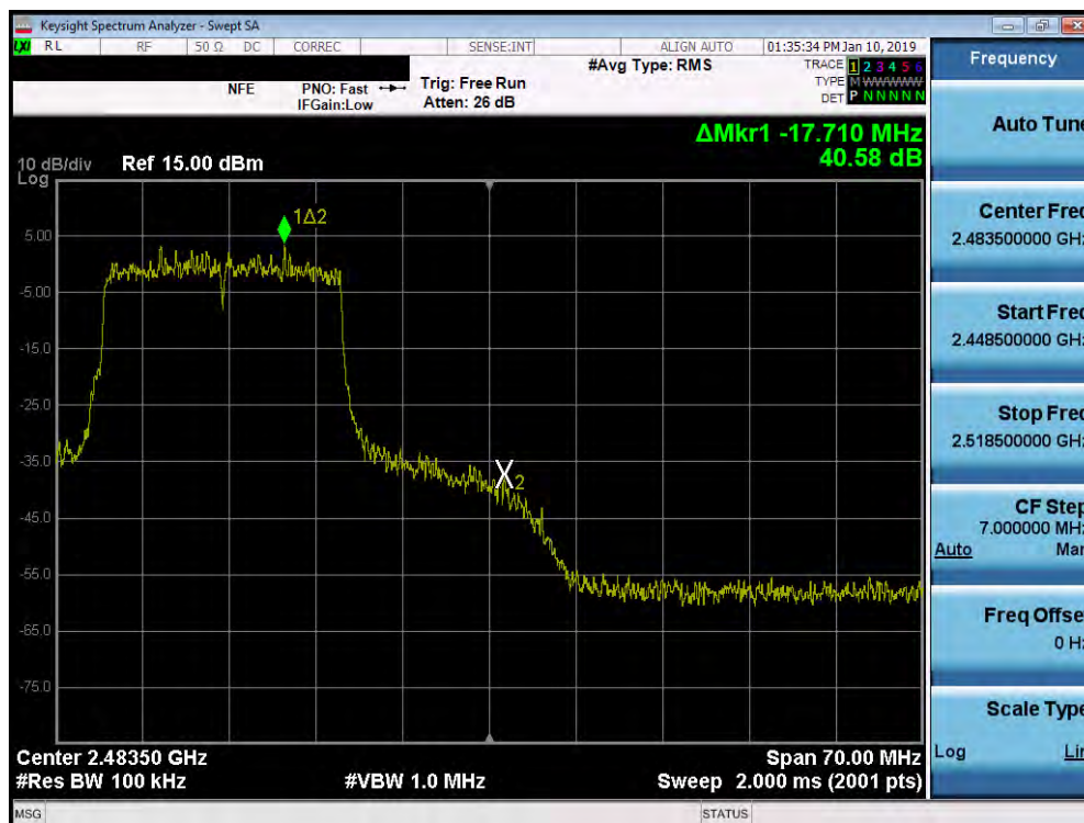
Plot 7-88. Band Edge Plot SISO ANT2 (802.11ax OFDMA – 242 Tones – Ch. 11)
