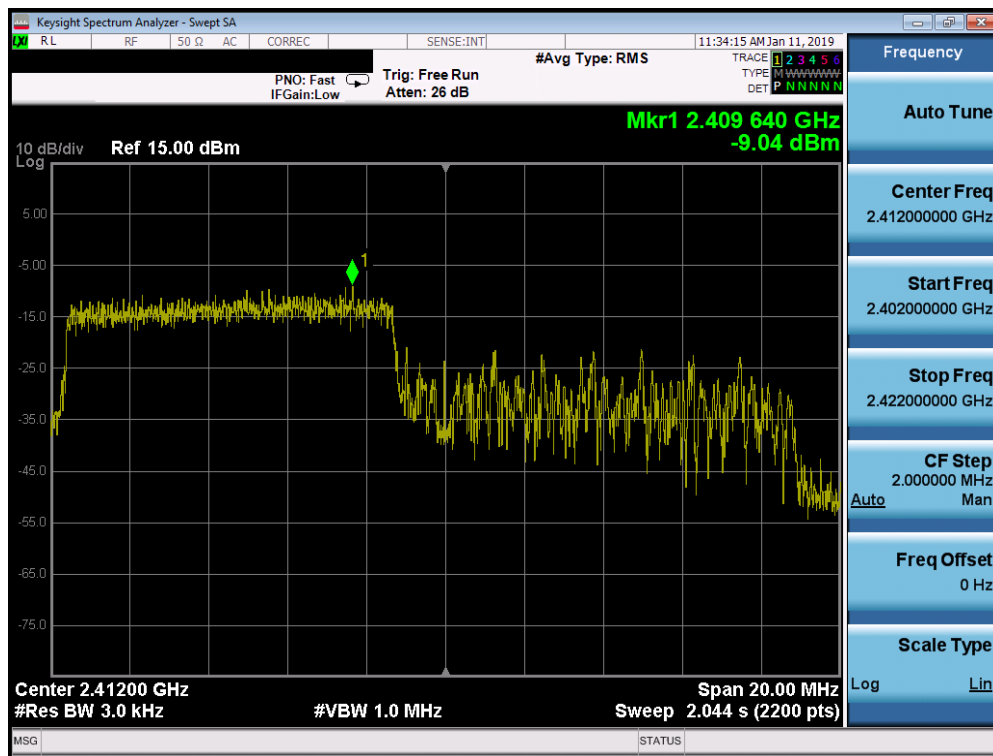
Plot 7-67. Power Spectral Density Plot SISO MIMO ANT2 (802.11ax OFDMA – 106 Tones – Ch. 1)
