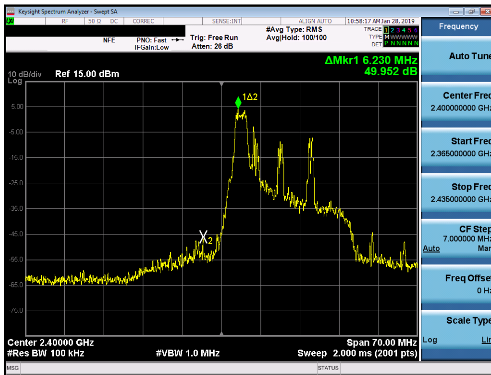
Plot 7-73. Band Edge Plot SISO ANT1 (802.11ax OFDMA – 26 Tones – Ch. 1)
