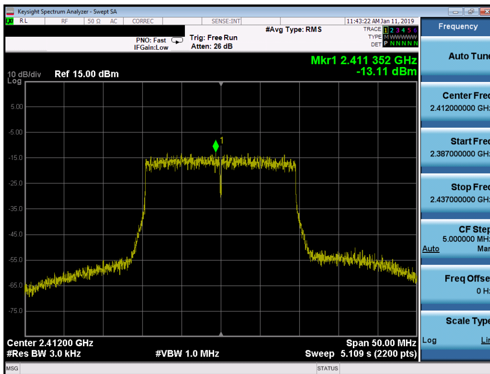
Plot 7-70. Power Spectral Density Plot SISO MIMO ANT2 (802.11ax OFDMA – 242 Tones – Ch. 1)
