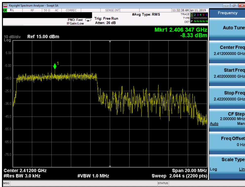
Plot 7-55. Power Spectral Density Plot SISO MIMO ANT1 (802.11ax OFDMA – 106 Tones – Ch. 1)
