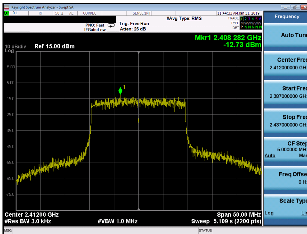
Plot 7-58. Power Spectral Density Plot SISO MIMO ANT1 (802.11ax OFDMA – 242 Tones – Ch. 1)
