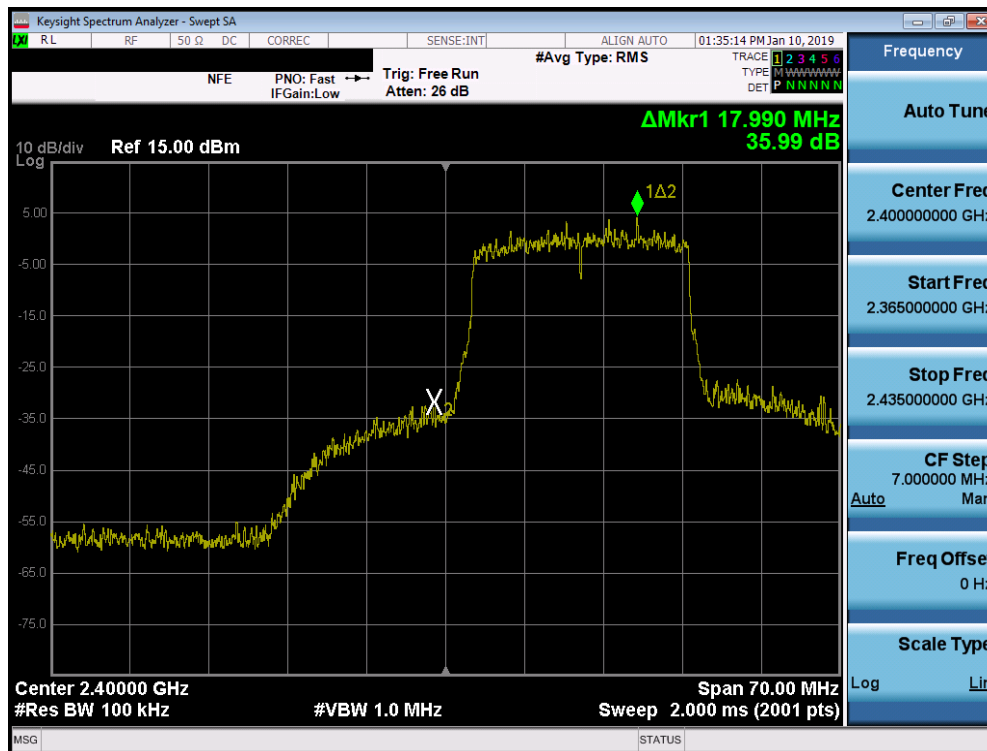
Plot 7-87. Band Edge Plot SISO ANT2 (802.11ax OFDMA – 242 Tones – Ch. 1)
