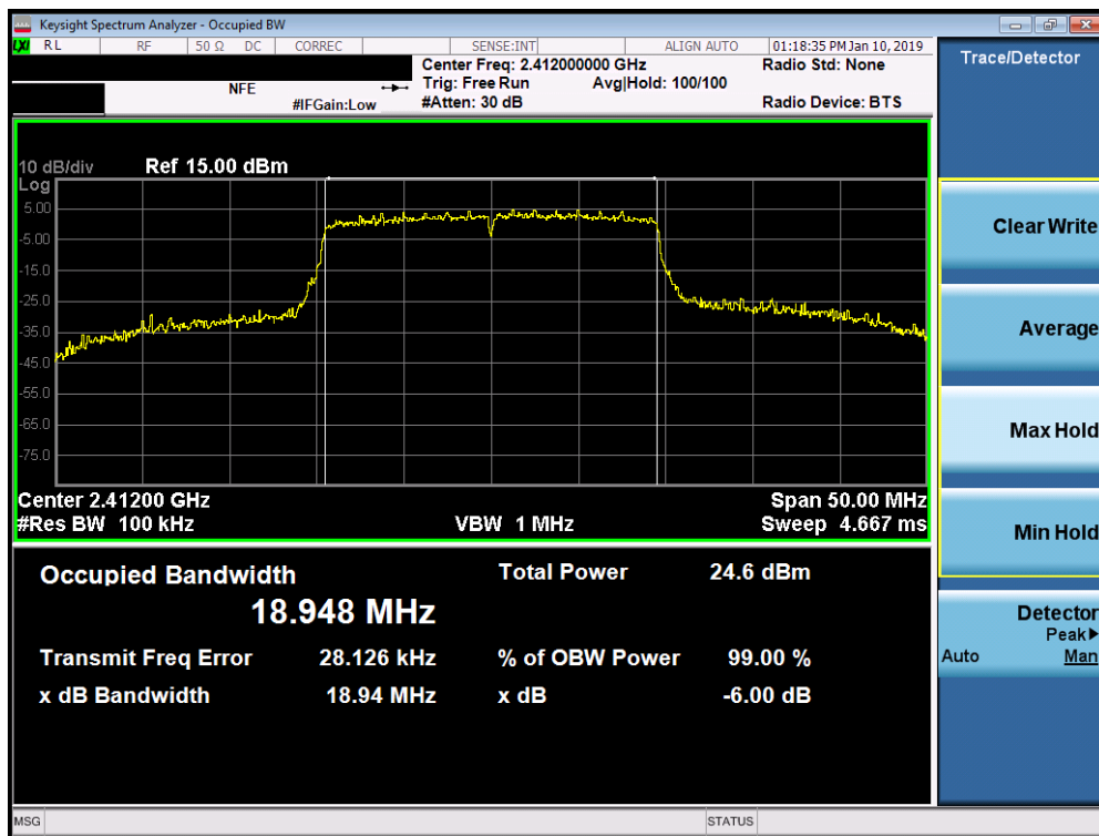
Plot 7-22. 6dB Bandwidth Plot SISO ANT2 (802.11ax OFDMA – 242 Tones – Ch. 1)
