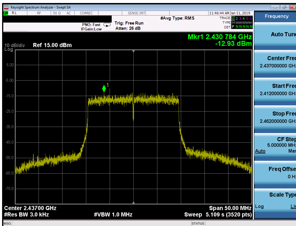
Plot 7-71. Power Spectral Density Plot SISO MIMO ANT2 (802.11ax OFDMA – 242 Tones – Ch. 6)
