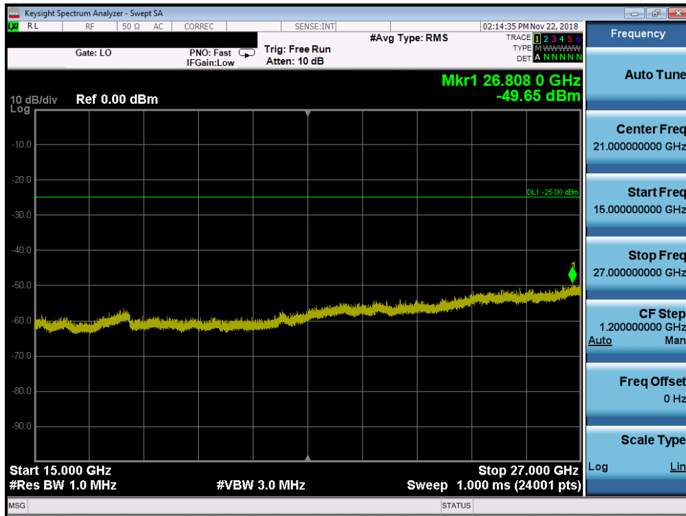
Plot 7-93. Conducted Spurious (Band 41 PC3 - 15.0MHz QPSK -RB Size 1, RB Offset 0 -Low Channel)
