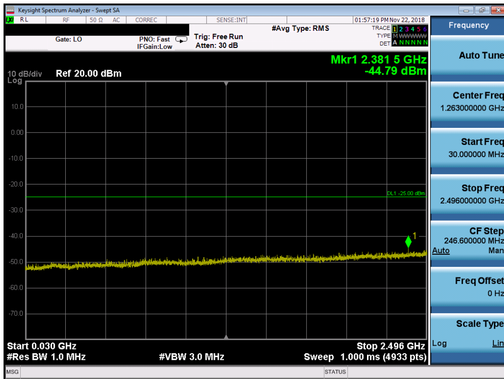
Plot 7-94. Conducted Spurious (Band 41 PC3 - 15.0MHz QPSK -RB Size 1, RB Offset 0 -Mid Channel)
