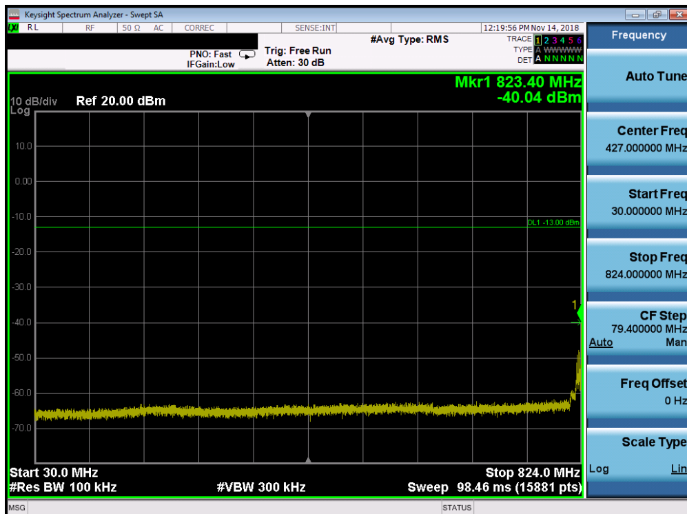
Plot 7-76. Conducted Spurious Plot (Band 5 - 5.0MHz QPSK - RB Size 1, RB Offset 0 - Mid Channel)
