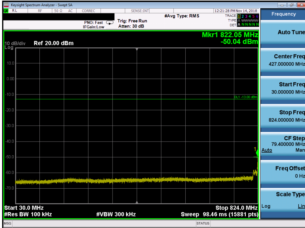
Plot 7-79. Conducted Spurious Plot (Band 5 - 5.0MHz QPSK - RB Size 1, RB Offset 0 - High Channel)
