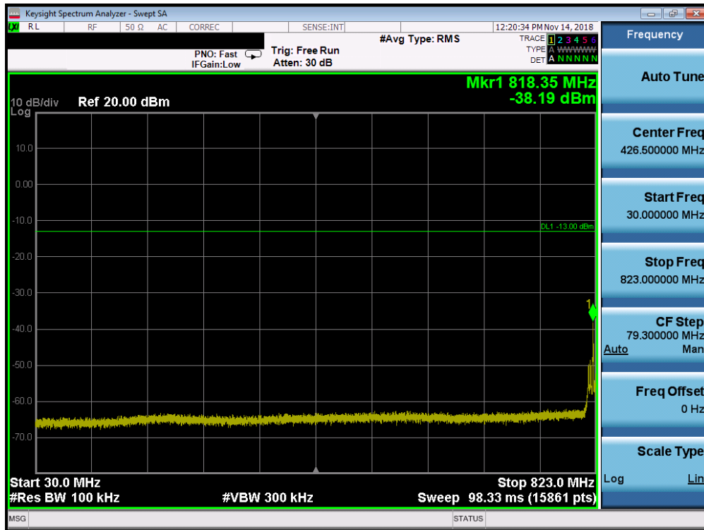
Plot 7-73. Conducted Spurious Plot (Band 5 - 5.0MHz QPSK - RB Size 1, RB Offset 0 - Low Channel)
