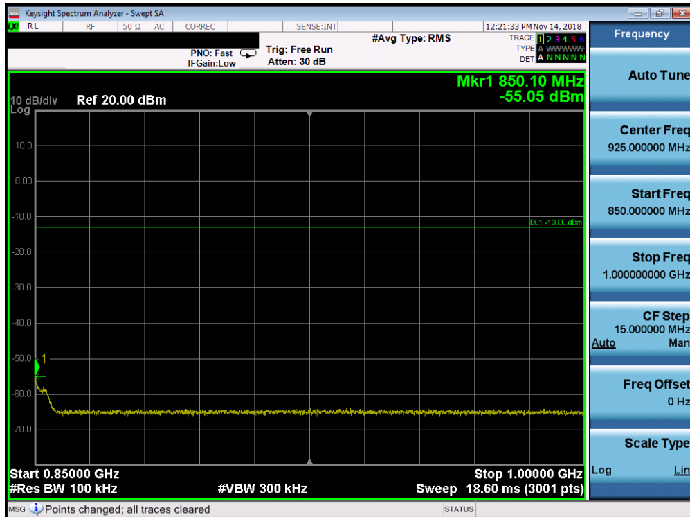
Plot 7-80. Conducted Spurious Plot (Band 5 - 5.0MHz QPSK - RB Size 1, RB Offset 0 - High Channel)
