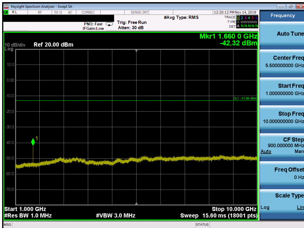
Plot 7-78. Conducted Spurious Plot (Band 5 - 5.0MHz QPSK - RB Size 1, RB Offset 0 - Mid Channel)
