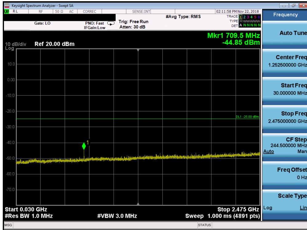
Plot 7-91. Conducted Spurious (Band 41 PC3 - 15.0MHz QPSK -RB Size 1, RB Offset 0 -Low Channel)
