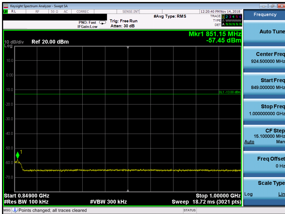
Plot 7-74. Conducted Spurious Plot (Band 5 - 5.0MHz QPSK - RB Size 1, RB Offset 0 - Low Channel)
