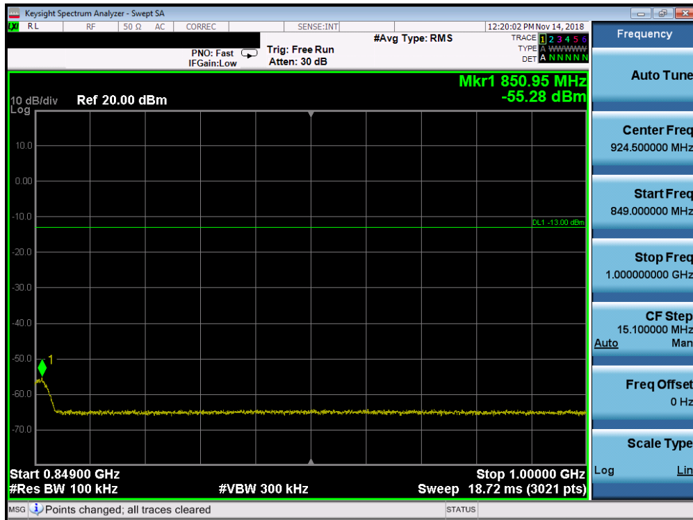
Plot 7-77. Conducted Spurious Plot (Band 5 - 5.0MHz QPSK - RB Size 1, RB Offset 0 - Mid Channel)
