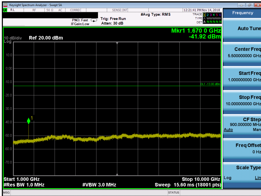
Plot 7-81. Conducted Spurious Plot (Band 5 - 5.0MHz QPSK - RB Size 1, RB Offset 0 - High Channel)
