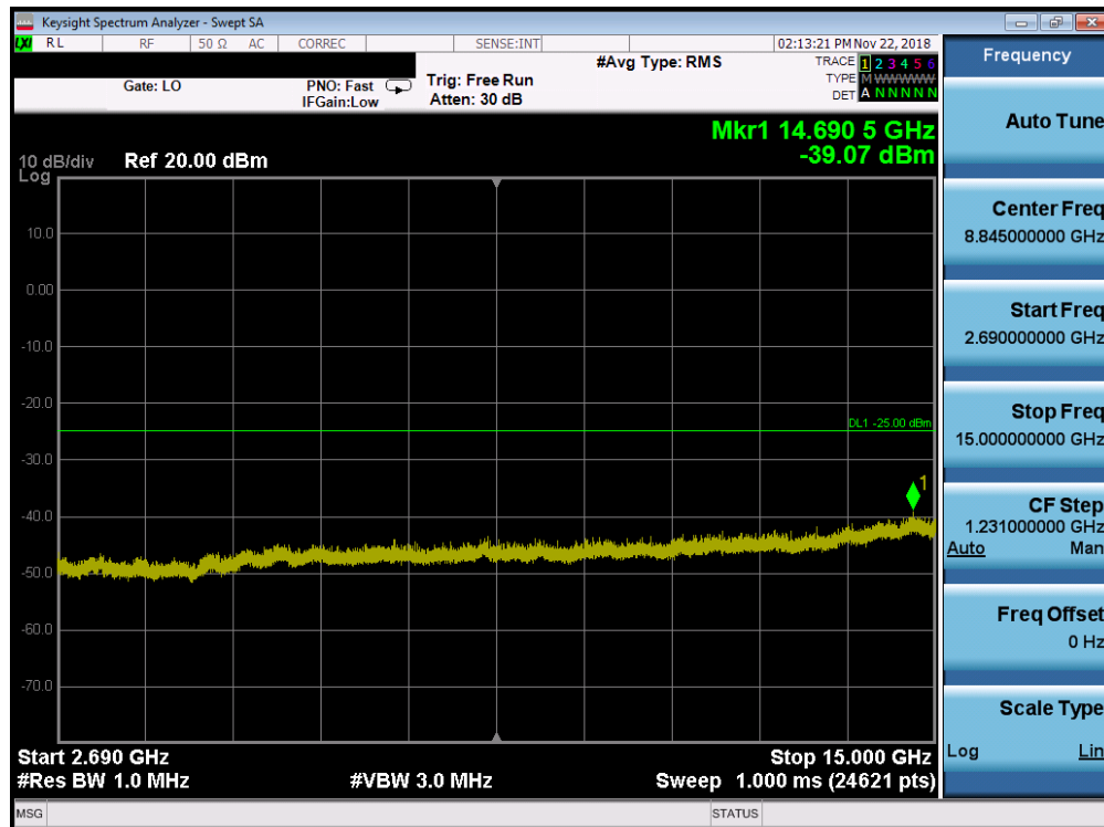
Plot 7-92. Conducted Spurious (Band 41 PC3- 15.0MHz QPSK - RB Size 1, RB Offset 0 -Low Channel)
