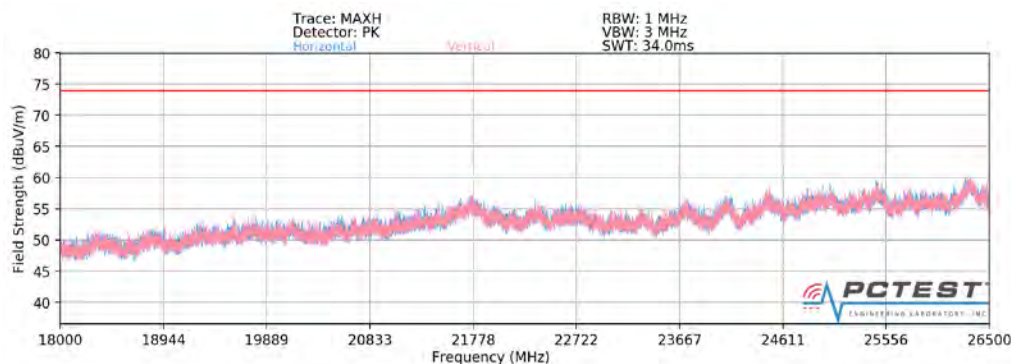
Plot 7-290. Radiated Spurious Plot 18GHz – 26.5GHz (Dual Band Simult. Tx)
