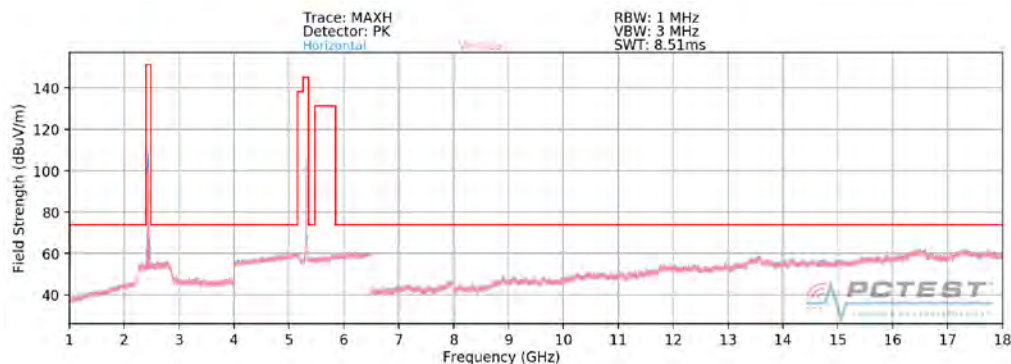
Plot 7-289. Radiated Spurious Plot above 1GHz (Dual Band Simult. Tx)
