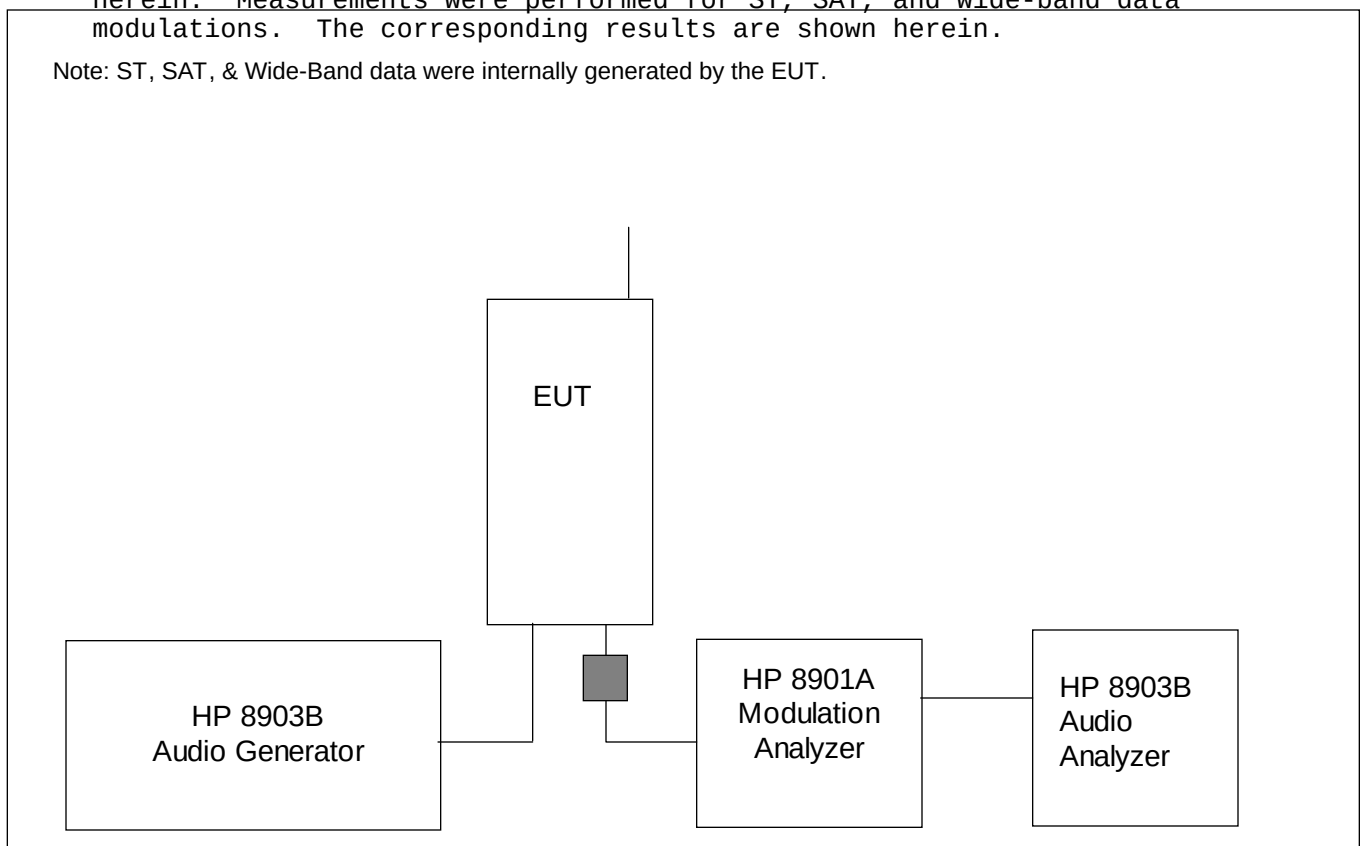
Fig. 3. Transmitter Audio Frequency & Tone Modulation Test Setup.
