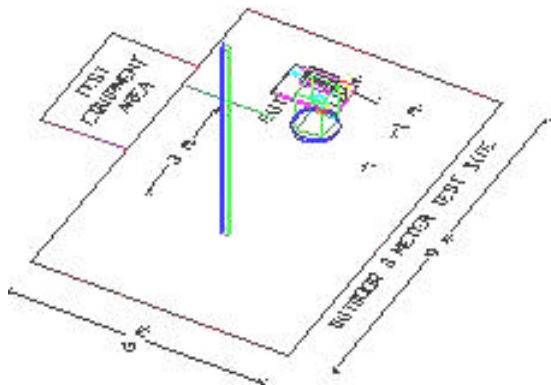
Figure 2. 3-meter Outdoor Test Range
