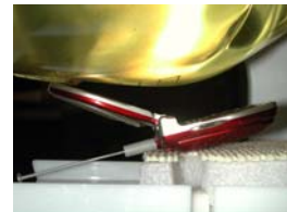
Figure 14.5 Right Head SAR Test Setup -- Ear / 15° Tilt Position --
