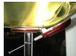
Figure 14.4 Right Head SAR Test Setup -- Cheek / Touch Position --
