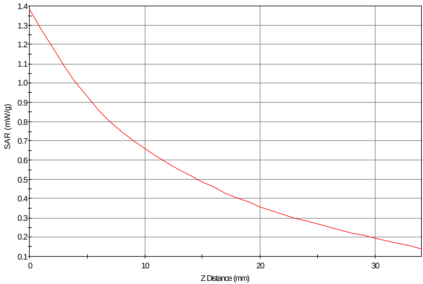
SAR - Z Axis at Hotspot x:66.0 y:13.0
