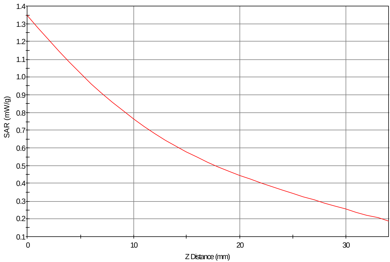
SAR - Z Axis at Hotspot x:68.0 y:8.0
