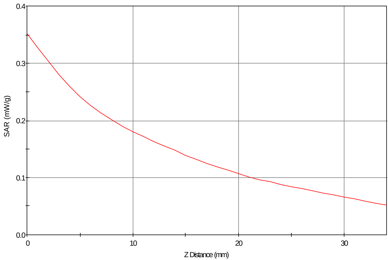
SAR - Z Axis at Hotspot x:30.0 y:-3.0
