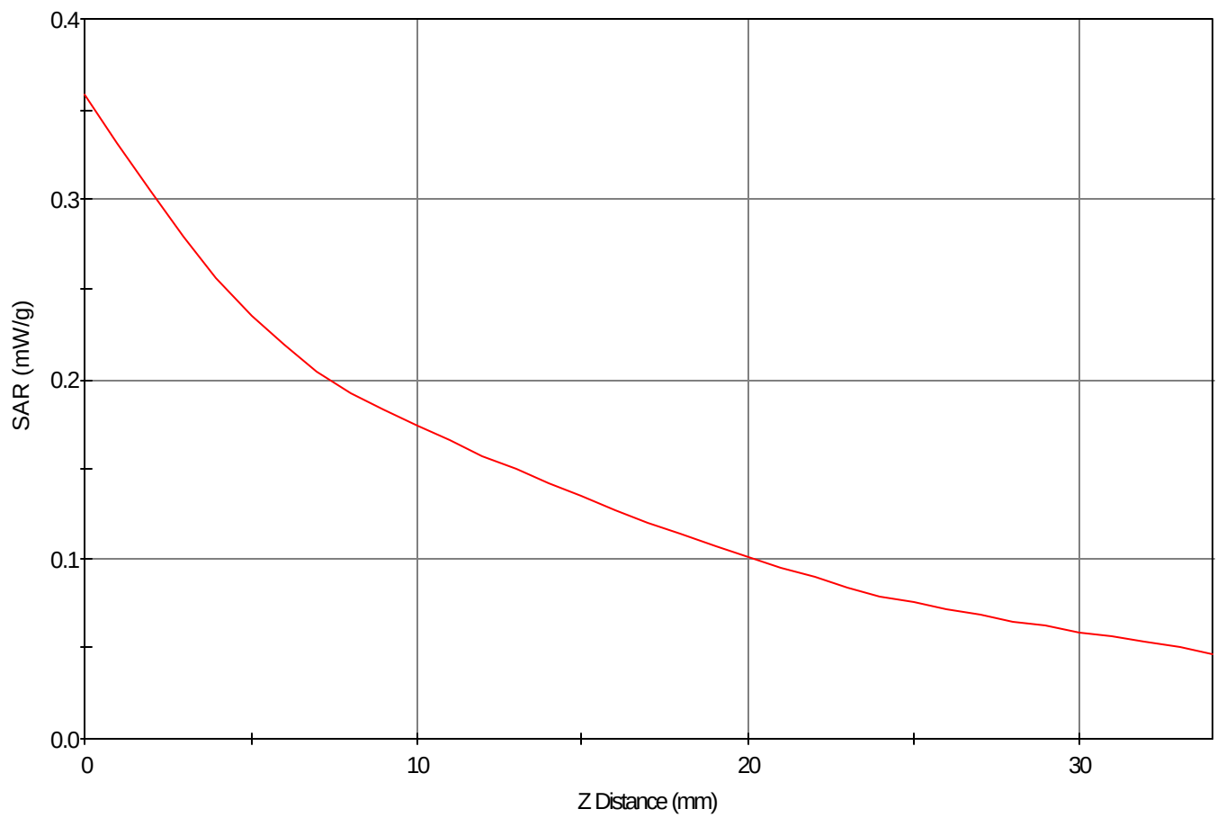
SAR - Z Axis at Hotspot x:32.0 y:3.0
