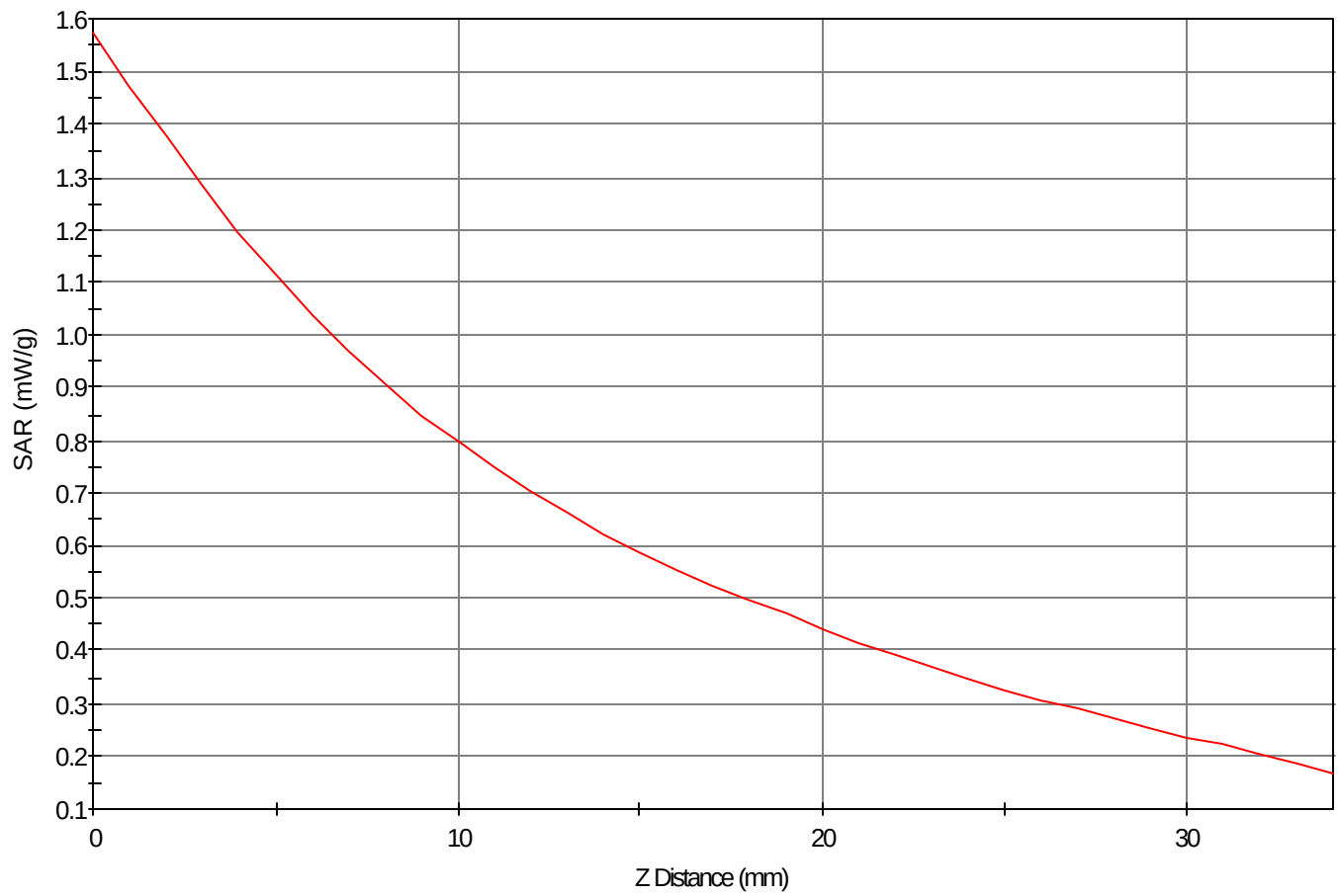
SAR - Z Axis at Hotspot x:64.0 y:12.0
