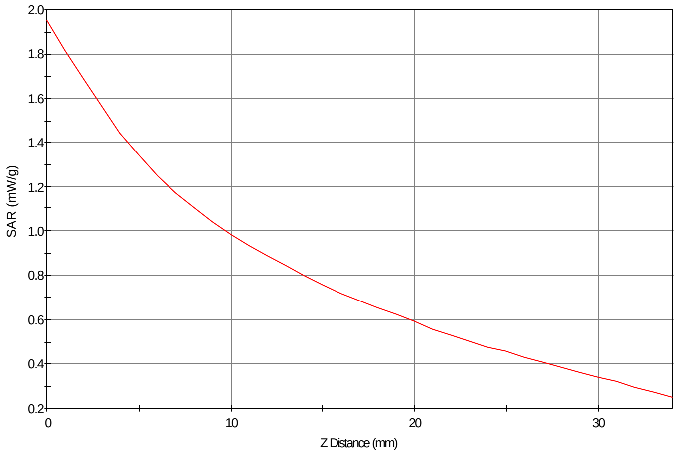
SAR - Z Axis at Hotspot x:67.0 y:10.0
