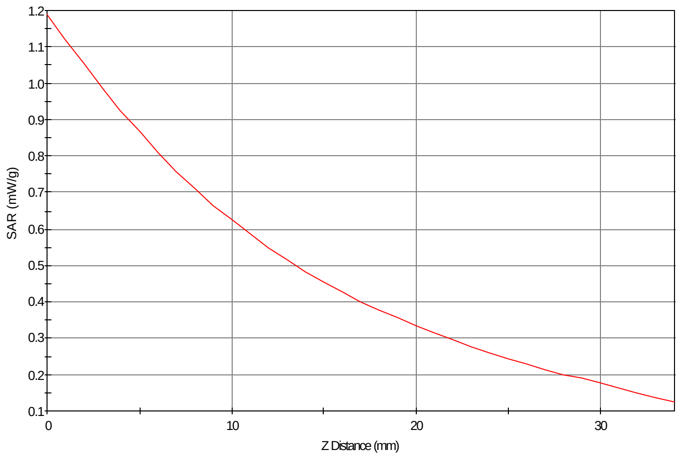
SAR - Z Axis at Hotspot x:70.0 y:17.0
