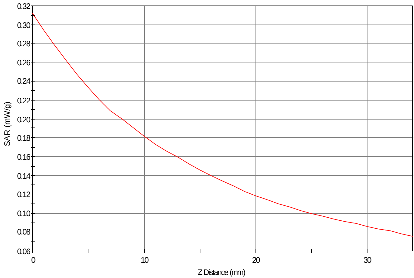
SAR - Z Axis at Hotspot x:65.0 y:21.0
