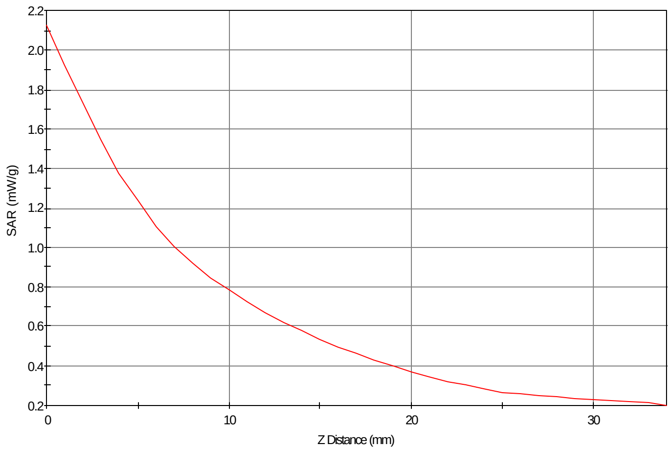
SAR - Z Axis at Hotspot x:68.0 y:24.0
