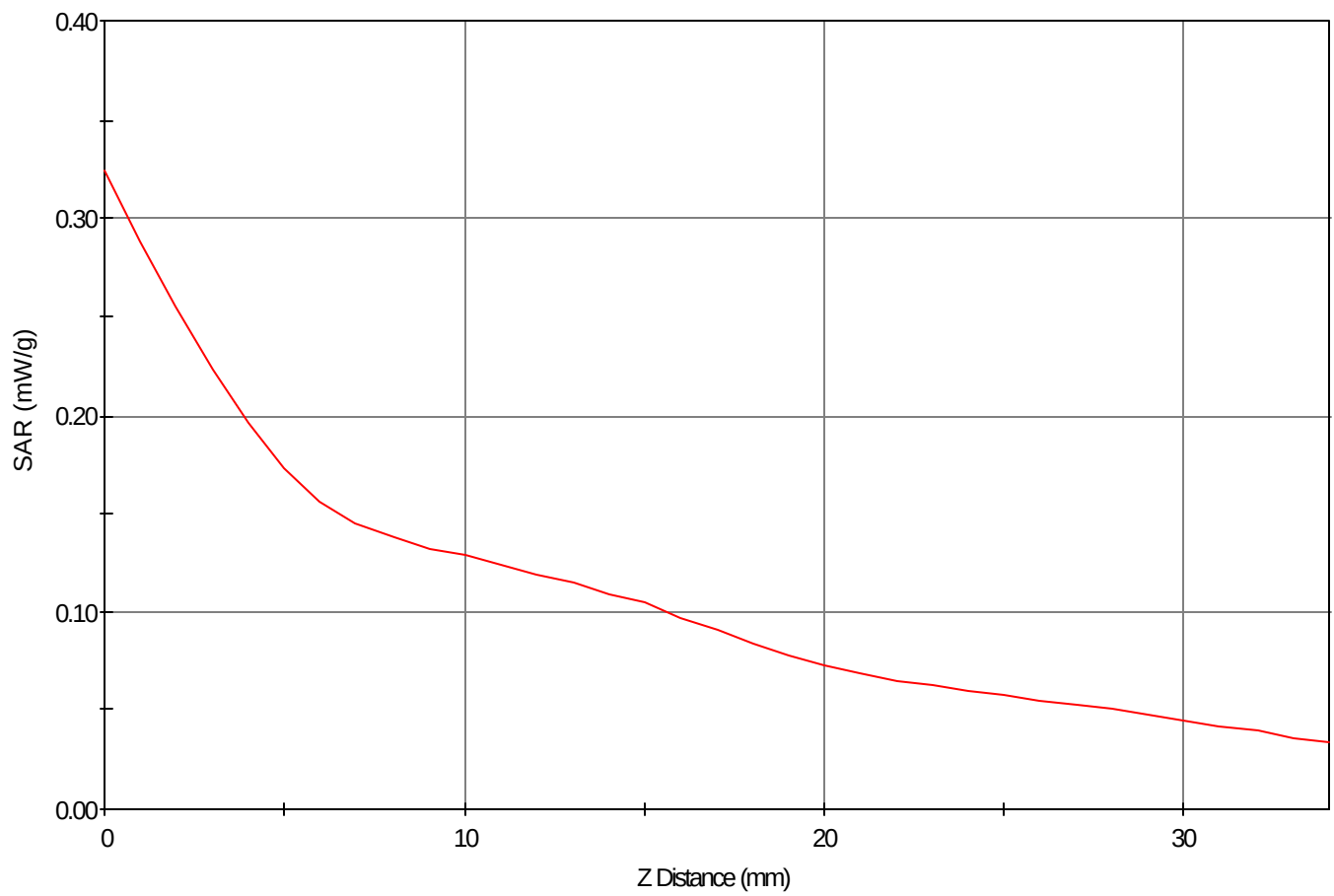
SAR - Z Axis at Hotspot x:62.0 y:26.0
