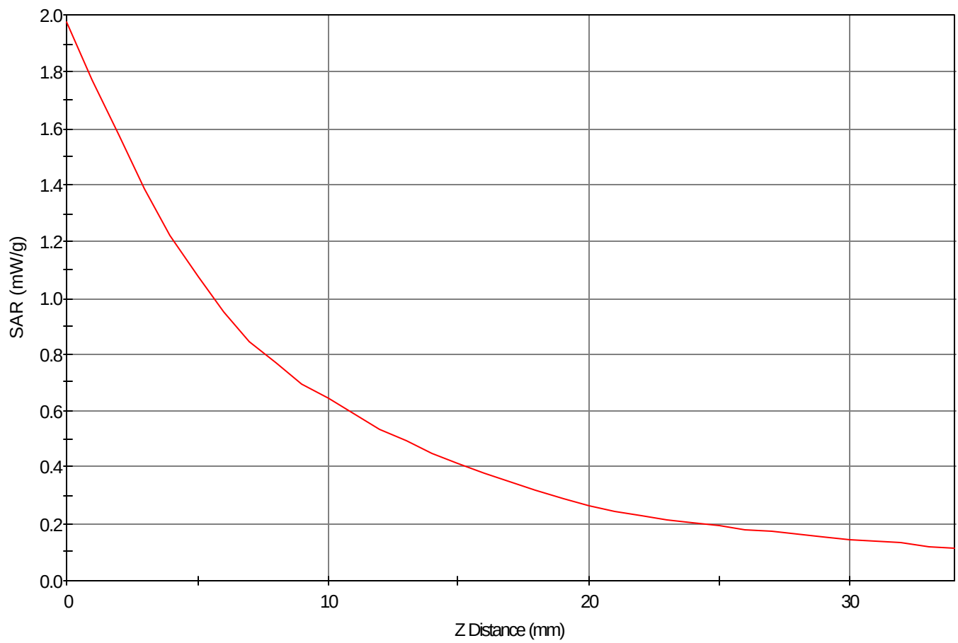
SAR - Z Axis at Hotspot x:65.0 y:14.0
