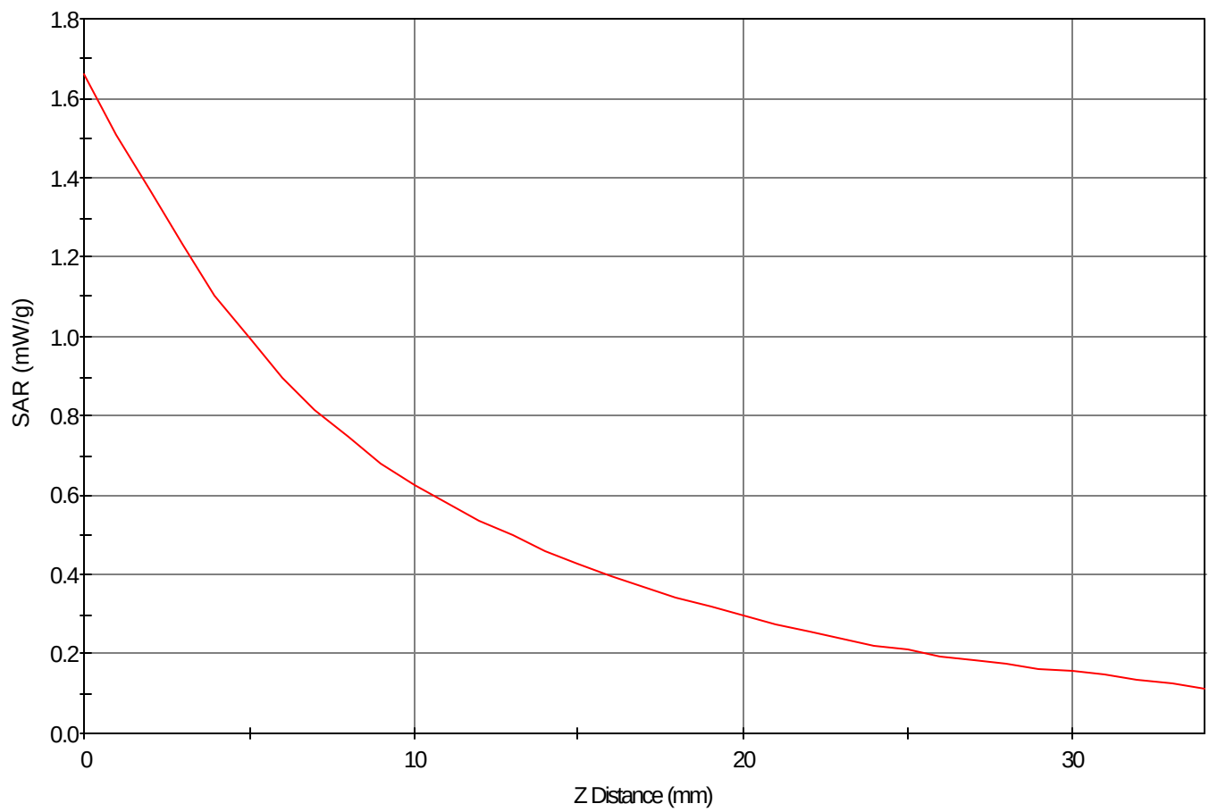
SAR - Z Axis at Hotspot x:73.0 y:25.0
