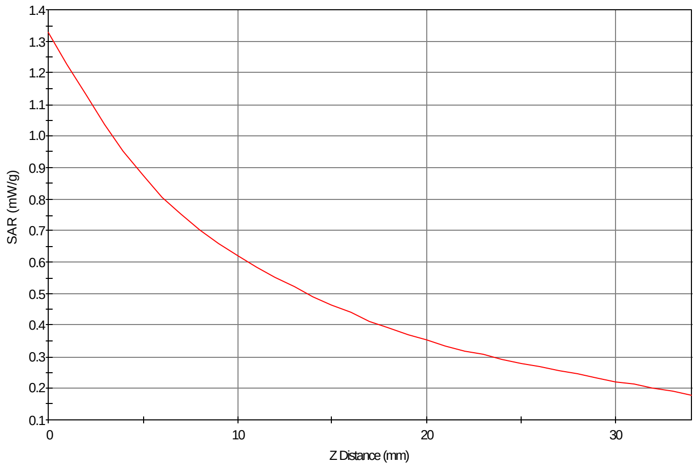
SAR - Z Axis at Hotspot x:68.0 y:18.0
