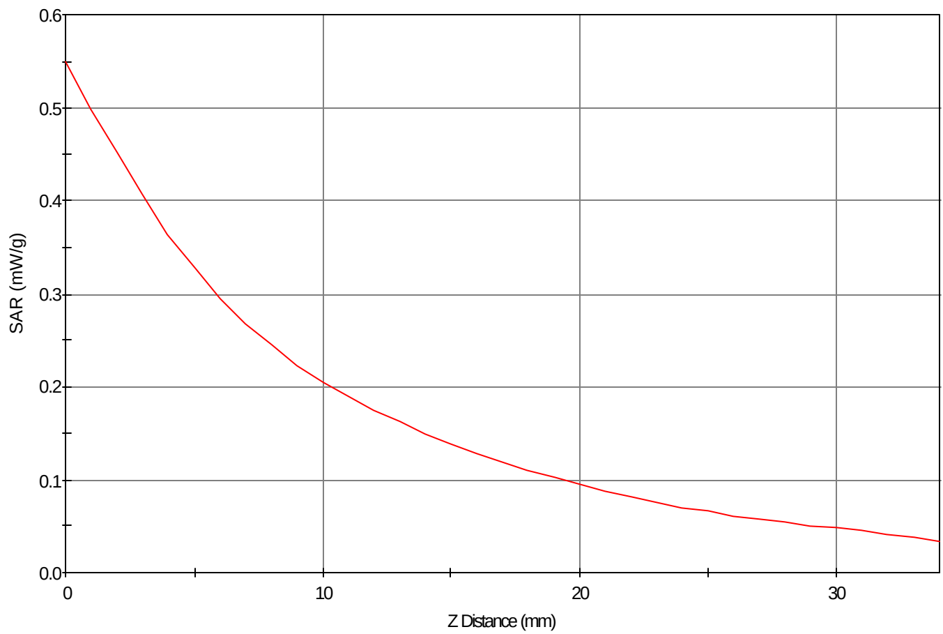
SAR - Z Axis at Hotspot x:63.0 y:17.0
