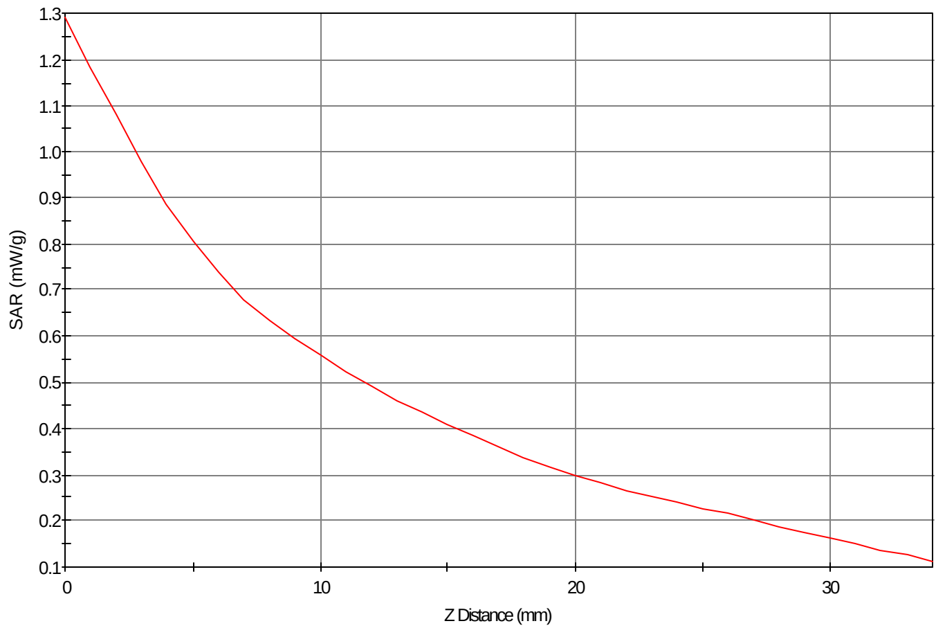
SAR - Z Axis at Hotspot x:3.0 y:-6.0
