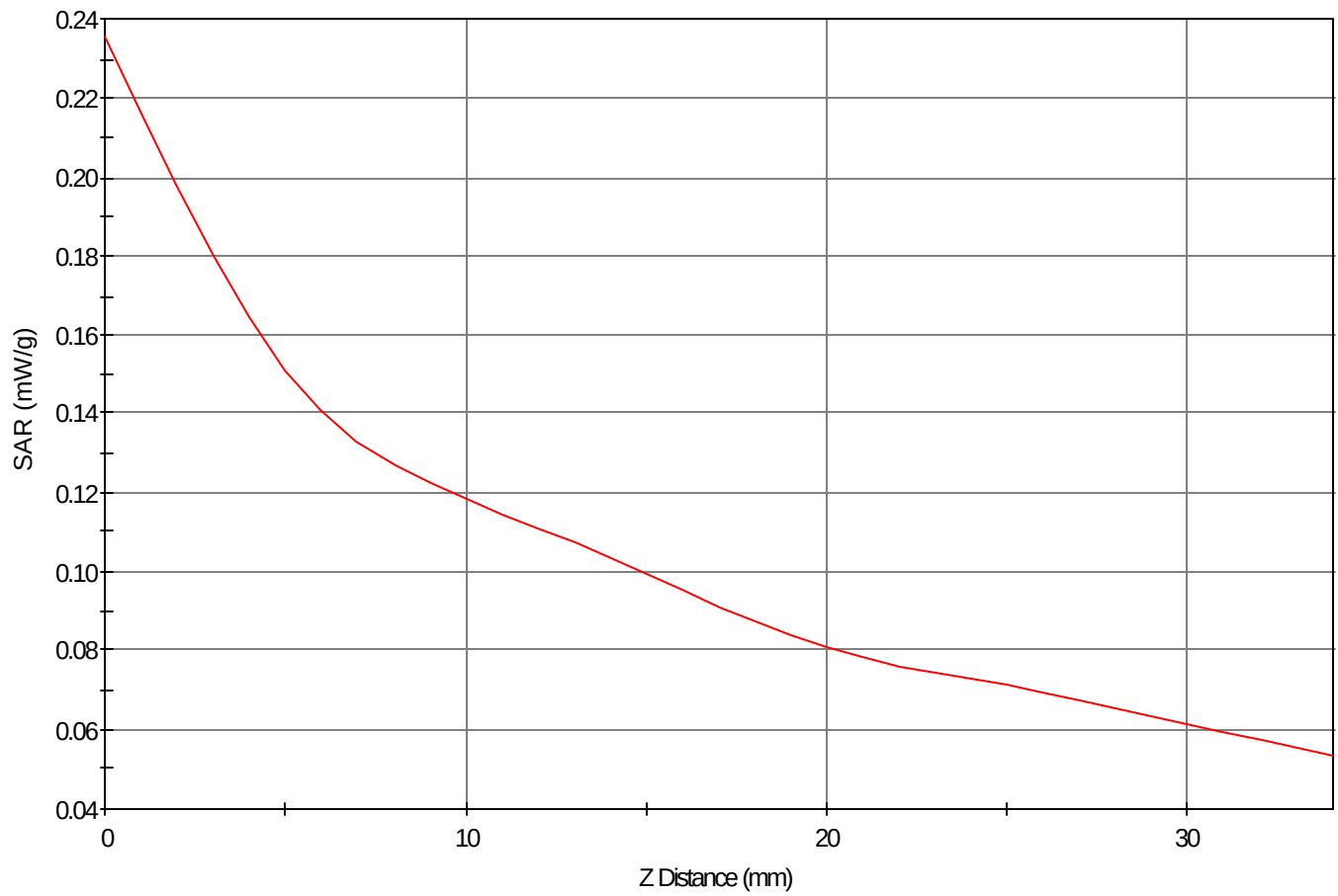
SAR - Z Axis at Hotspot x:60.0 y:28.0
