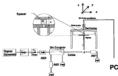
Figure 7.1 Dipole Validation Test Setup
