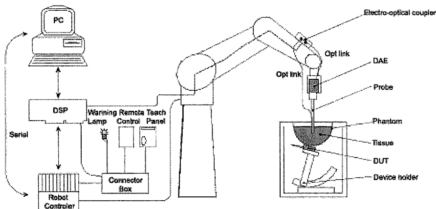
Figure 3.1 SAR Measurement System Setup
