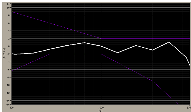
Figure 7-1 Axial Frequency Response
