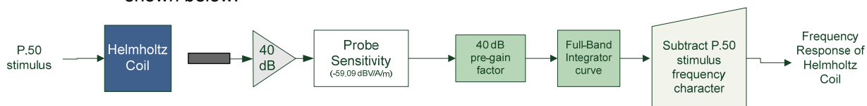
Figure 5-4 Frequency Response Validation
