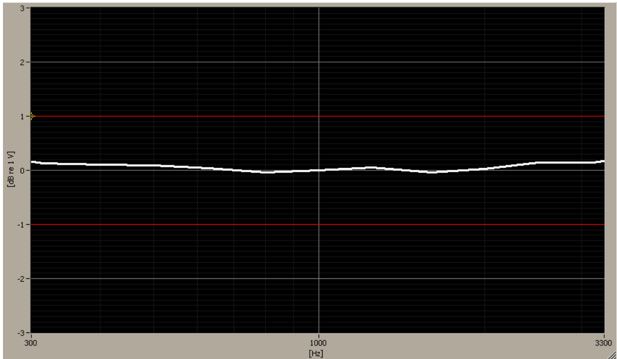
Figure 7-2 Helmholtz Coil Validation for Frequency Response
