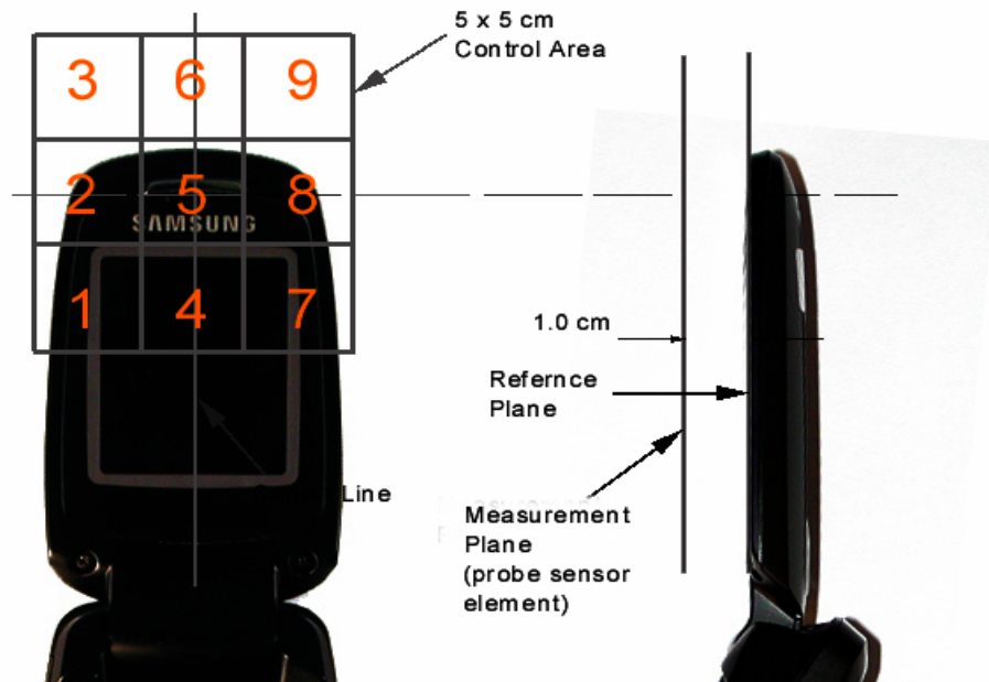
Figure 31 5x5 Scan grid above WD
