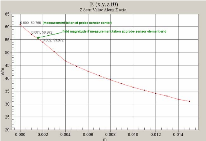
Figure 5 Z-axis scan at maximum point above wireless device for E-field
