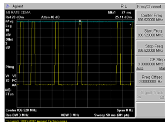
Figure 25 Zero-Span Plots
