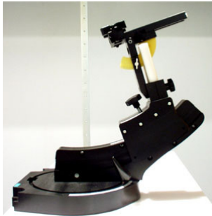
Figure 3.8 Device Holder
