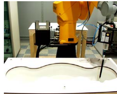
Figure 3.7 Simulated Tissue
