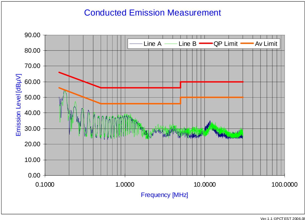
Plot 7-1. Line-Conducted Test Plot
