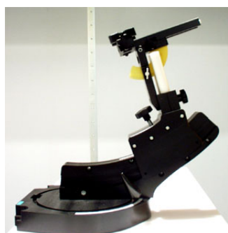
Figure 3.8 Device Holder
