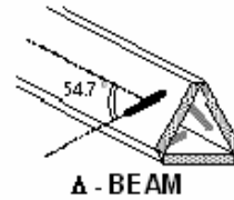
Figure 3.3 Triangular Probe Configuration
