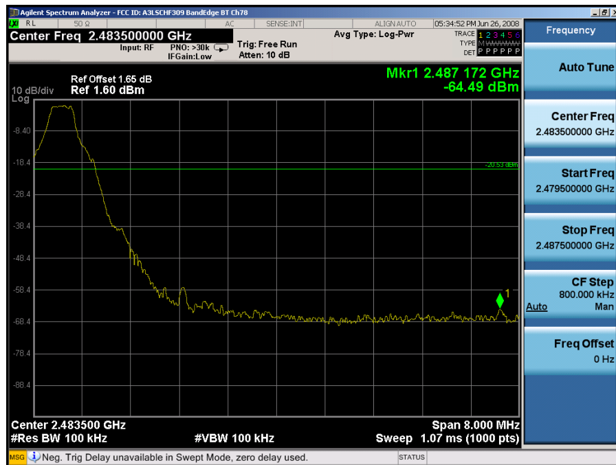
Plot 6-5. Band Edge Plot (Bluetooth – Ch. 78)
