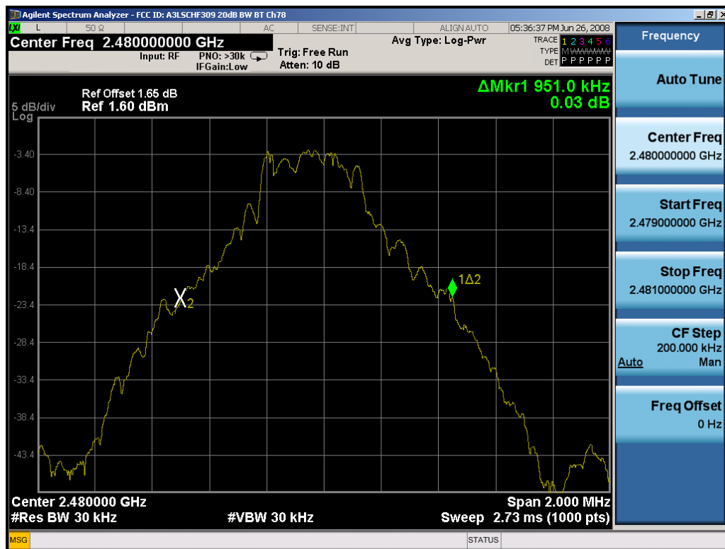
Plot 6-3. 20dB Bandwidth Plot (Bluetooth – Ch. 78)
