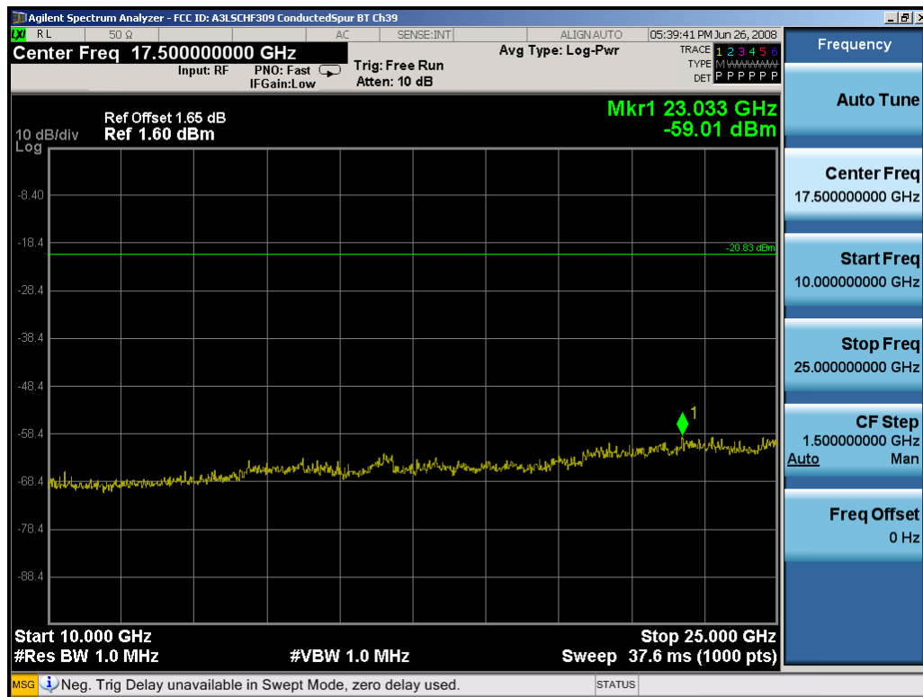
Plot 6-13. Conducted Spurious Plot (Bluetooth – Ch. 39)
