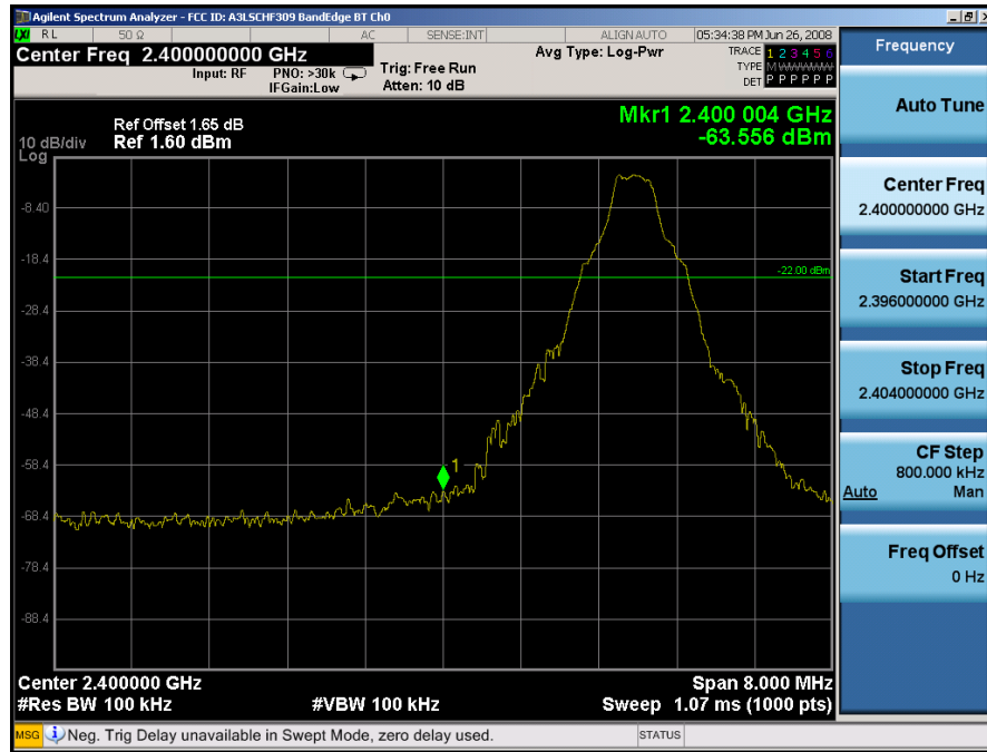
Plot 6-4. Band Edge Plot (Bluetooth – Ch. 0)
