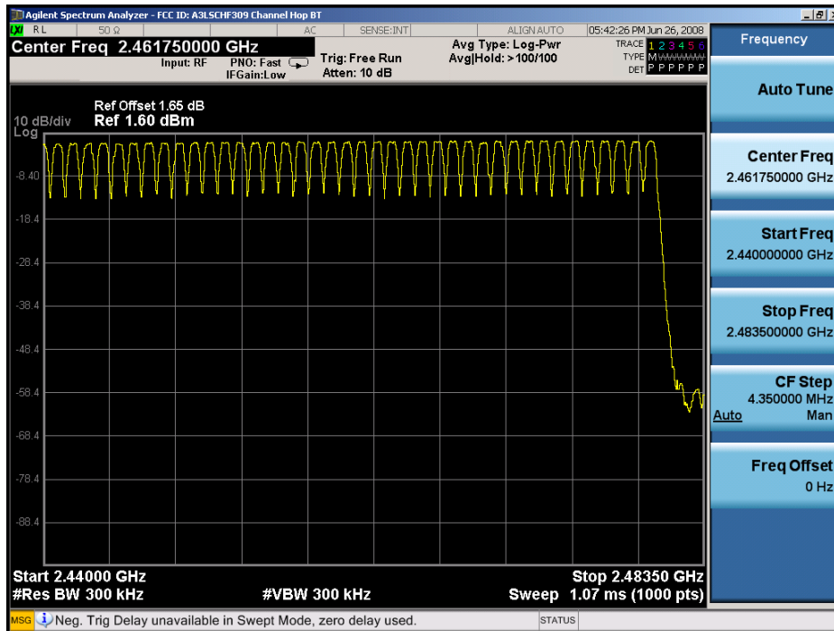
Plot 6-9. High End Spectrum Channel Hopping Plot (Bluetooth)
