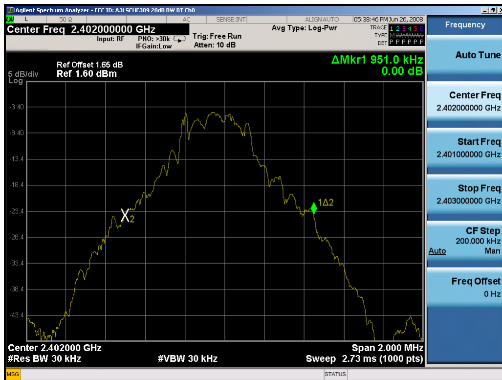
Plot 6-1. 20dB Bandwidth Plot (Bluetooth – Ch. 0)
