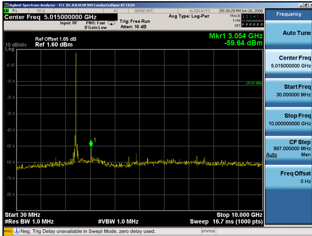
Plot 6-12. Conducted Spurious Plot (Bluetooth – Ch. 39)
