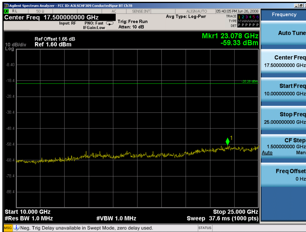
Plot 6-15. Conducted Spurious Plot (Bluetooth – Ch. 78)
