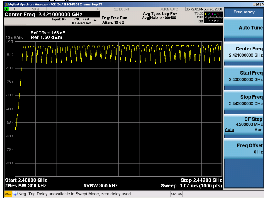
Plot 6-8. Low End Spectrum Channel Hopping Plot (Bluetooth)
