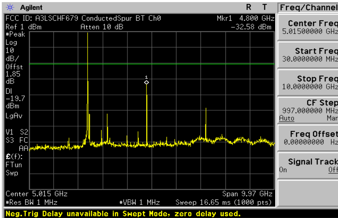
Plot 6-10. Conducted Spurious Plot (Bluetooth – Ch. 0)
