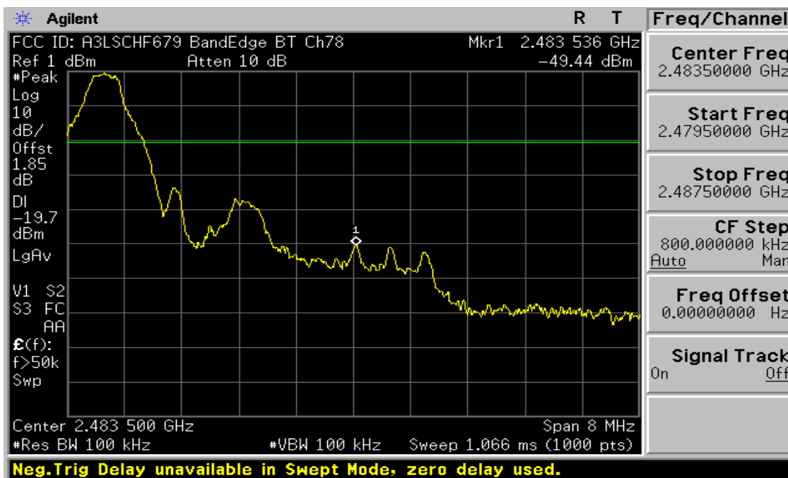
Plot 6-5. Band Edge Plot (Bluetooth – Ch. 78)
