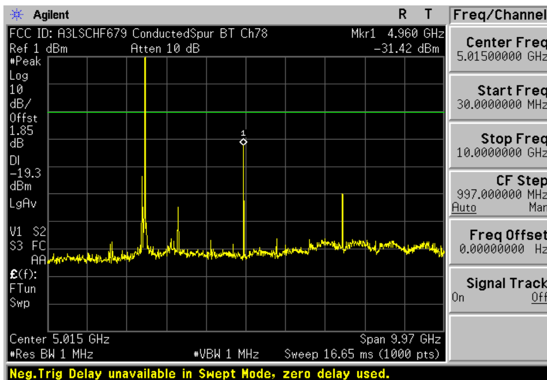
Plot 6-14. Conducted Spurious Plot (Bluetooth – Ch. 78)
