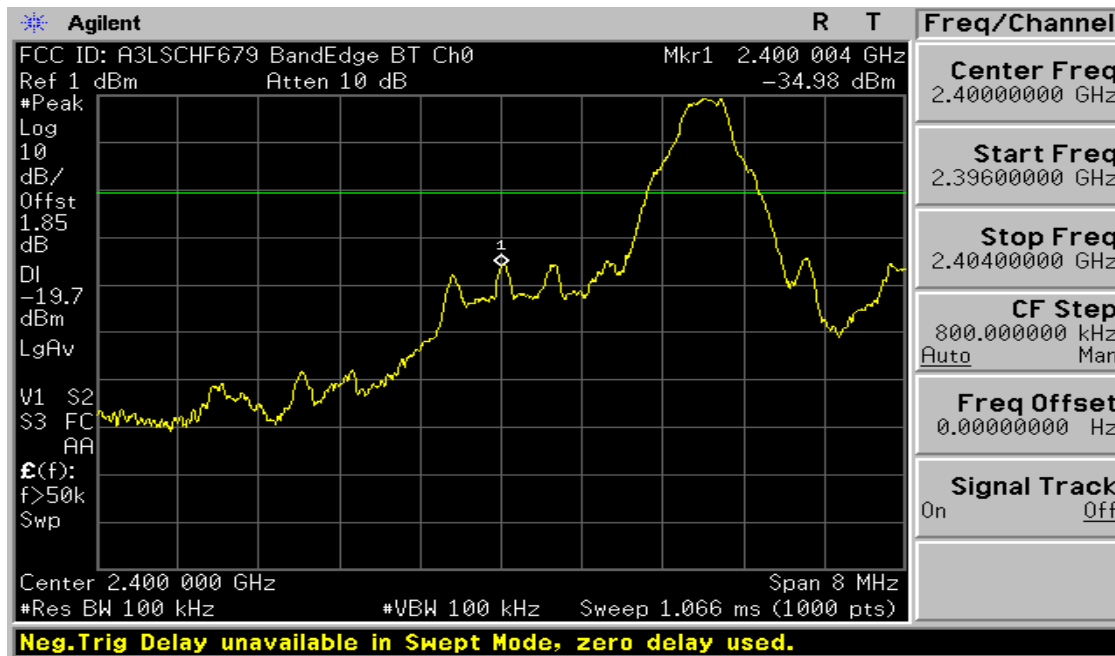
Plot 6-4. Band Edge Plot (Bluetooth – Ch. 0)
