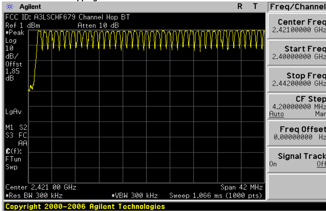
Plot 6-8. Low End Spectrum Channel Hopping Plot (Bluetooth)
