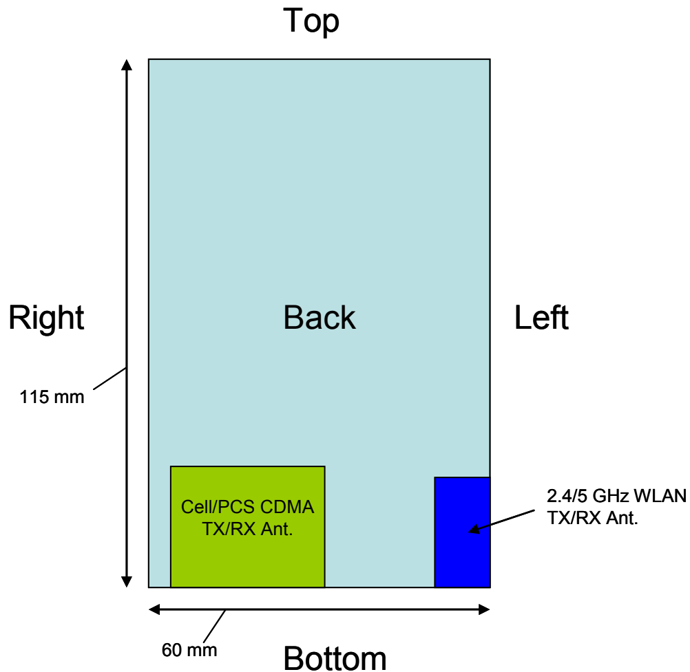
Figure 13-1 Identification of Sides for SAR Testing
