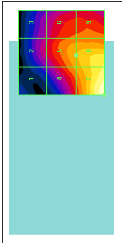
Figure 10-2 Sample H-field Scan Overlay
