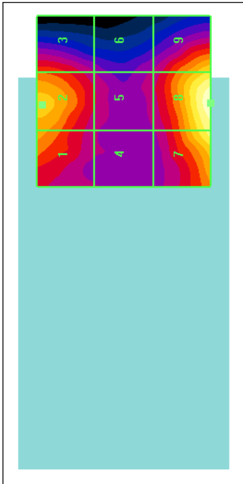
Figure 10-1 Sample E-field Scan Overlay
