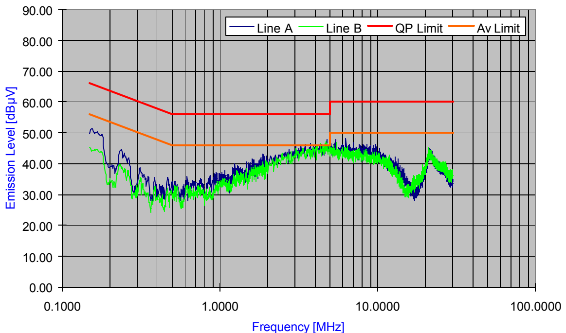
Plot 6-53. Line Conducted Plot with 802.11b
