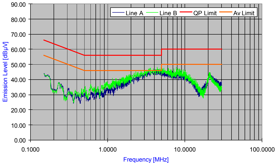
Plot 6-54. Line Conducted Plot with 802.11g
