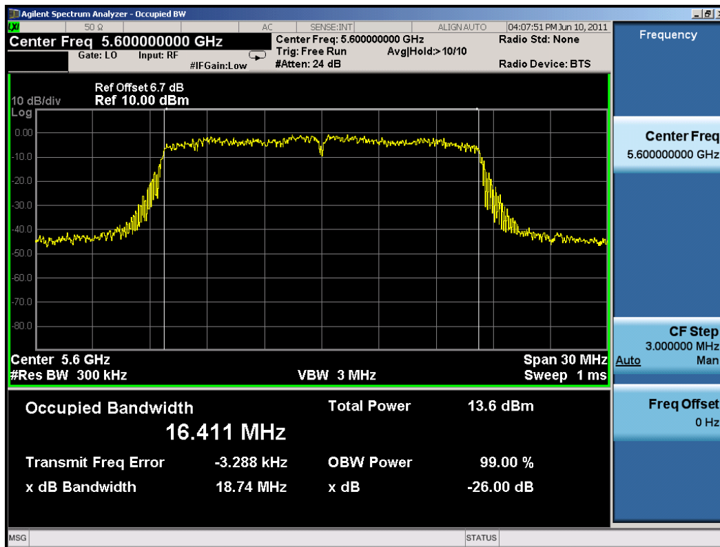
Plot 6-14. 26dB Bandwidth Plot (802.11a (UNII Band 3) – Ch. 120)
