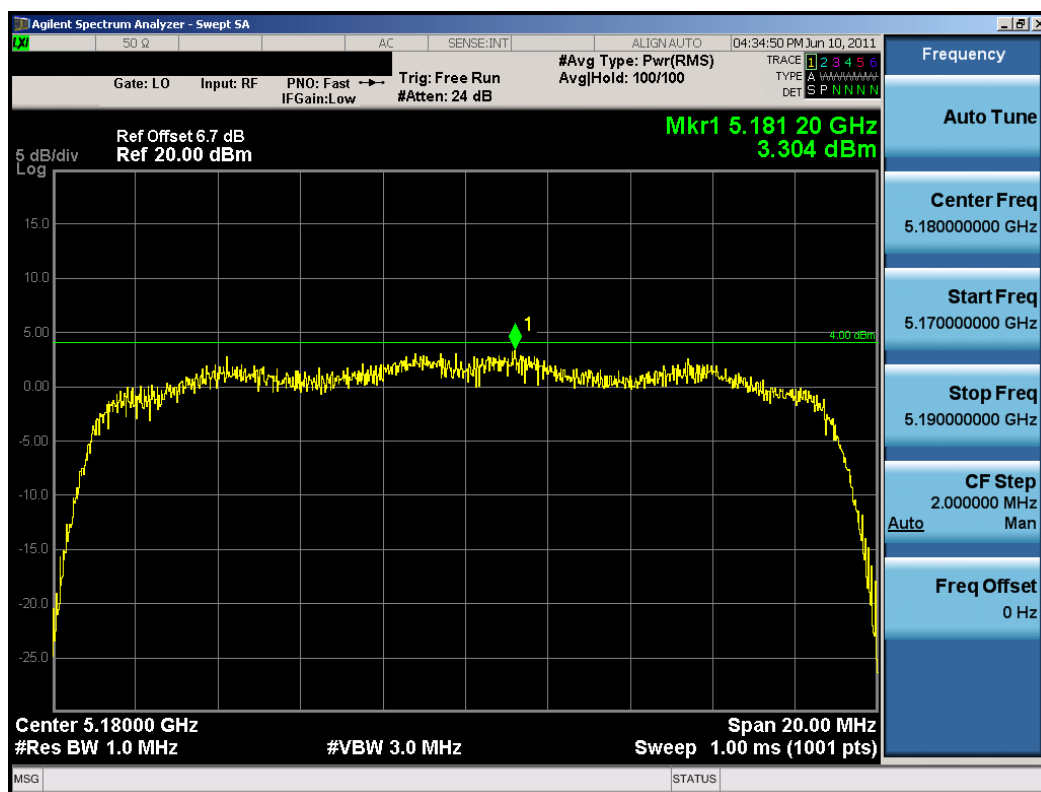
Plot 6-22. Peak Power Spectral Density Plot (802.11n (UNII Band 1) – Ch. 36)
