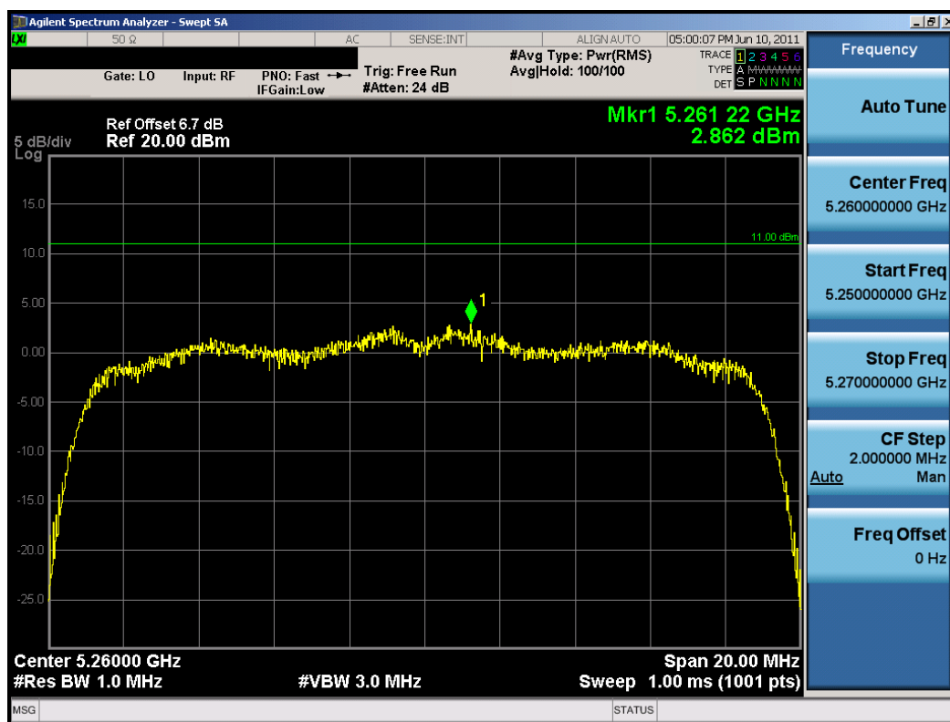
Plot 6-28. Peak Power Spectral Density Plot (802.11n (UNII Band 2) – Ch. 52)
