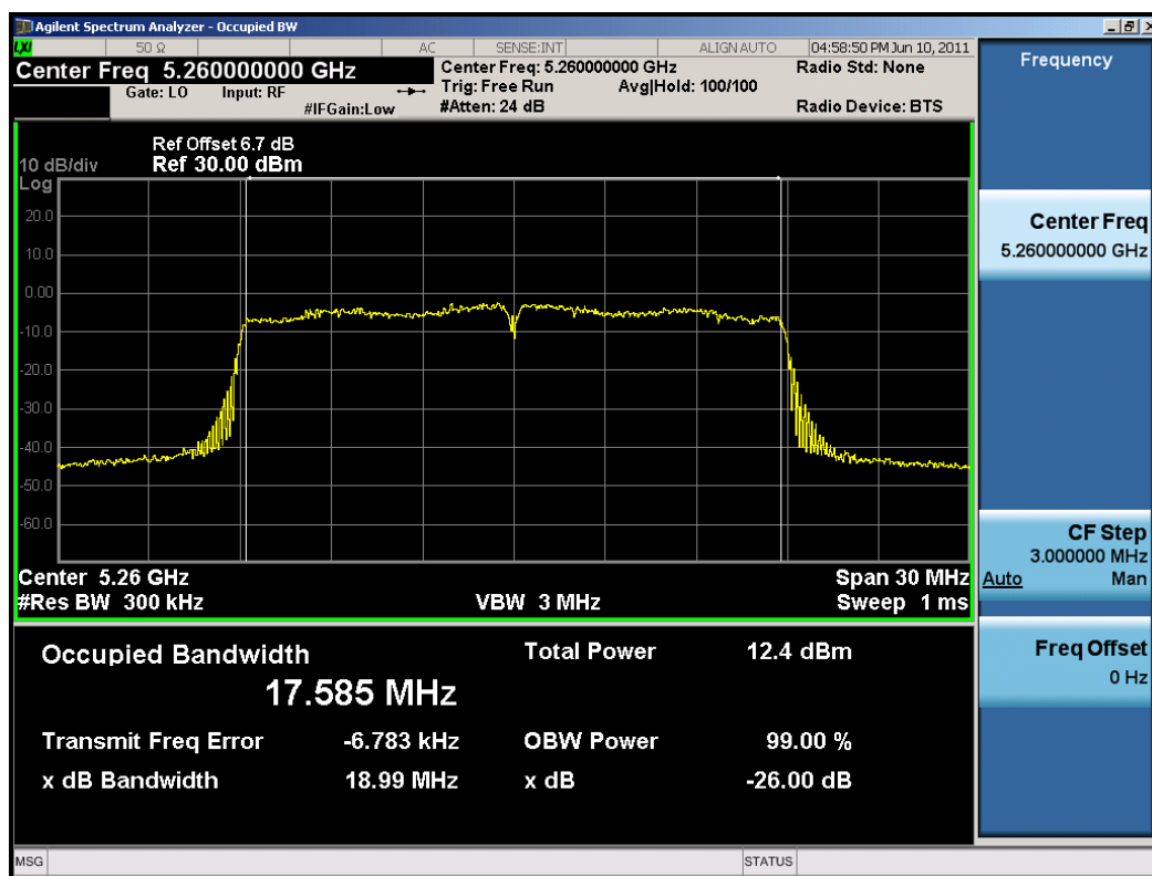
Plot 6-10. 26dB Bandwidth Plot (802.11n (UNII Band 2) – Ch. 52)
