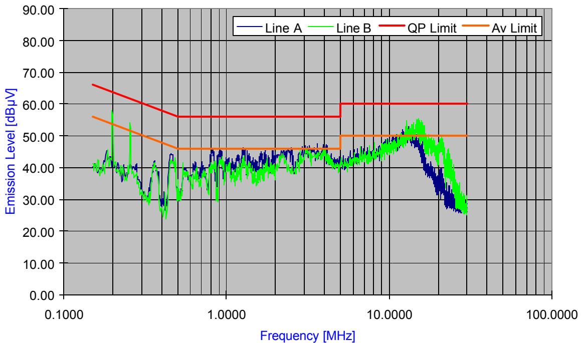
Plot 6-60. Line Conducted Plot with 802.11n (UNII Band 3)
