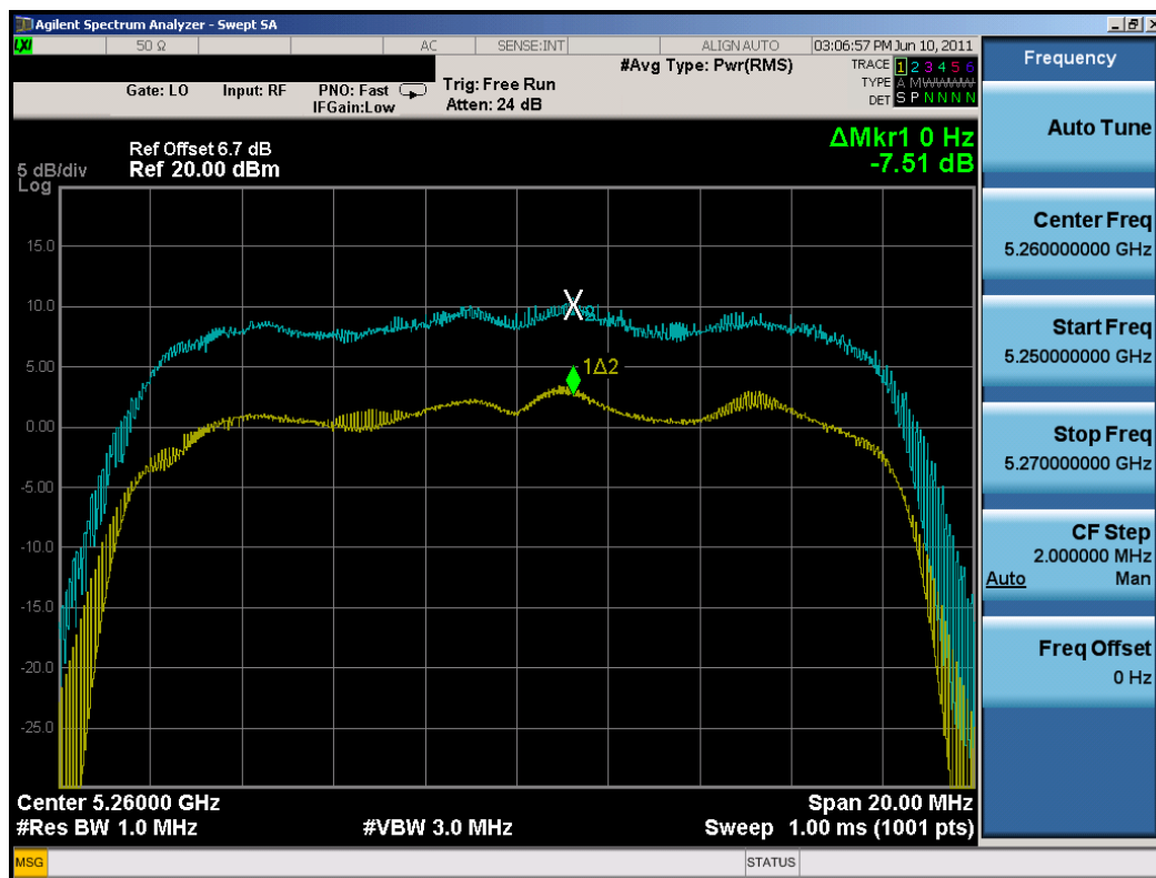
Plot 6-43. Peak Excursion Ratio Plot (802.11a (UNII Band 2) – Ch. 52)
