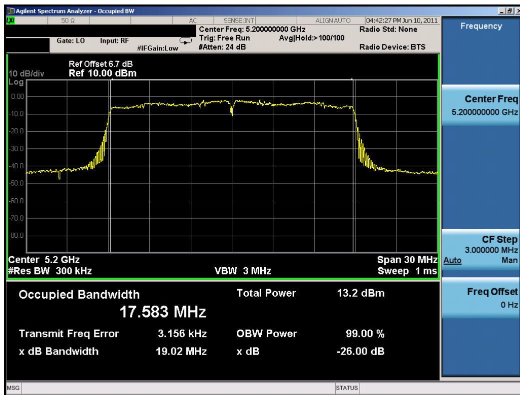
Plot 6-5. 26dB Bandwidth Plot (802.11n (UNII Band 1) – Ch. 40)
