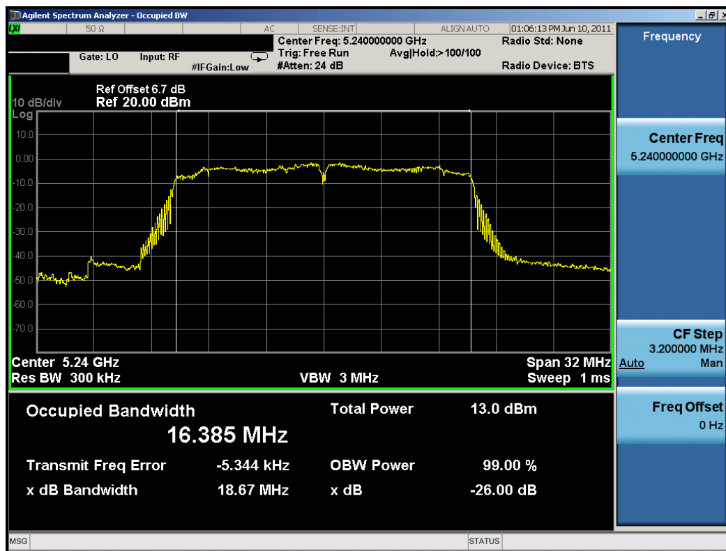
Plot 6-3. 26dB Bandwidth Plot (802.11a (UNII Band 1) – Ch. 48)
