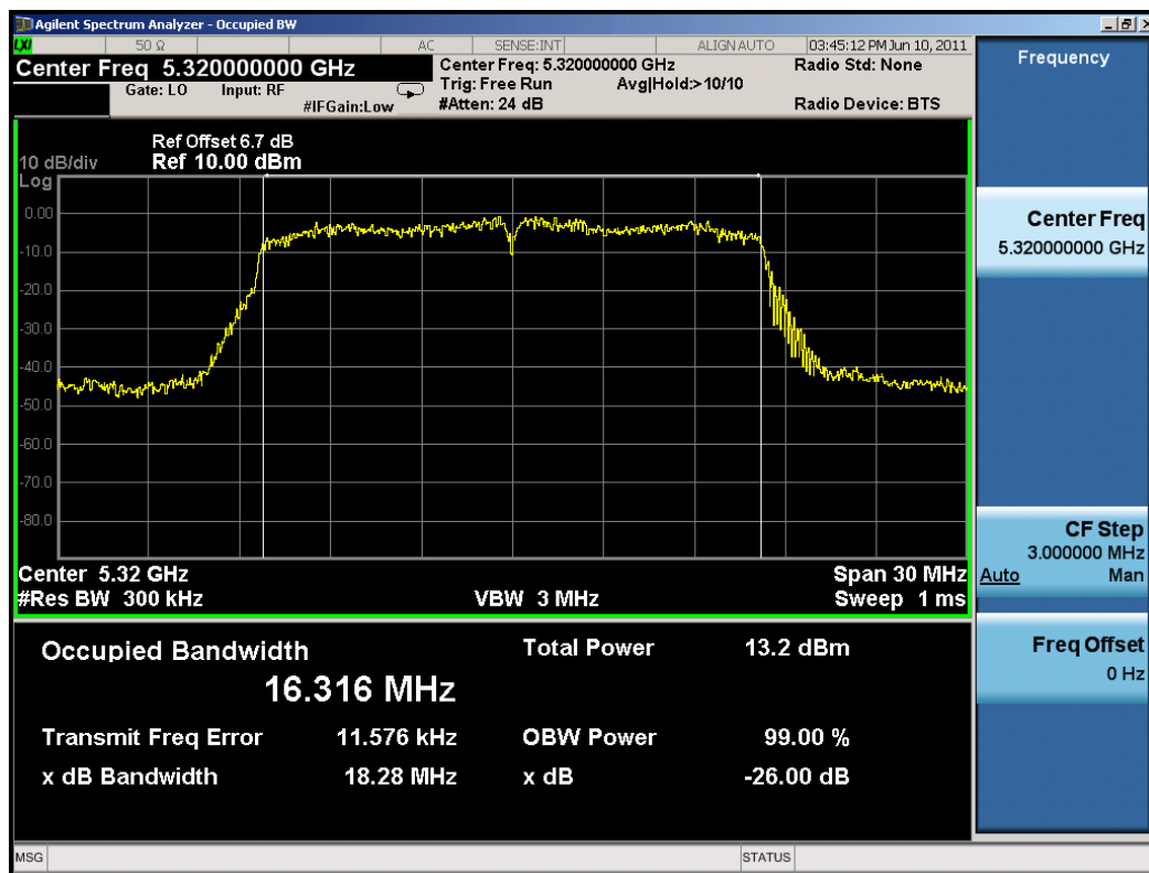
Plot 6-9. 26dB Bandwidth Plot (802.11a (UNII Band 2) – Ch. 64)
