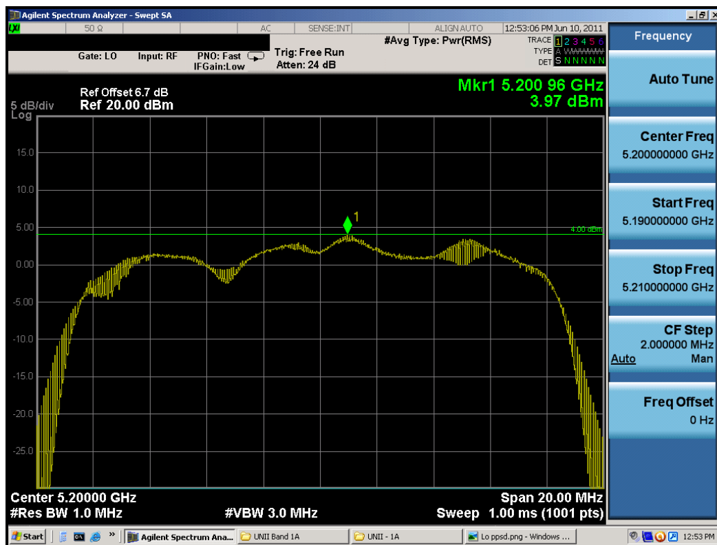
Plot 6-20. Peak Power Spectral Density Plot (802.11a (UNII Band 1) – Ch. 40)
