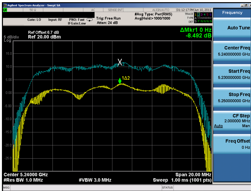
Plot 6-39. Peak Excursion Ratio Plot (802.11a (UNII Band 1) – Ch. 48)
