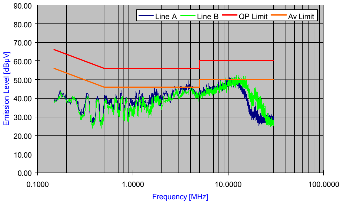
Plot 6-58. Line Conducted Plot with 802.11n (UNII Band 1)
