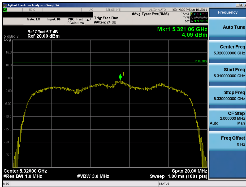
Plot 6-27. Peak Power Spectral Density Plot (802.11a (UNII Band 2) – Ch. 64)
