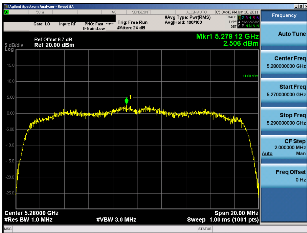
Plot 6-29. Peak Power Spectral Density Plot (802.11n (UNII Band 2) – Ch. 56)
