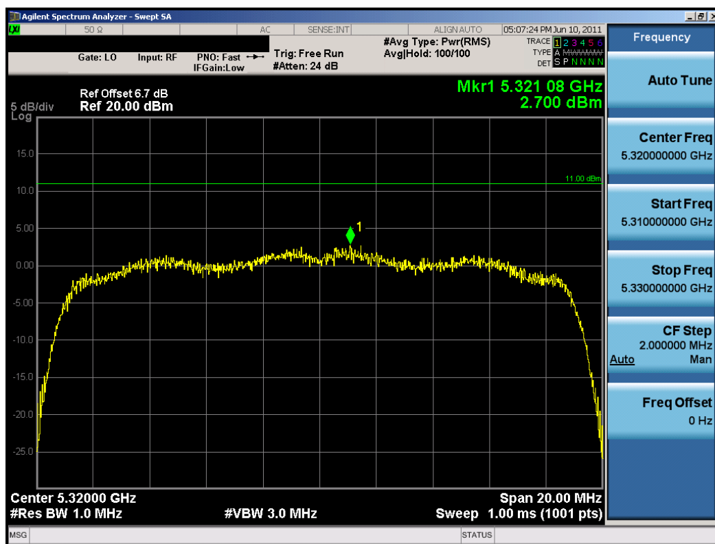
Plot 6-30. Peak Power Spectral Density Plot (802.11n (UNII Band 2) – Ch. 64)
