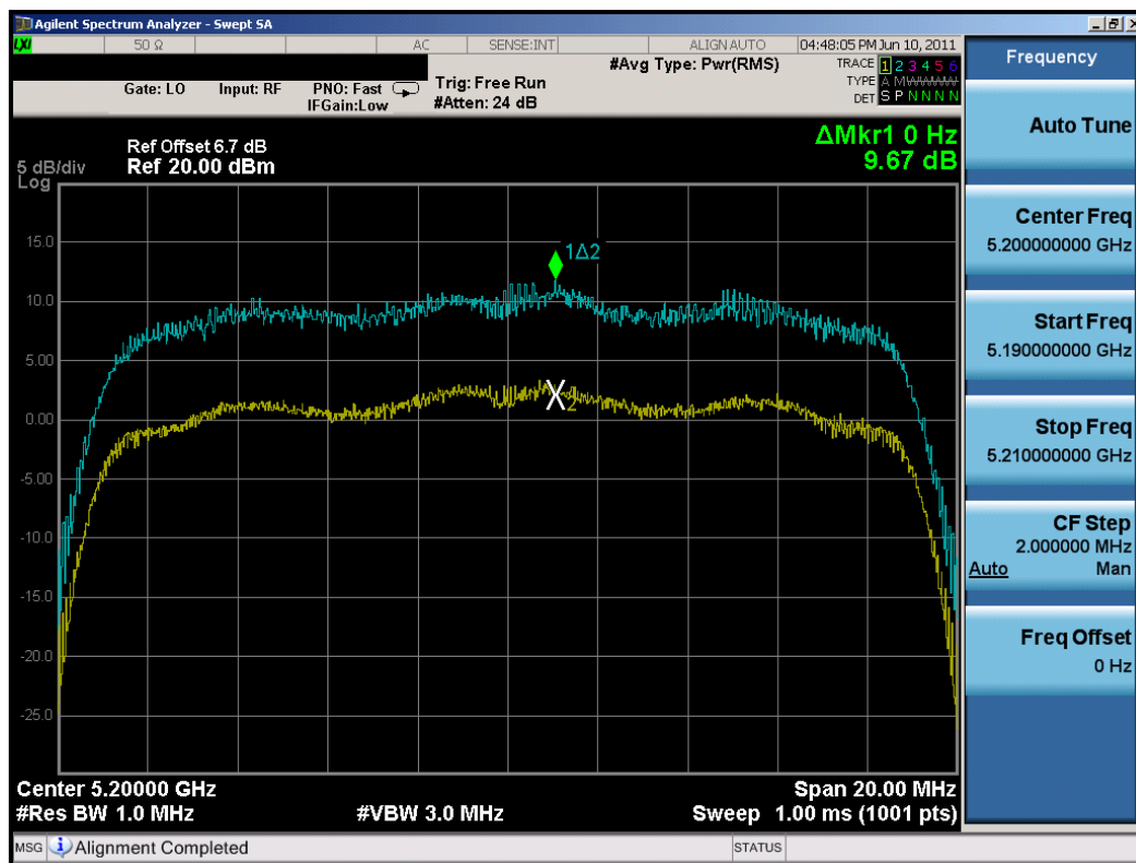
Plot 6-41. Peak Excursion Ratio Plot (802.11n (UNII Band 1) – Ch. 40)
