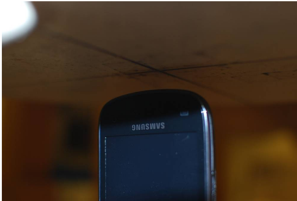
SAR Test Setup Photo 9 – Body Bottom at 1.0 cm with Extended Battery
