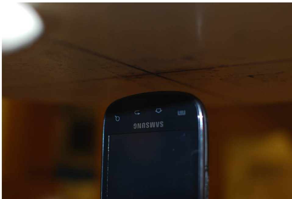
SAR Test Setup Photo 8 – Body Bottom at 1.0 cm with Standard Battery
