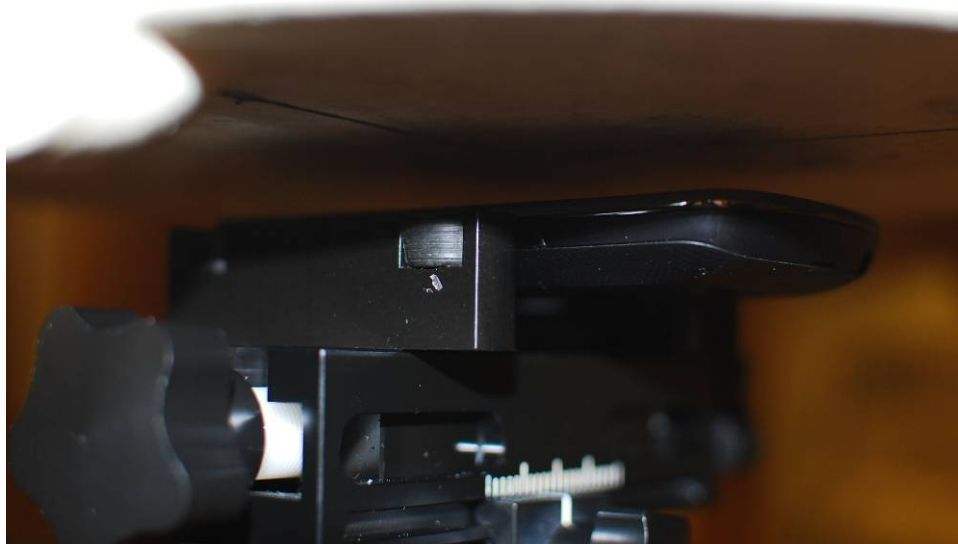
SAR Test Setup Photo 7 – Body Front at 1.0 cm with Standard Battery
