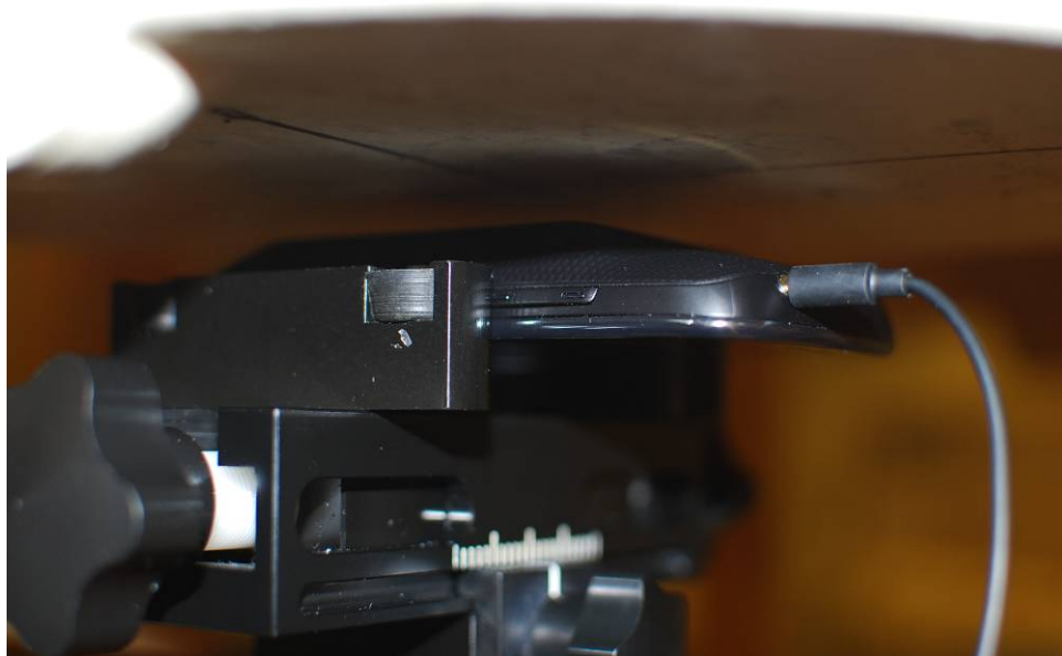
SAR Test Setup Photo 13 – Body-Worn Back at 1.0 cm with Extended Battery
