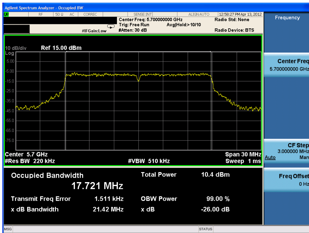
Plot 6-22. 26dB Bandwidth Plot (802.11a/n UNII MEASUREMENT REPORT (CERTIFICATION)
