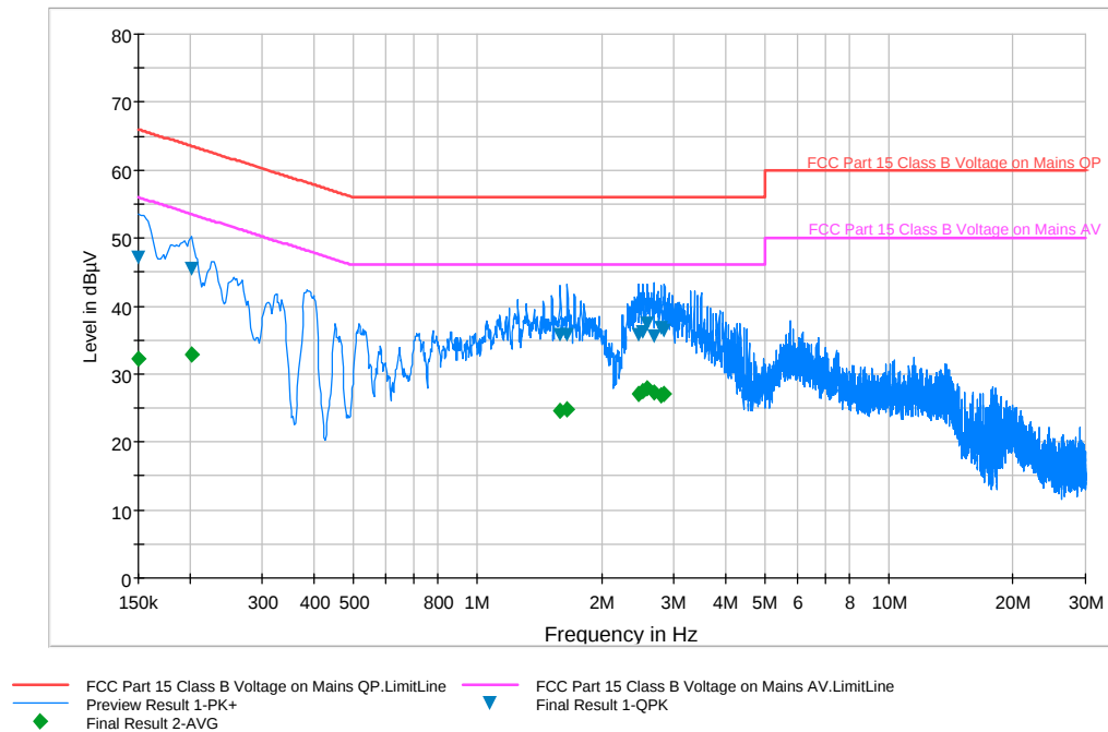
Plot 6-24. Line-Conducted Test Plot (L1)
