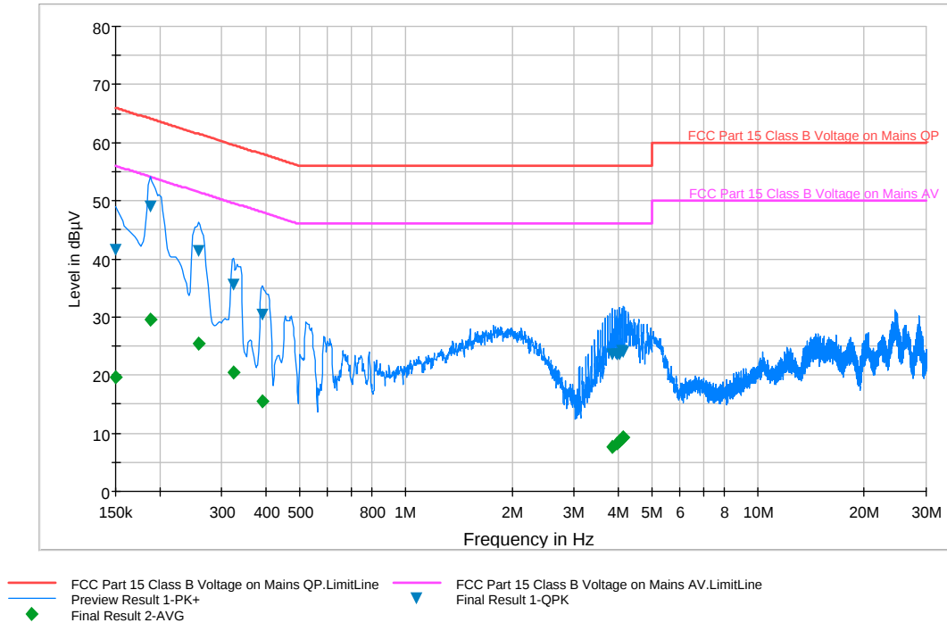
Plot 7-2. Line Conducted Plot (LN)
