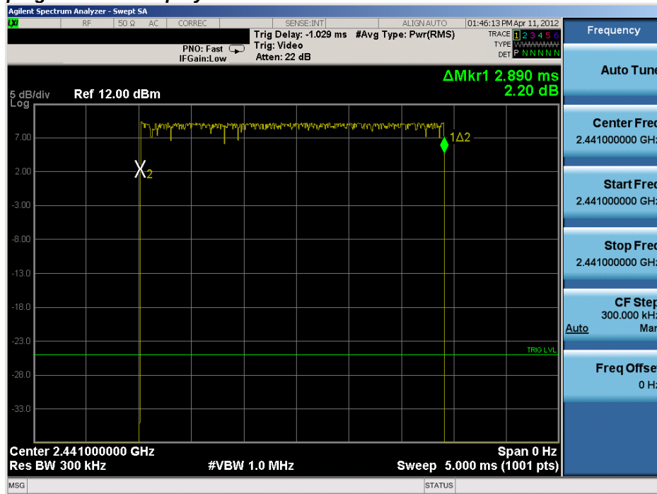
Plot 6-1. Time of Occupancy Plot (Bluetooth)
