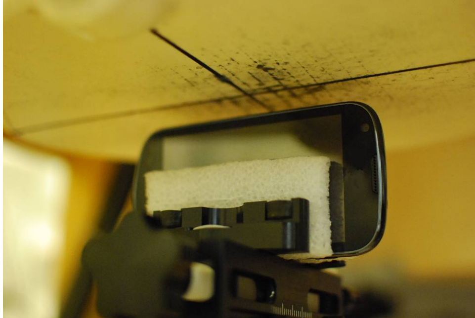
SAR Test Setup Photo 7: Left Edge at 1.0 cm
