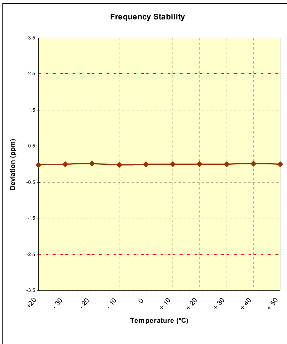
Figure 6-1. Frequency Stability Graph (AWS CDMA Mode – Ch. 450)
