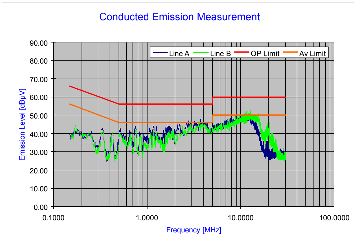
Plot 6-56. Line Conducted Plot with 802.11n (2.4GHz)
