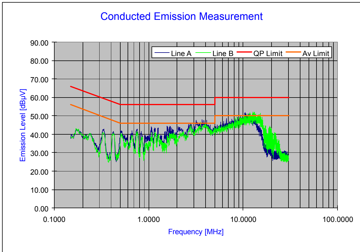
Plot 6-54. Line Conducted Plot with 802.11g
