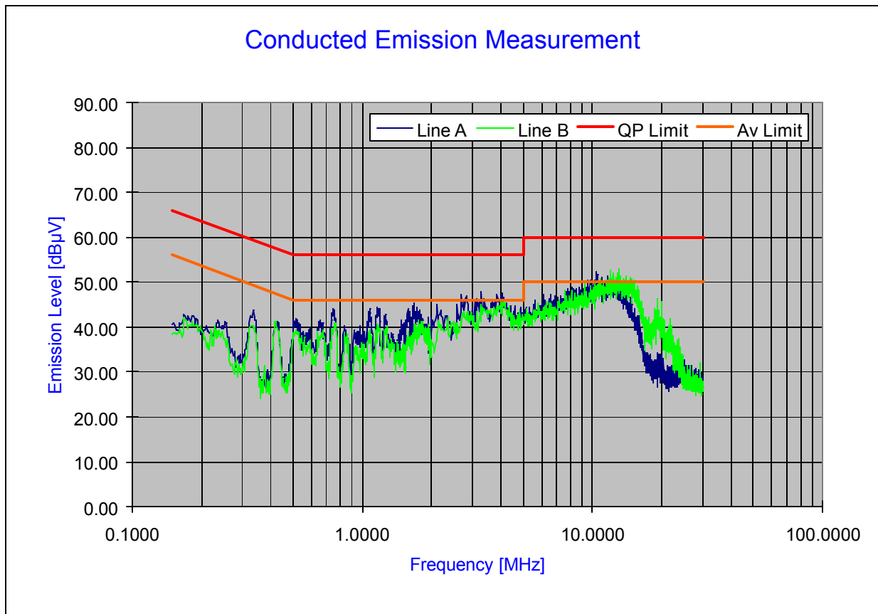
Plot 6-53. Line Conducted Plot with 802.11b
